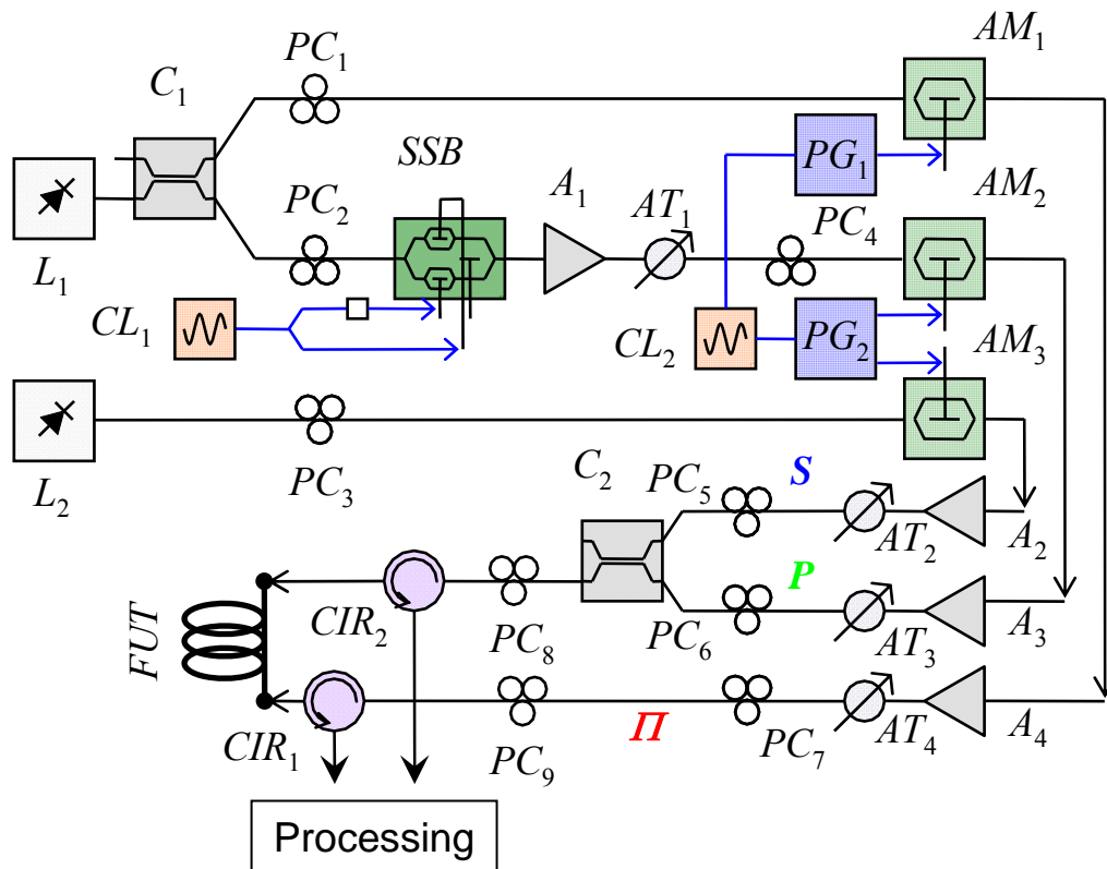
Fig. 13: Experimental setup.
