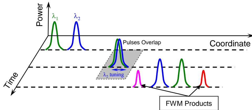
Fig. 4: Schematic representation of Gordon's method.
