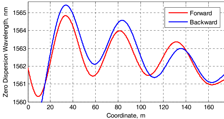
Fig. 39: Comparison between ZDW measurements obtained from traces scanned in both directions.
