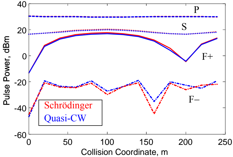
Fig. 23: Powers of the probe P, second pulse S, and FPM sidebands F_{\pm} at the end of the fiber obtained using the integration of the time-dependent Schrödinger and quasi-CW equations.
