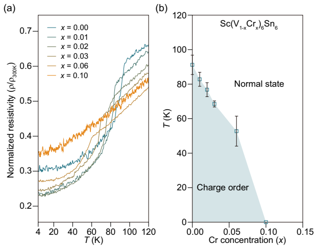
Fig. 5 Phase diagram of charge order in \text{Sc}(\text{V}_{1-x}\text{Cr}_x)_6\text{Sn}_6 series. a Evolution of the normalized resistivity T/\rho_{300\text{K}} as a function of Cr-doping in x = 0, 0.01, 0.02, 0.03, and 0.06 samples. b Doping-temperature phase diagram of the charge order in \text{ScV}_6\text{Sn}_6 , error bars indicate the range of resistance change during transitions.
