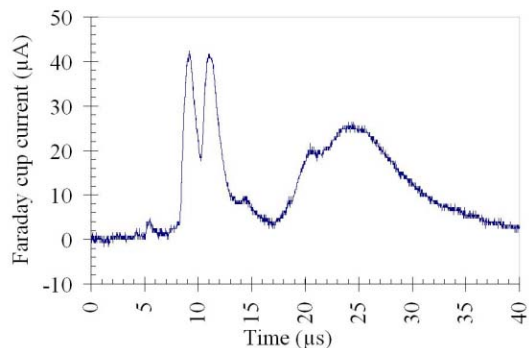
Figure 5: Faraday cup signal, pulsed arc.
