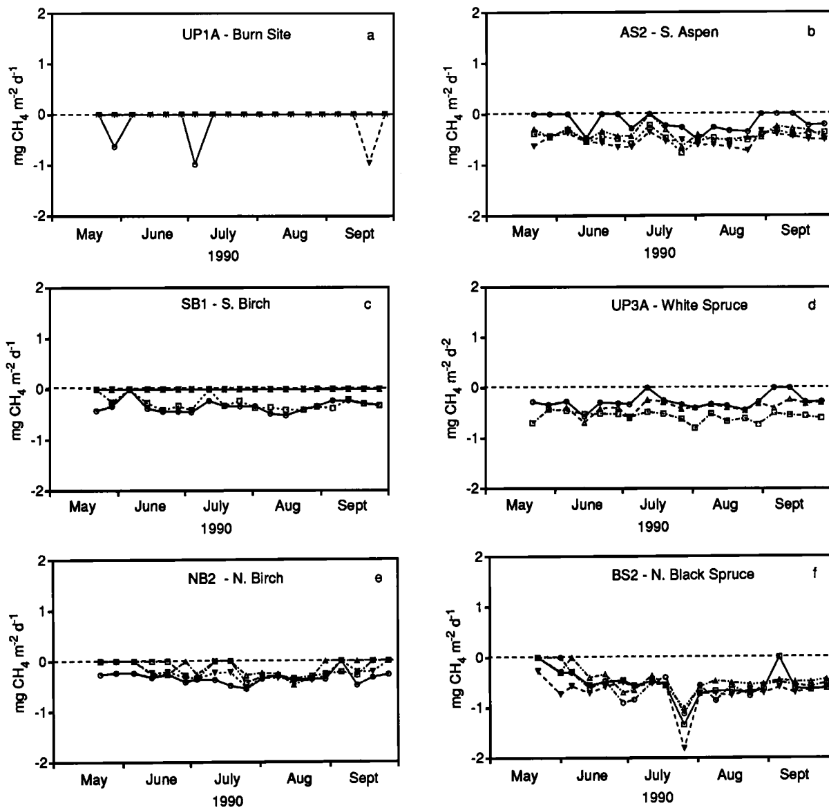
Fig. 3. Methane fluxes ( \text{mg m}^{-2} \text{d}^{-1} ) from Bonanza Creek Experimental Forest upland sites, May 22 - September 27, 1990. Data from the N-fertilized plots at sites AS2, SB1, NB2, and BS2 are plotted as triangles. (a) UP1A, burn site ( Calamagrostis , triangles; Equisetum , open symbols). (b) AS2, aspen. (c) SB1, birch. (d) UP3A, white spruce. (e) NB2, north birch. (f) BS2, north black spruce.
