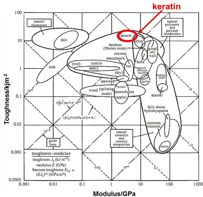
Figure 1.5 A material property chart for natural materials, plotting toughness against Young's modulus [25].
