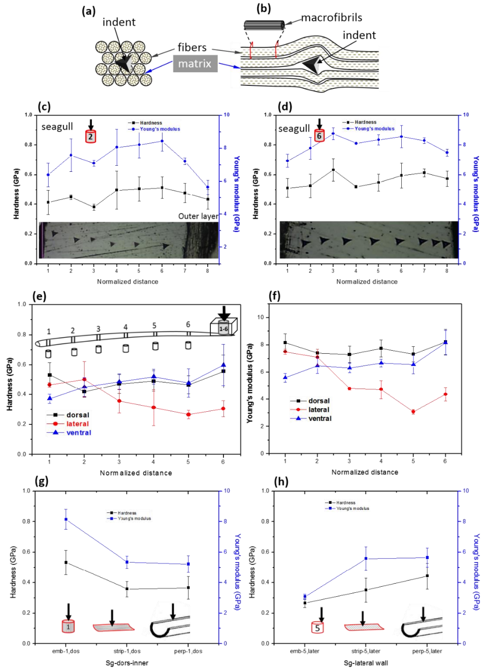
Figure 5.9 Indenting on composite of uniaxial fibers with indenting (a) parallel and (b) perpendicular to the fiber direction. The fibers are composed of macrofibrils in the feather cortex. Nanoindentation results from seagull feather shaft: along dorsal cortex thickness from inner to outside (c) at the calamus and (d) the distal rachis (position #6); (e,f) on dorsal, lateral and ventral regions along the shaft length; (g,h) on dorsal and lateral pieces in different loading directions. Each data point represents an average of five measurements and error bars represent standard deviations.
