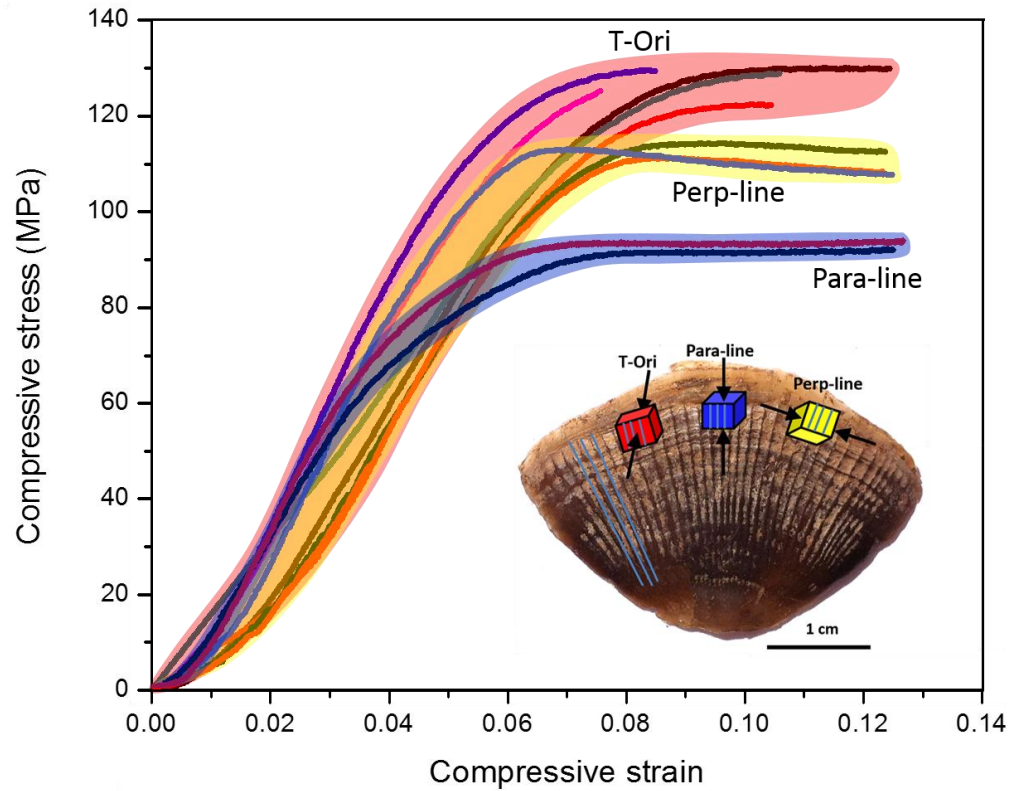
Figure 4.12 Compressive stress-strain curves of Chinese pangolin scales loaded in three orientations.
