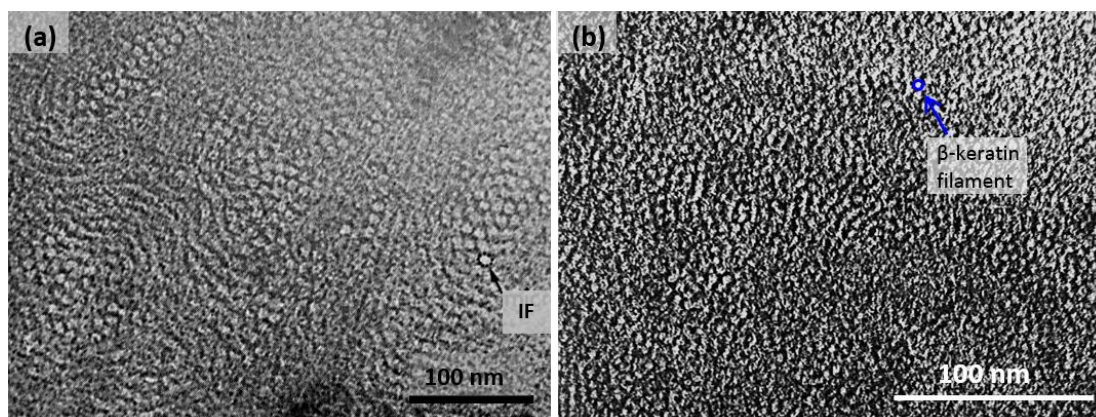
Figure 3.6 Transmission electron micrographs of typical keratinous materials with clear filament-matrix structure: (a) cross section of a human hair ( \alpha -keratin), stained with osmium tetroxide, showing 7 nm diameter intermediate filaments embedded in a darker matrix; (b) cross section of a seagull feather rachis ( \beta -keratin), stained with potassium permanganate, showing the 3.5 nm diameter \beta -keratin filaments differentiated by the densely stained matrix [48].
