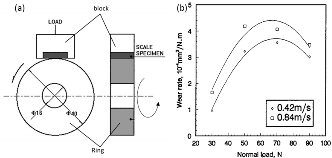
Figure 3.33 . (a) Schematic diagram of the block-on-ring wear test used to determine for wear rate (in volume per unit energy) of pangolin scales; (b) wear rate as a function of normal load for two sliding velocities: 0.42 and 0.84 m/s; as wear rate increases with velocity [249].
