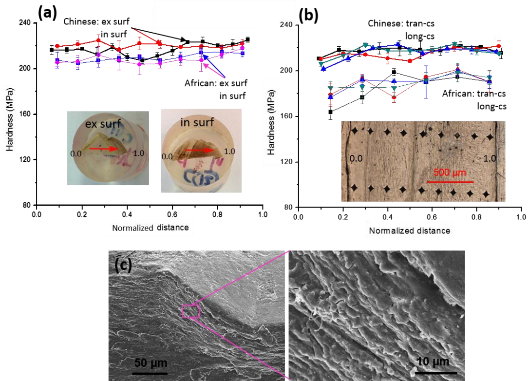
Figure 4.10 Microhardness results of the scales: (a) hardness values of African tree and Chinese pangolins scale along on external surface (ex surf) and internal surface (in surf) along growth line direction (red arrows, from scale base to tip); (b) hardness values of African tree and Chinese pangolin scales indenting on transverse (tran-cs) and longitudinal (long-cs) along thickness direction. (c) Scanning electron micrographs of the indent (flat region in c) showing the compressed lamellae.
