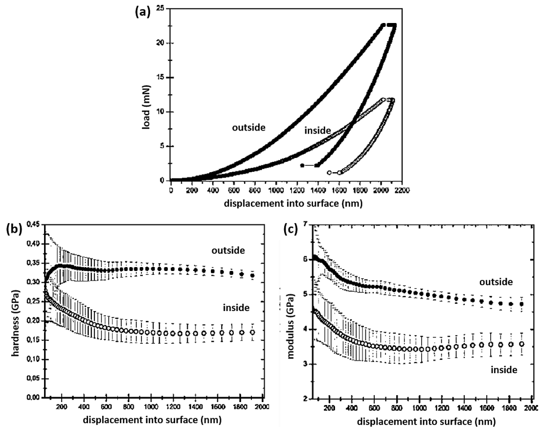
Figure 3.31 Variation in nanoindentation from the outer (outside) and inner (inside) scale layers in Kenyan sand boa Gongylophis colubrinus . (a) Load-penetration curves; (b) Hardness variation with penetration in outer and inner layers; (c) Effective elastic modulus as a function of penetration for outer and inner layers. The error bars denote the standard deviations [151].
