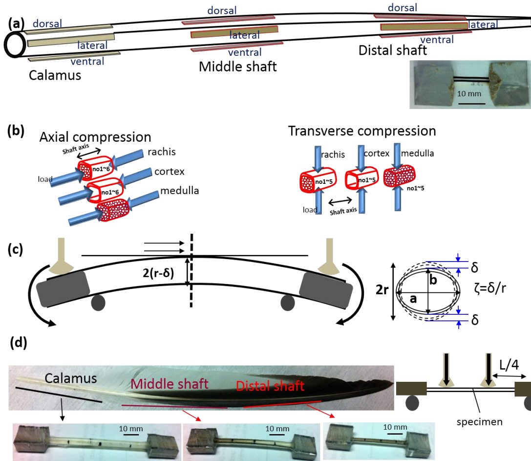
Figure 5.2 (a) Tensile tests on thin strips at dorsal, lateral and ventral regions at calamus, middle shaft and distal shaft, with a photo of specimen ready for test. (b) Axial and transverse compression specimens, both include rachis, cortex and medulla. (c) Pure bending of thin circular tubes, and the Brazier effect: the original circular cross section (dashed circles) deforms into an oval shape. The degree of ovalization, \zeta , is characterized by the ratio of \delta over r . (d) Four-point flexure along the shaft length including calamus, middle shaft and distal shaft; the two ends of each specimen were embedded in epoxy and square tubes.
