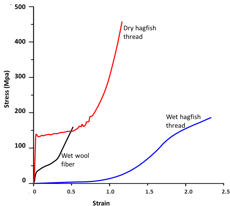
Figure 3.22 Tensile stress-strain curves of hagfish threads in seawater (blue), wet wool fibers (black) and a hagfish thread tested in air (red) (reproduced from [197]).
