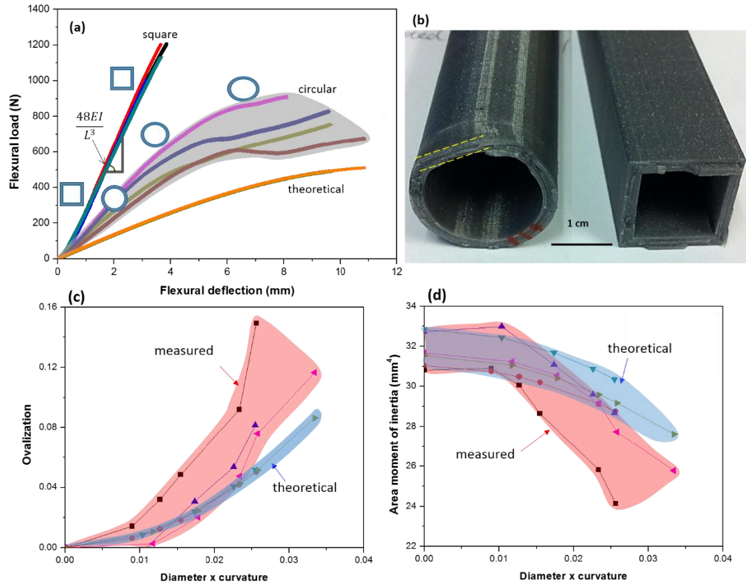
Figure 5.4 Flexural behavior of the 3D-printed PLA tubes with circular and square shapes: (a) flexural load-deflection curves, overlaid with theoretical calculated curves for circular tubes considering ovalization; (b) photo of the fractured surfaces. Pure bending of circular hollow PP tubes: plots of (c) measured degree of ovalization versus bending curvature (dimensionless), and (d) measured area moments of inertia versus bending curvature (dimensionless); overlaid plots shaded in blue are from theoretical calculations.
