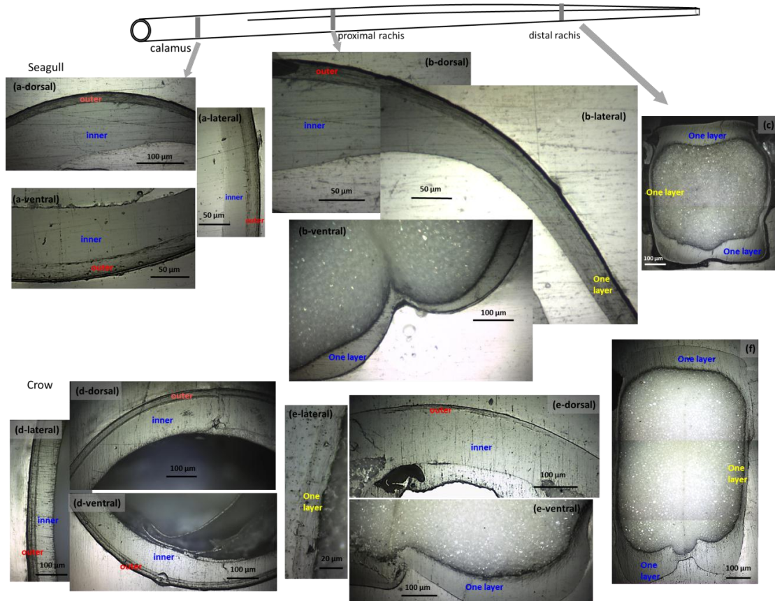
Figure 5.5 Optical micrographs of the transverse sections of feather shafts from the calamus to the distal shaft, showing the layered structure varying depending on local corticale regions and positions along the shaft length. Seagull feather: (a) calamus, (a-dorsal) dorsal region, (a-lateral) lateral wall, (a-ventral) ventral region; (b) proximal rachis, (c) distal rachis. Crow feather shaft shows similar layered structure: (d) calamus; (e) proximal rachis; (f) distal rachis. The outer layer and inner layer are indicated in red and blue, and the one layer in lateral wall in yellow.
