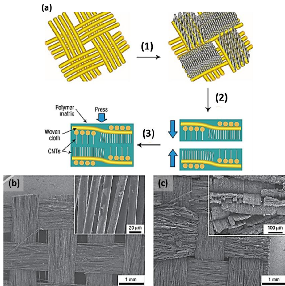
Figure 3.34 (a) Processing for the manufacture of 3D carbon nanotubes (CNT) composite: (1) aligned CNTs grown perpendicular to SiC fiber cloth; (2) stacking of matrix-infiltrated (blue color) CNT-grown fiber cloth; (3) 3D nanocomposite plate fabrication by hand lay-up. (b) Scanning electron micrograph of the plain-weave SiC fabric cloth. Insert: higher magnification of the individual fibers. (c) Scanning electron micrograph of the cloth with CNTs grown perpendicularly on the surface. Insert: higher magnification image [252].
