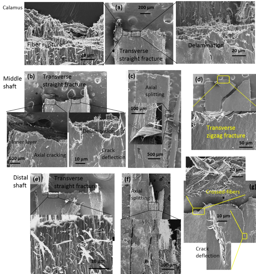
Figure 5.14 Side views of tensile fractured cortex specimens along the shaft length: at the calamus (a), the dorsal, lateral and ventral regions all show a transverse straight fracture due to rupture of the axial fibers, the circumferential fibers covering axial fibers, delamination and peeling off. The middle shaft (b) shows the same transverse straight fracture with axial cracking, crack deflection, and delamination, the ventral region (c) shows significant axial splitting, whereas (d) the lateral walls show transverse zigzag fracture due to crossed-fibers. At the distal shaft, the dorsal and ventral regions (e,f) exhibit transverse straight fracture, while the lateral walls (g) show cross fibers in layers and crack deflection.
