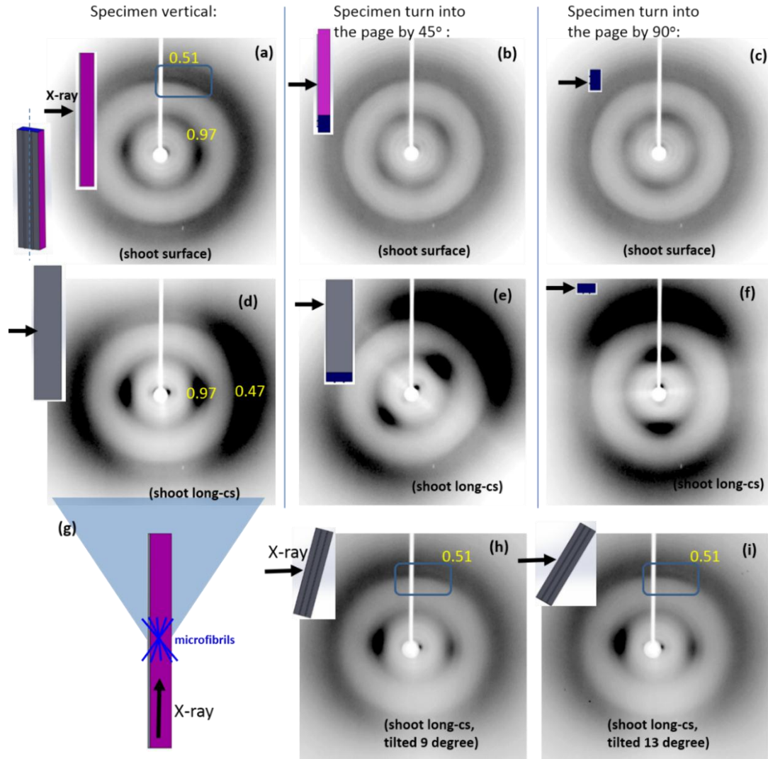
Figure 4.9 X-ray diffraction patterns of pangolin scale specimens. Top left is a schematic of the strip. (a,b,c) Diffraction patterns of x-ray shooting the scale surface with specimens vertical, turning into the page by 45 degree and turning into the page by 90 degree. (d,e,f) Diffraction patterns of x-ray shooting the long-cs with specimens vertical, turning into the page by 45 degree and turning into the page by 90 degree. (g) Illustration of the microfibrils aligned in a preferred range of directions and diffracting the x-rays to form a pattern in (d). (h,i) Diffraction patterns of x-ray shooting the long-cs with specimens tilted 9 and 13 degrees to show the characteristic 0.51 meridional reflection of \alpha -keratin.
