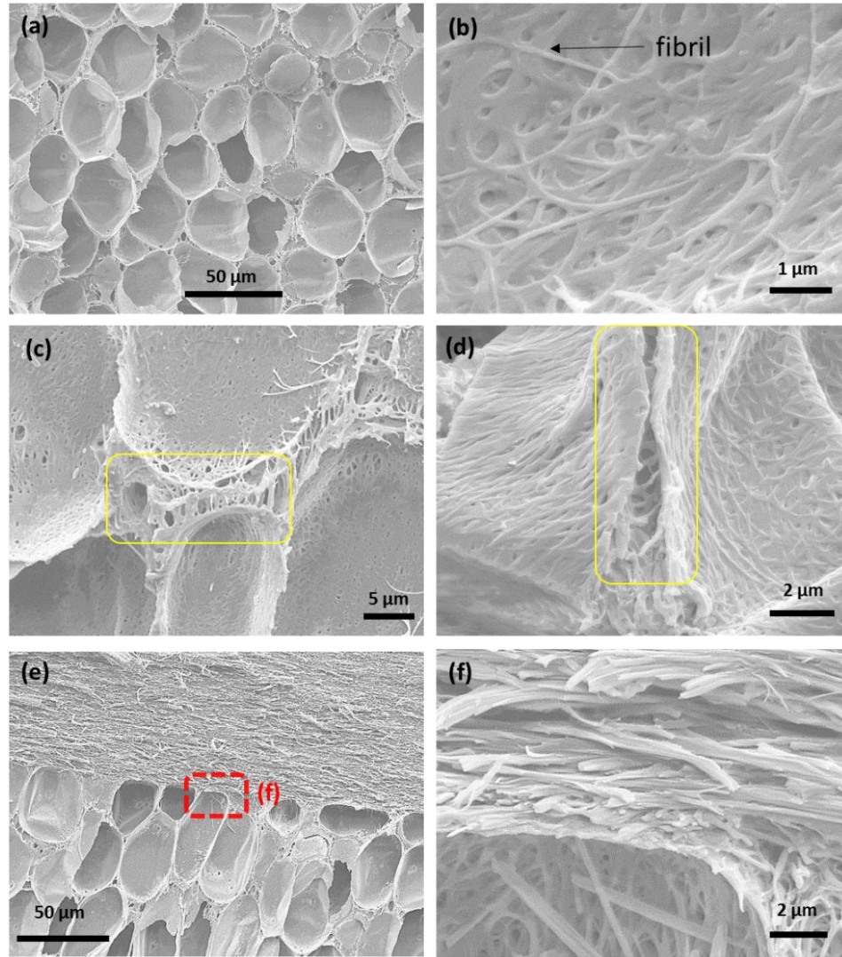
Figure 5.12 Scanning electron micrographs of the medulla: (a) closed-cell foam-like structure; the cells show near round shape with about 20-30 \mu\text{m} in diameter; (b) higher magnification image of the cell walls reveals the fibrous and porous structure at nanoscale, arrow pointing to fibrils; (c) and (d) the fibrous struts that connect and strengthen the cell wall interfaces (yellow rectangles); (e) longitudinal section of distal rachis at the interface of medulla and cortex; (f) higher magnification image of the area in red dotted rectangle in (e), the fibrils of cell walls merge well with those composing the cortex.
