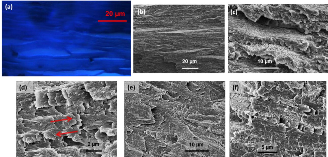
Figure 4.5 The lamellar structure formed by keratinized cells: (a) fluorescence micrograph of transverse cross section (tran-cs) of a scale, the cell profiles (upper) and the lamellae are clearly seen, indicating that keratinized cells form lamellae; (b) scanning electron micrographs of tran-cs of the scale showing (a) the lamellae and (c) that each lamella is one layer of cells. Scanning electron micrographs of the three regions showing the crossed-lamellae structure: (d) dorsal region, (e) middle region, and (f) inner region.
