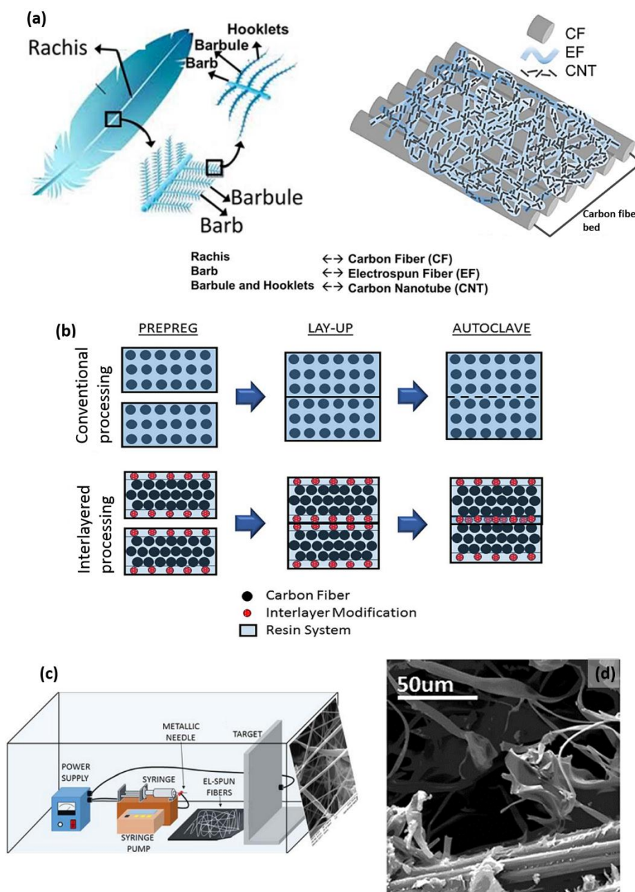
Figure 3.35 The feather-inspired composite with electrospun fiber interlayers: (a) the feather fractal architecture of rachis, barbs and barbules and the inspired the structure consisting of carbon fibers, electrospun fibers and carbon nanotubes; (b) conventional laminate composite and interlayered laminate; (c) electrospinning apparatus with the electrospun fibers on the right; (d) flexural fractured surface of the composite at the carbon nanotube reinforced electrospun fiber interlayer [253].
