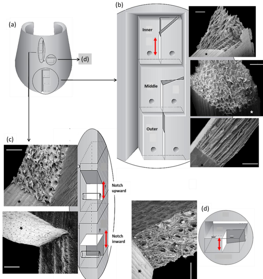
Figure 3.19 Crack diversion mechanisms (white areas indicate notch surfaces with asterisks, and dark gray areas fracture surfaces) and scanning electron micrographs of fracture surfaces of equine hoof (scale bars, 1 mm). Red arrows indicate the tubule direction. (a) Specimens in three groups: along the thickness direction, at middle region with notches parallel and perpendicular to tubules, and at middle region with notches trans-passing tubule axis. (b) At inner, middle and outer regions of the hoof wall with notches upward parallel to tubule axis and the crack paths, and the fracture surfaces. (c) Specimens with notches upward and inward and the crack paths, and the fracture surfaces. (d) Specimens with notch inward and the crack path, and the fracture surface [181].
