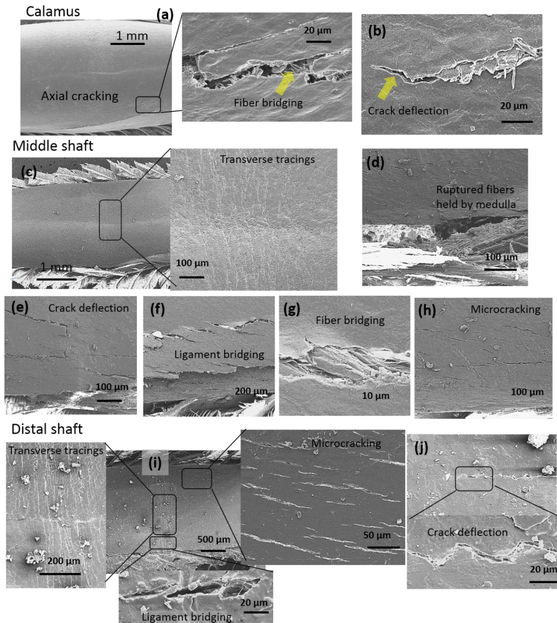
Figure 5.19 The dorsal views of the buckled feather shaft along the shaft length: (a,b) the calamus, showing significant axial cracking and minor crack deflection and fiber bridging; (c-h) the middle shaft, showing transverse tracings at the buckled region, and ruptured fibers held by the medulla, crack deflection, ligament and fiber bridging, and microcracking; (i-j) the distal shaft with similar features as those in the middle shaft.
