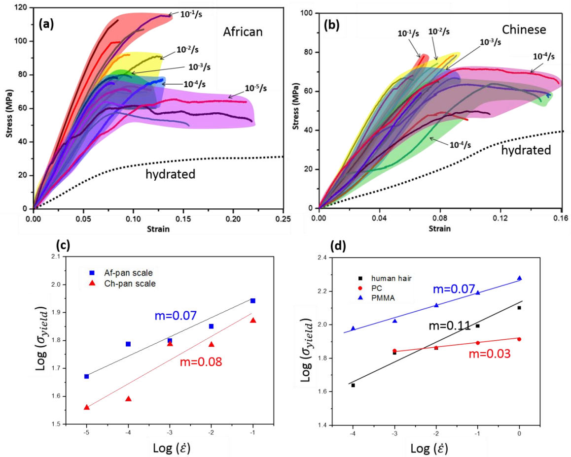
Figure 4.13 Strain rate and hydration sensitivity of pangolin keratin: (a) tensile stress-strain curves of African tree pangolin scales stretched longitudinally (Long-Ori) at different strain rates, and the hydrated 100% relative humidity, dotted curves), showing significant decrease in strength and stiffness; (b) tensile stress-strain curves of Chinese pangolin scales stretched longitudinally (Long-Ori) at different strain rates, and the tensile behavior of the hydrated specimen (100% relative humidity, dotted curves); (c) strain rate sensitivities of African tree and Chinese pangolin scales, calculated via Eq. (2) with yield stresses obtained from (a) and (b); (d) strain rate sensitivities of human hair (keratinous material) and typical polymers (polycarbonate, PC, and polymethyl methacrylate (PMMA)).
