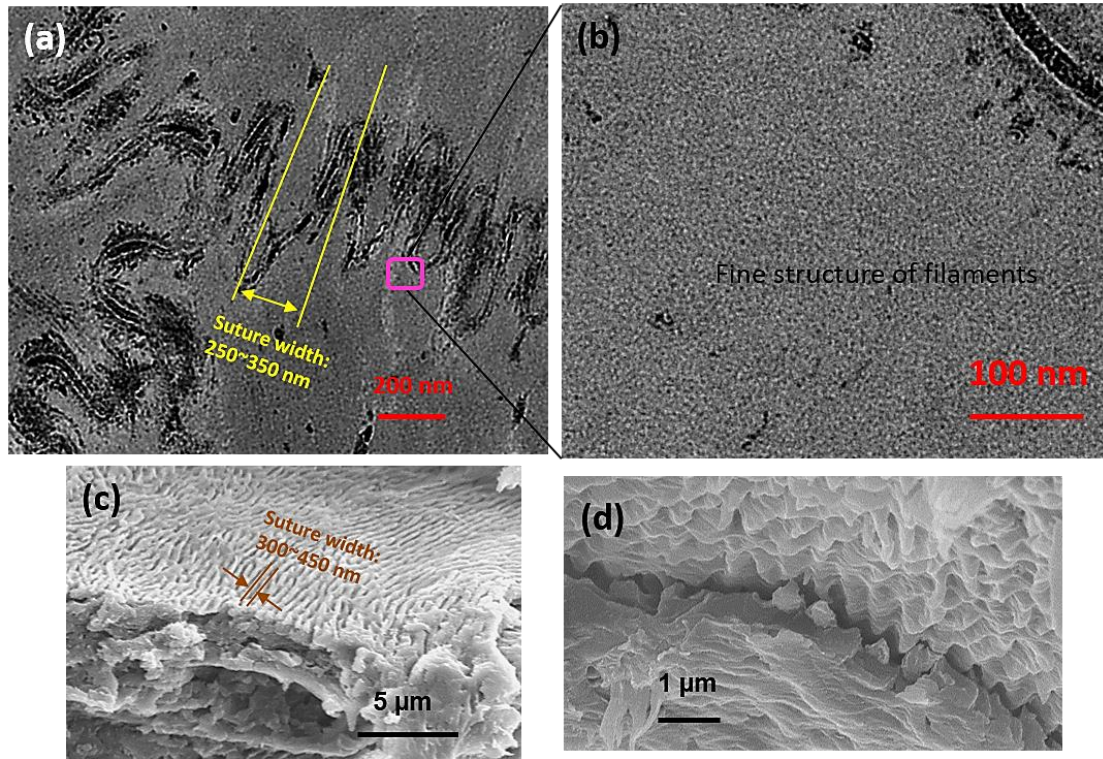
Figure 4.8 The suture-like cell membrane complex and the fine filaments of pangolin scales: (a) transmission electron micrograph of transverse cross section (tran-cs) of a scale. The cell membrane complex (about 25-50 nm thick) consists of one densely-stained central layer and two less dense layers, typical of keratinous materials, but interestingly shows suture-like profile (suture width ~350 nm); (b) transmission electron micrograph of the area in (a) showing the fine filaments about 3~5 nm in diameter inside cells. Scanning electron micrographs: (c) tran-cs of the scale, the lamellae also show fine suture-like protrusions, since they are formed from flattened keratinized cells; (c) and (d) the suture-like cell membrane complex provides interlocking interface between lamellae.
