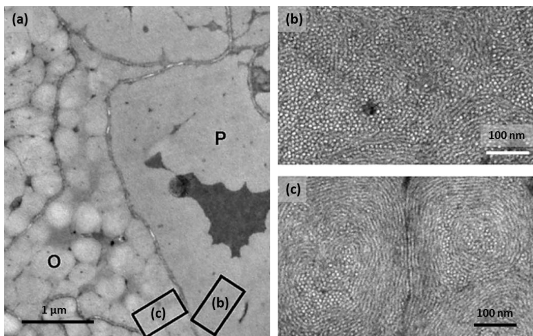
Figure 3.15 Transmission electron micrographs of a red deer hair: (a) cross section of the hair showing the paracortex (P) and orthocortex (O). High magnification images of rectangular regions (b and c) are shown in (b) and (c); (b) hexagonally arranged IFs embedded in matrix in paracortex; (c) IFs arranged in a whorl-like pattern in orthocortex [179].
