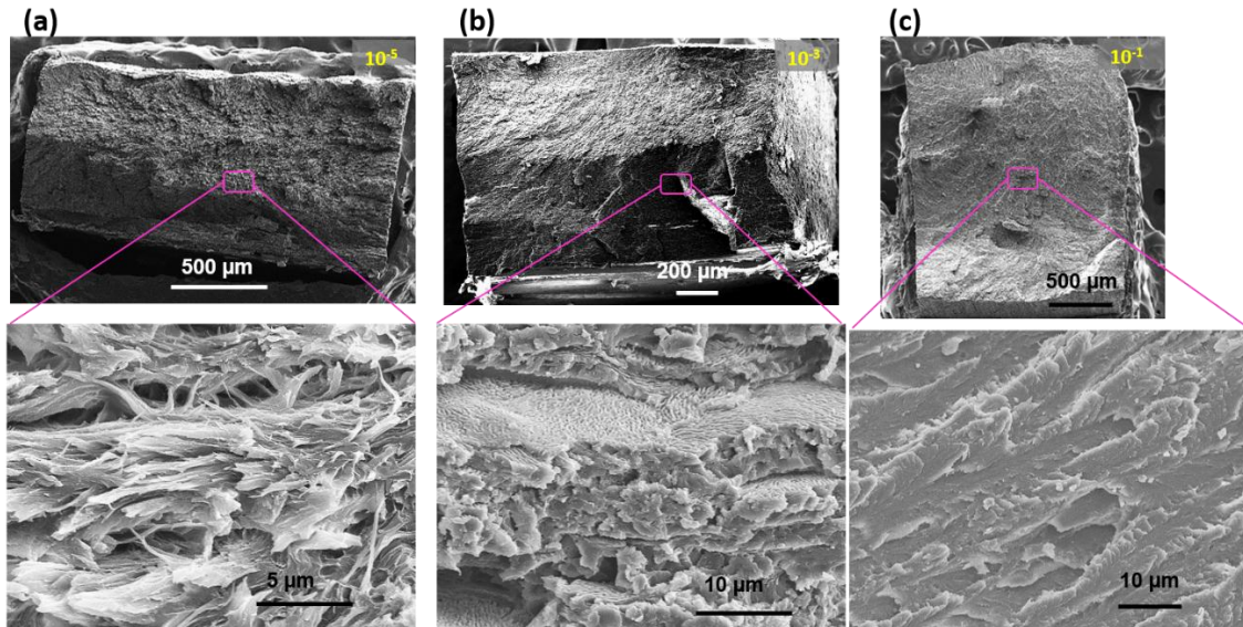
Figure 4.14 Tensile fractured surfaces of the pangolin scale at (a) 10^{-5}/s , (b) 10^{-3}/s and (c) 10^{-1}/s . The fracture mode changes from fiber tear and fracture (lamellae delaminate into fibers) to lamella pull-out (lamella with surface suture) and trans-lamella fracture (smooth lamellar & cross-lamellar fracture) as strain rate increases.
