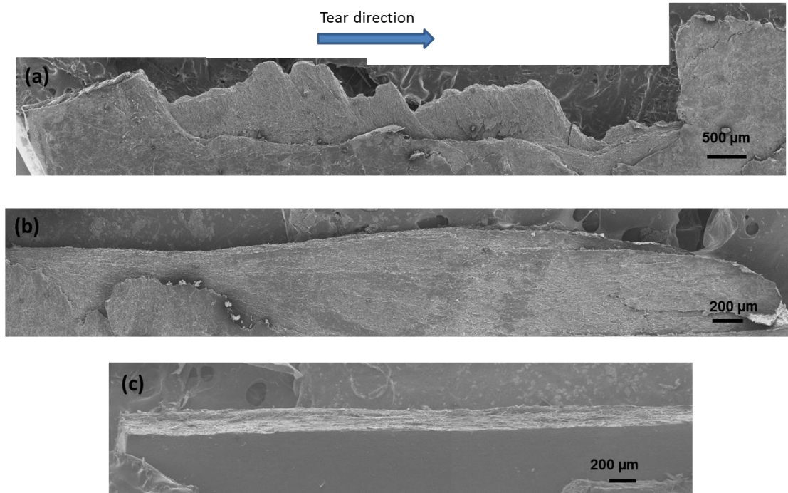
Figure 4.7 Side views of tear fractured (a) pangolin scale exhibiting zigzag profile, indicating that fibers are oriented in angles to scale longitudinal direction, whereas (b) fingernail and (c) feather rachis show smooth torn edge, indicating uniaxially aligned fibers.
