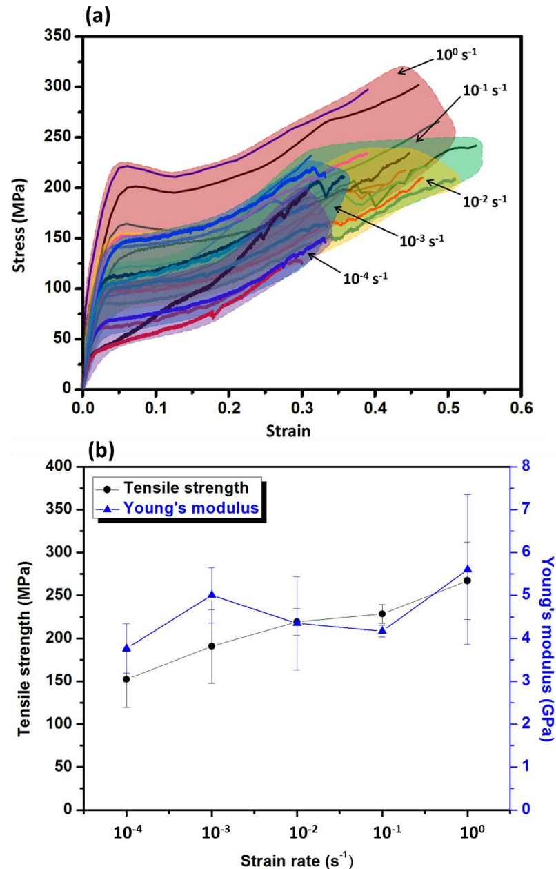
Figure 3.16 Tensile results of human hair at different strain rates [180]: (a) stress-strain curves grouped for each strain rate; (b) Young's modulus and tensile stress as a function of strain rate (error bars indicate standard deviation).
