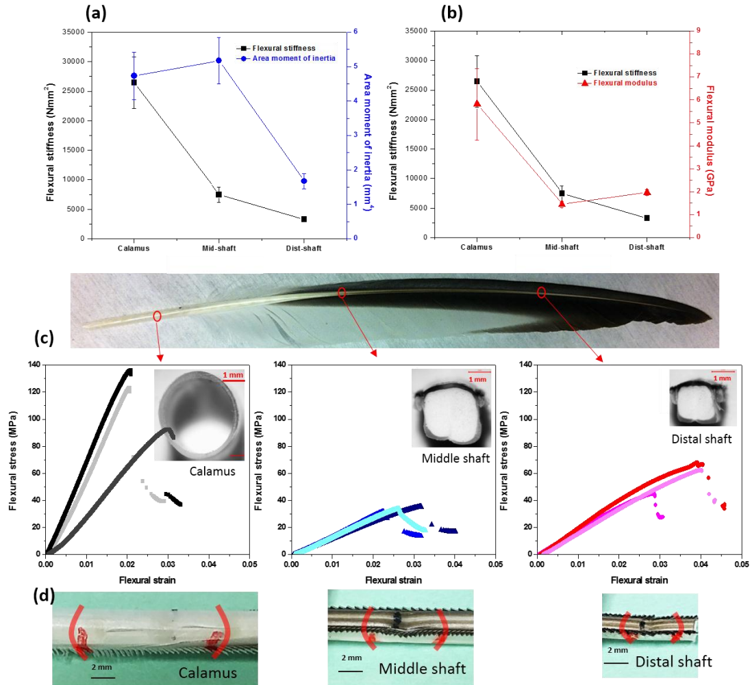
Figure 5.18 Flexural responses of seagull feather shaft: (a) flexural stiffness and area moment of inertia along the shaft length; (b) flexural stiffness and modulus along the shaft length; (c) flexural stress-strain curves of the calamus, middle shaft and the distal shaft, with the sectional views; (d) local buckling failure during flexure at the calamus, middle shaft and distal shaft.
