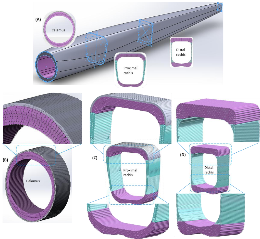
Figure 5.11 Structural model of the feather shaft cortex. (a) The cross section changes from circular at the calamus to near rectangular at rachis. The layered fibrous structure of cortex: (b) at the calamus, all the cortex consists of a thin outer layer of circumferential fibers and a thick inner layer of axial fibers; (c) at the proximal rachis, the dorsal cortex consists of a thinner outer layer of circumferential fibers covering axial fibers, the lateral walls of crossed-fibers and the ventral cortex of axial fibers; (d) at the distal rachis, the dorsal and ventral regions are composed of axial fibers and the lateral walls of crossed-fibers.
