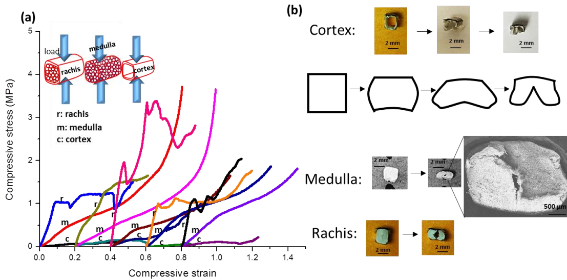
Figure 5.17 Transverse compression: (a) stress-strain curves of rachis, medulla and cortex specimens; (b) deformation mechanisms of cortex, medulla and rachis.
