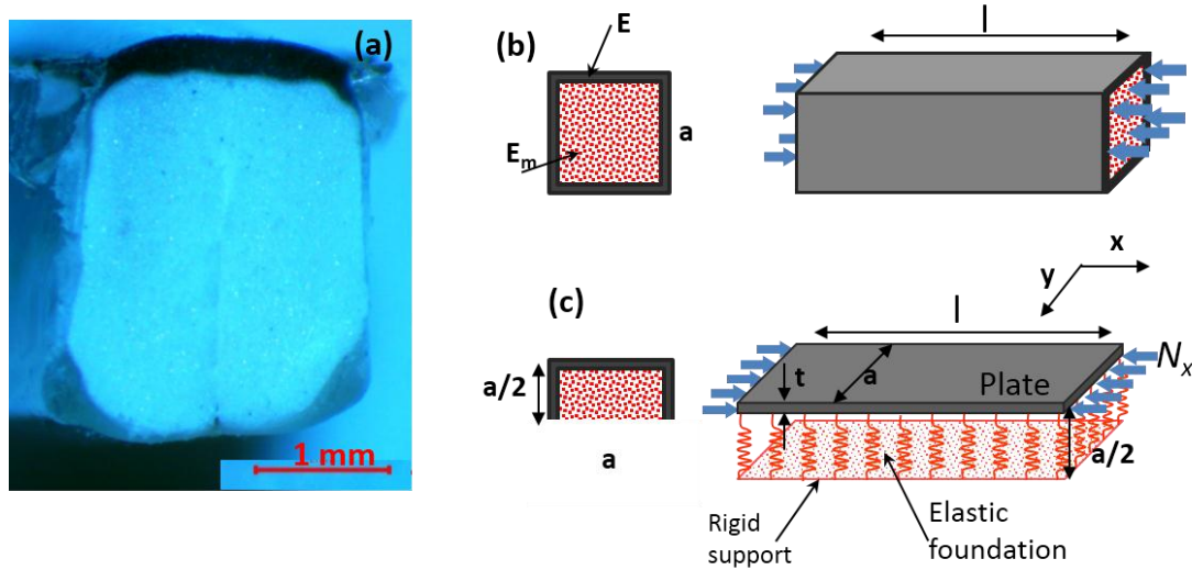
Figure 5.16 Axial compression model: (a) image of transverse section of one specimen; (b) schematics of the square tube with a foamy core under axial loading; (c) schematics of the plate supported by an elastic foundation under in-plane compressive loading.
