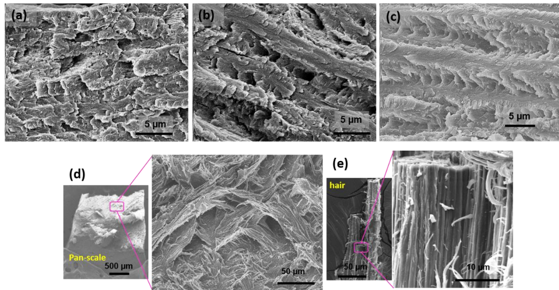
Figure 4.6 Crossed-lamellar and crossed fiber structure of pangolin scales: (a) dorsal region (freeze fractured), (b) middle region (freeze fractured), and (c) ventral region (10-1/s). Side views of tensile fractured specimens in three keratinized biological materials: (d) pangolin scale in hydrated state, showing crossed-fibers, (e) human hair composed of uniaxial fibers.
