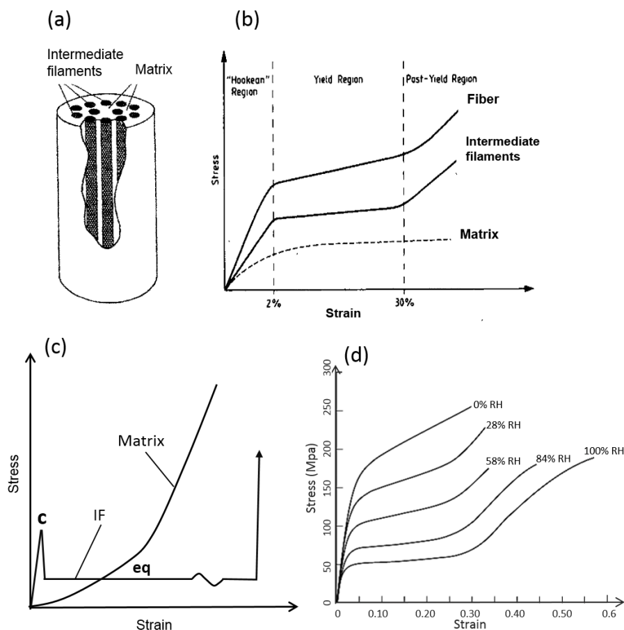
Figure 3.14 (a) Two-phase composite model for a wool fiber: cylinders of intermediate filaments (IFs) embedded in matrix [165]; (b) schematic stress–strain curve proposed for a wool fiber in water (not drawn to scale) [166]; (c) stress–strain curves of independent IF and matrix from a modified two-phase model (c, critical stress; eq, equilibrium stress) (reproduced from [167]); (d) stress–strain curves of wool fibers at different relative humidities (RH) [38].
