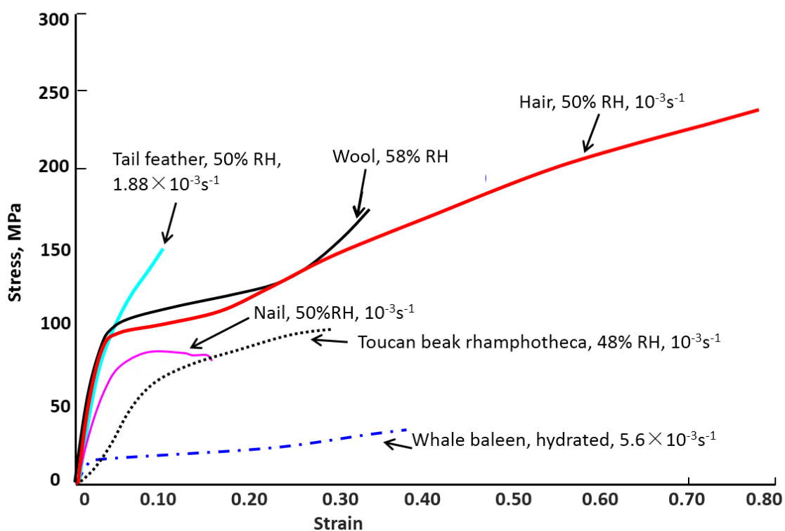
Figure 3.10 Tensile stress-strain curves of several typical keratinous materials (wool from [38], whale baleen from [144]).
