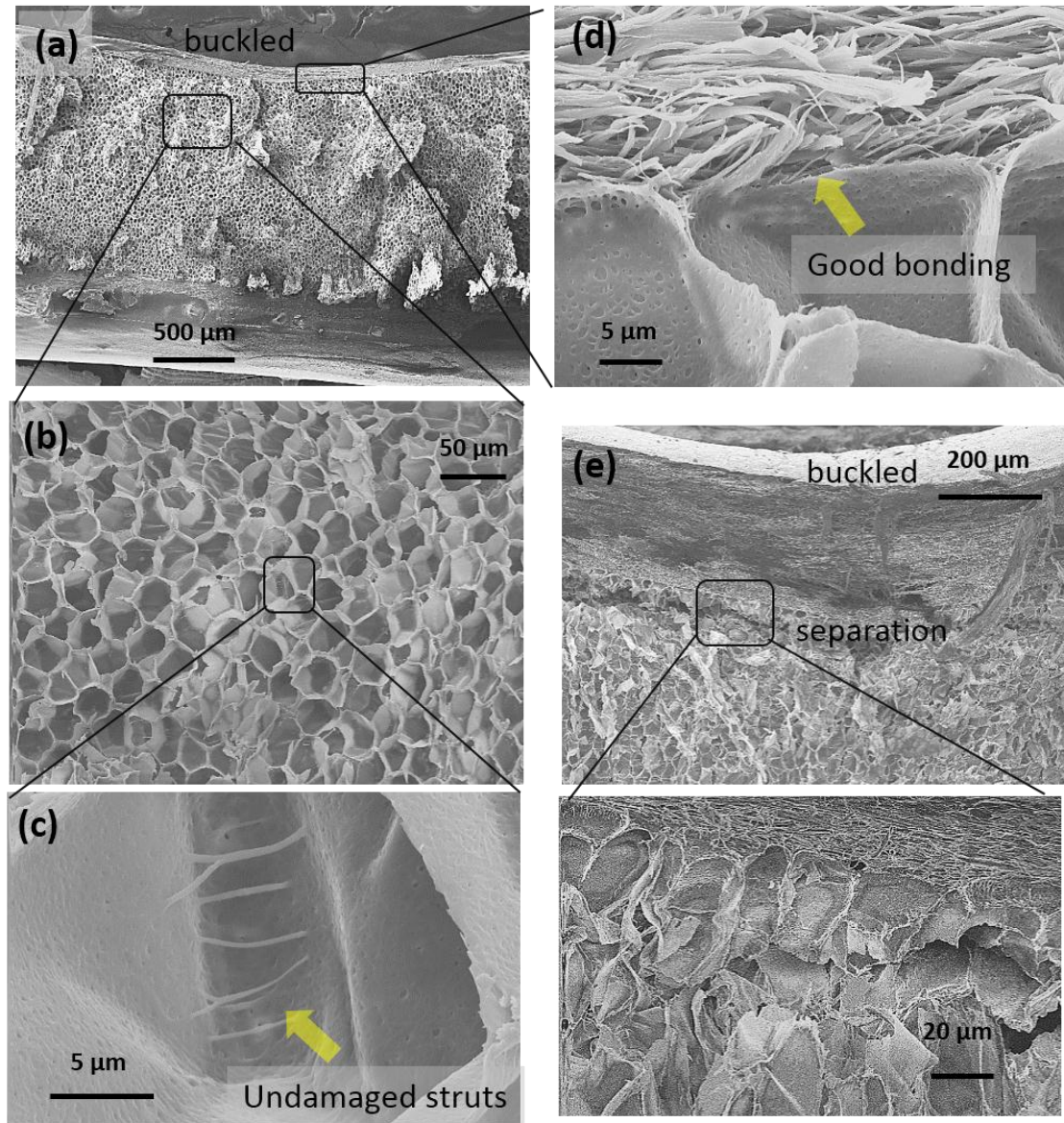
Figure 5.20 Sectional views of the buckled feather rachis: (a,b) the medullary cells show mostly original shape and show undamaged fibrous struts at inter-cell walls (c). (d) The bonding between medulla and cortex remains well. (e) The apparent separation within foamy medulla (below the cortex) is indeed very shallow, and the cells remain connected
