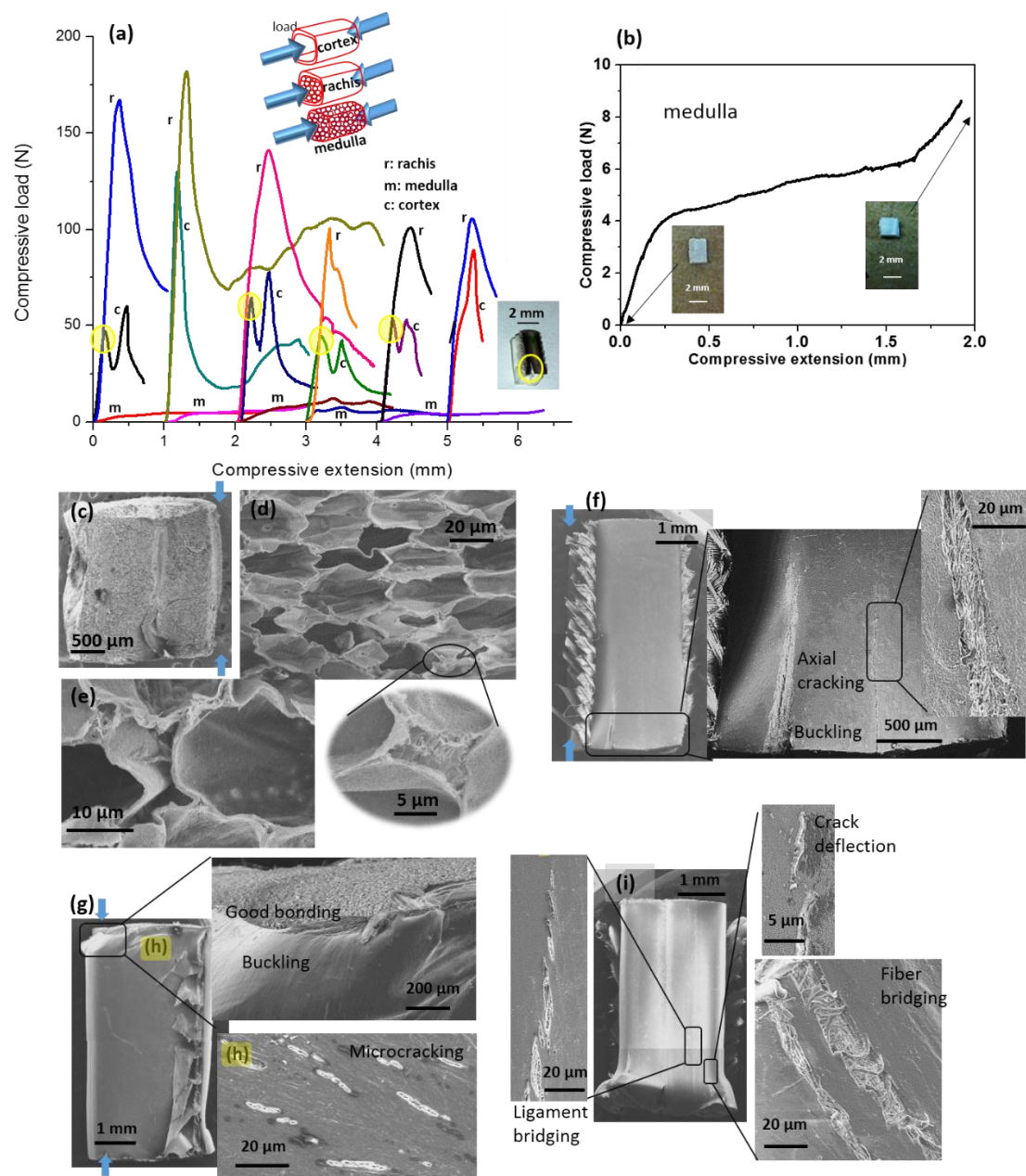
Figure 5.15 Axial compression. (a) Load-extension curves of the cortex, medulla and rachis specimens. The first load drop in cortex is due to axial splitting. (b) Load-extension curve of medulla. Scanning electron micrographs of (c) compressed medulla (blue arrows indicate loading direction), (d) medullary cells showing deformed shape, while the fibril bundles at the cell interface remain connected; (e) the deformed cell edges. (f) Compressed cortex with axial cracking and buckling. (g-h) Compressed rachis with uniform buckling and microcracking. (i-j) Severely compressed rachis with toughening mechanisms.
