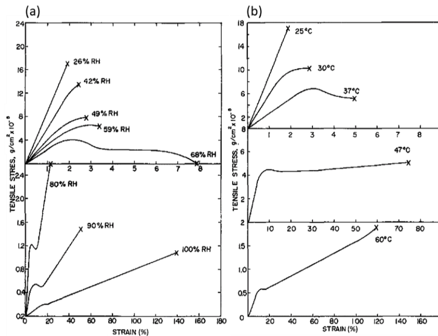
Figure 3.12 Tensile tests (stress-strain curves) of new born rat stratum corneum at strain rate of 0.5 cm/min [157]: (a) curves at 25°C and different humidities; (b) curves at 10% water content at different temperatures.
