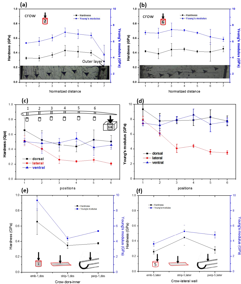
Figure 5.10 Nanoindentation results from crow feather shaft: along dorsal cortex thickness from inner to outside (a) at the calamus (position #2) and (b) the distal rachis (position #6); (c,d) on dorsal, lateral and ventral regions along the shaft length; (e,f) on dorsal and lateral pieces in different loading directions. Each data point represents an average of five measurements and error bars represent standard deviations.
