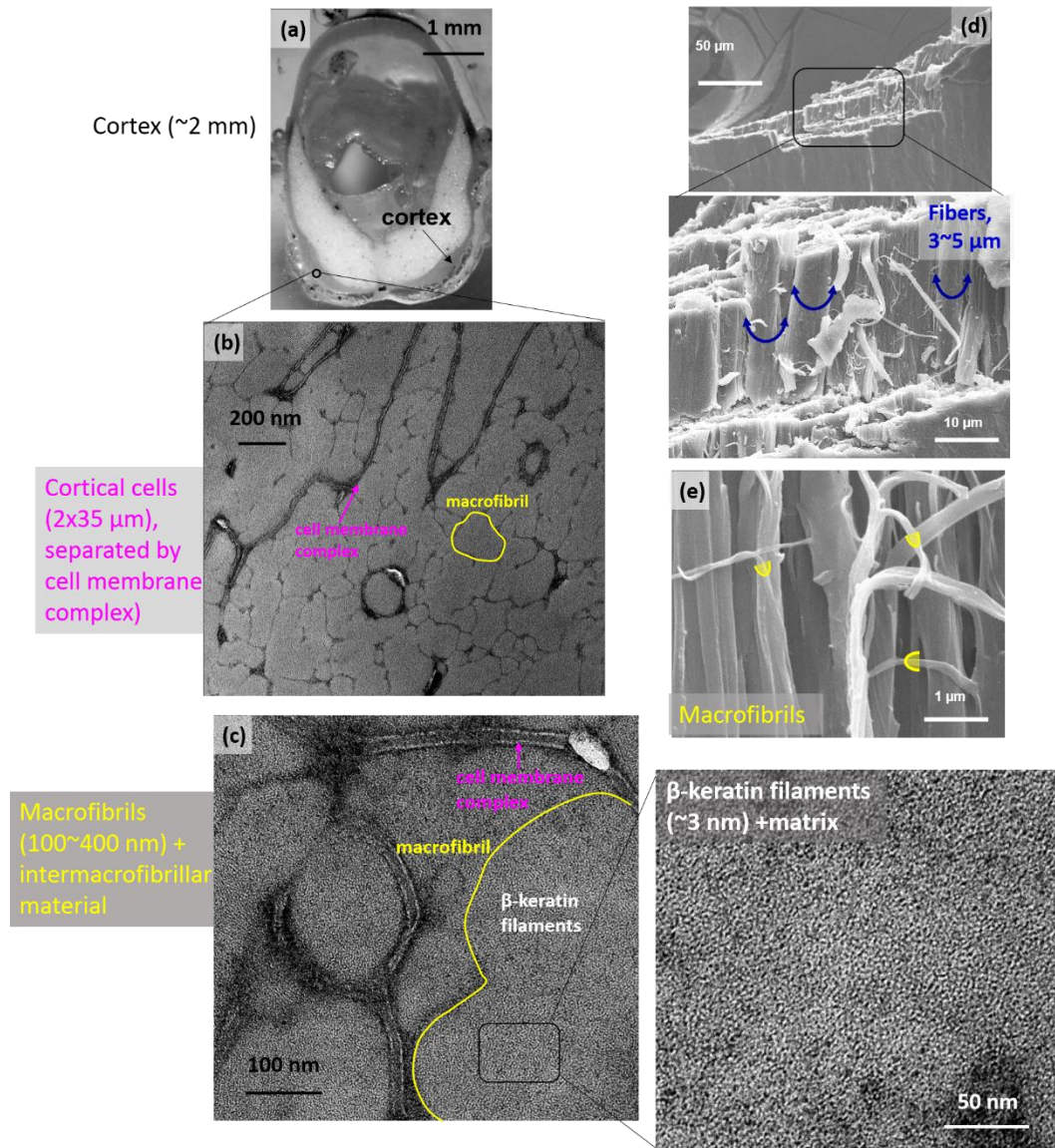
Figure 5.8 The hierarchical fibrous structure of seagull rachis: (a,b,c) transmission electron micrographs of transverse sections showing the cortex, cortical cells separated by cell membrane complex, macrofibrils outlined by intermacrofibrillar material, and \beta -keratin filaments embedded in matrix. Scanning electron micrographs of tensile fractured ventral strip of rachis, lateral view: (d) axially aligned fibers, bulk fibers about \sim 5 \mu\text{m} (blue doubled arrows). (e) An image shows the macrofibrils (50-300 nm in diameter, yellow semi-circles), which agree with those in transmission electron micrographs.
