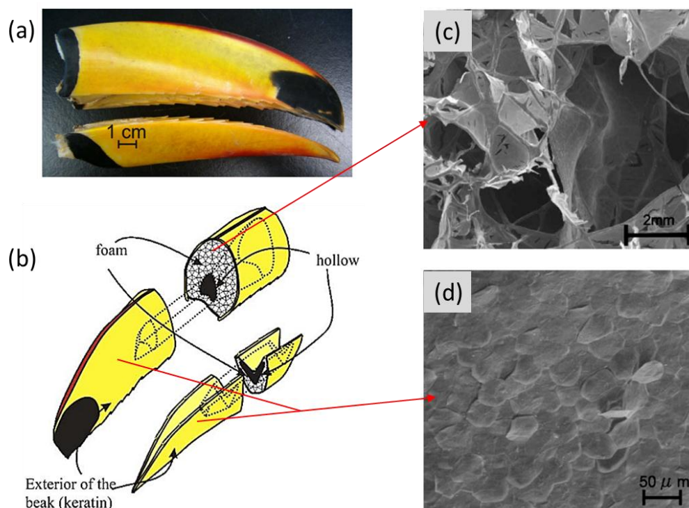
Figure 3.25 Structure of a Toco toucan beak: (a) Photograph of the beak showing maxilla and mandible [214]; (b) schematic showing internal and external structure; (c) scanning electron micrograph of the interior of beak, showing the foam with closed cells (several are crushed/ripped); (d) scanning electron micrograph of the rhamphotheca, (keratinous surface) showing the keratin scales [213].
