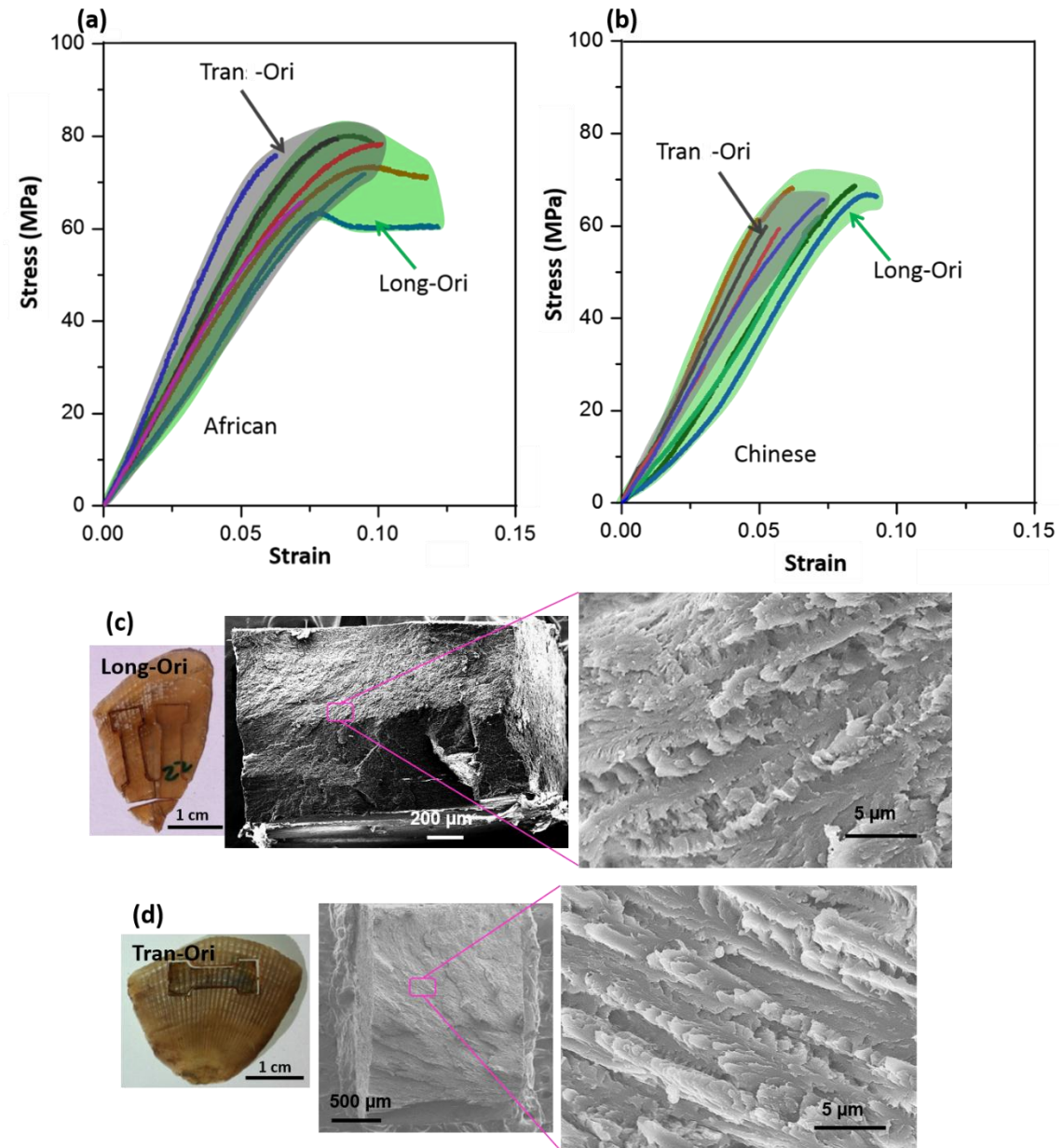
Figure 4.11 Tensile response of the (a) African pangolin and (b) Chinese pangolin scales loaded in longitudinal (Long-Ori) and transverse (Tran-Ori). Fracture surfaces of Chinese pangolin scales from (c) Long-Ori and (d) Tran-Ori.
