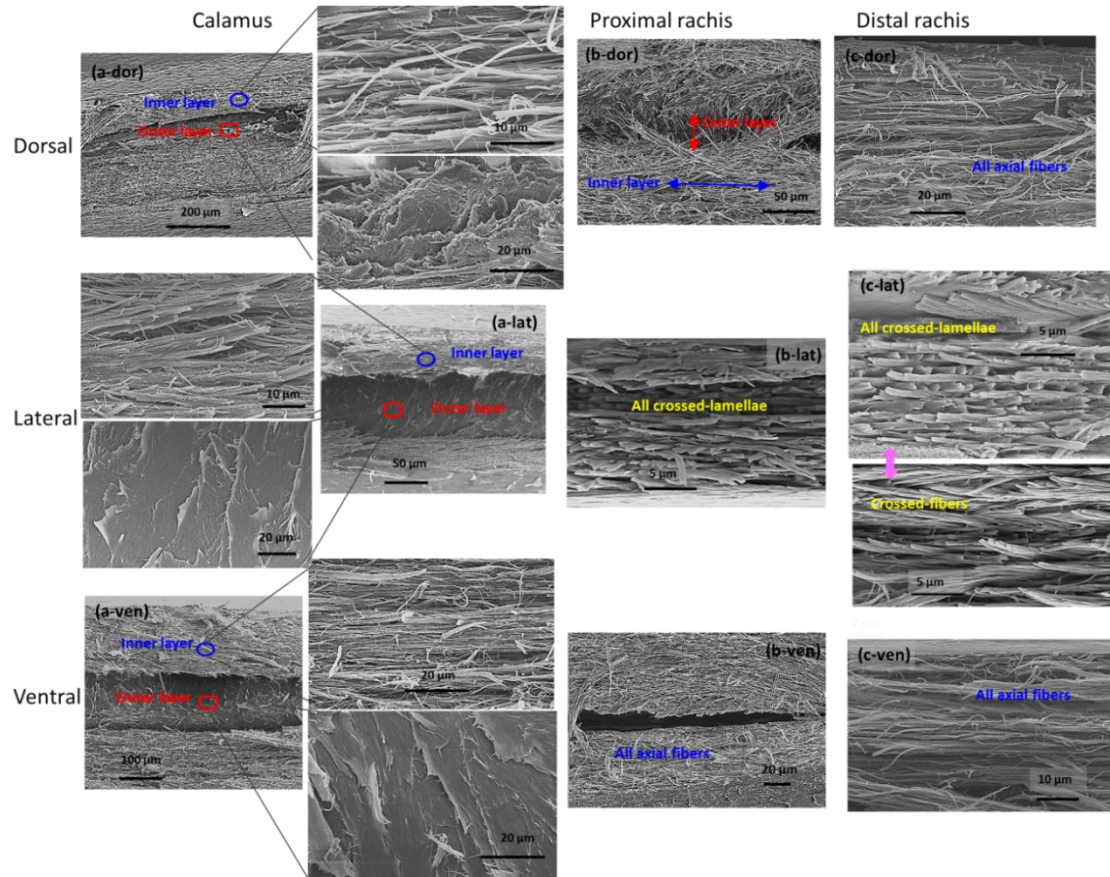
Figure 5.7 Scanning electron micrographs of the longitudinal sections at the dorsal, lateral and ventral regions of the cortex from crow feather, which shows the same fibrous structure as that of seagull: (a) at the calamus, (b) at the proximal rachis, (c) at the distal rachis.
