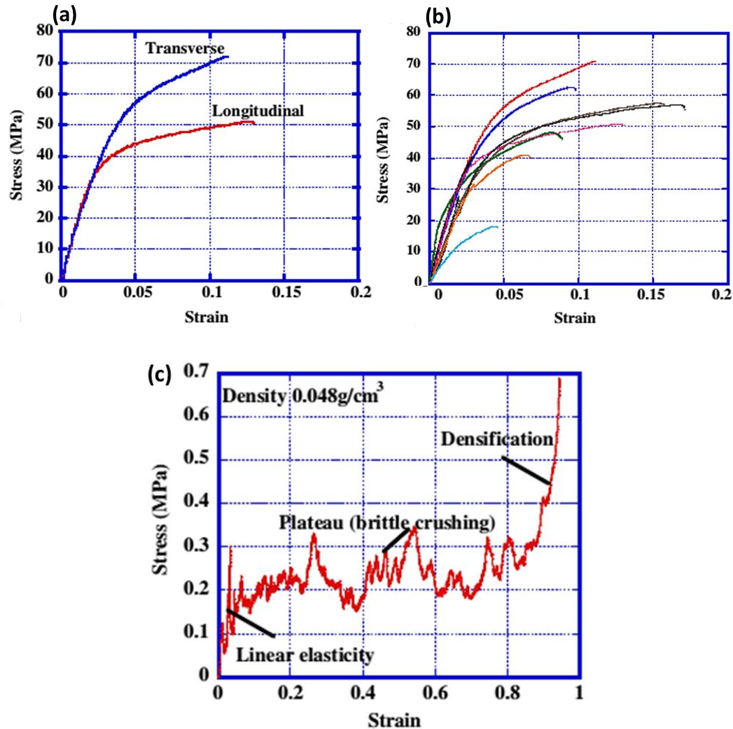
Figure 3.26 Mechanical properties of a Toco toucan beak: (a) representative tensile stress-strain curves of the rhamphotheca along transverse and longitudinal orientations [213]; (b) tensile stress-strain curves showing the scatter of results; (c) compressive stress-strain curve of the interior foam showing characteristic cellular response [150].
