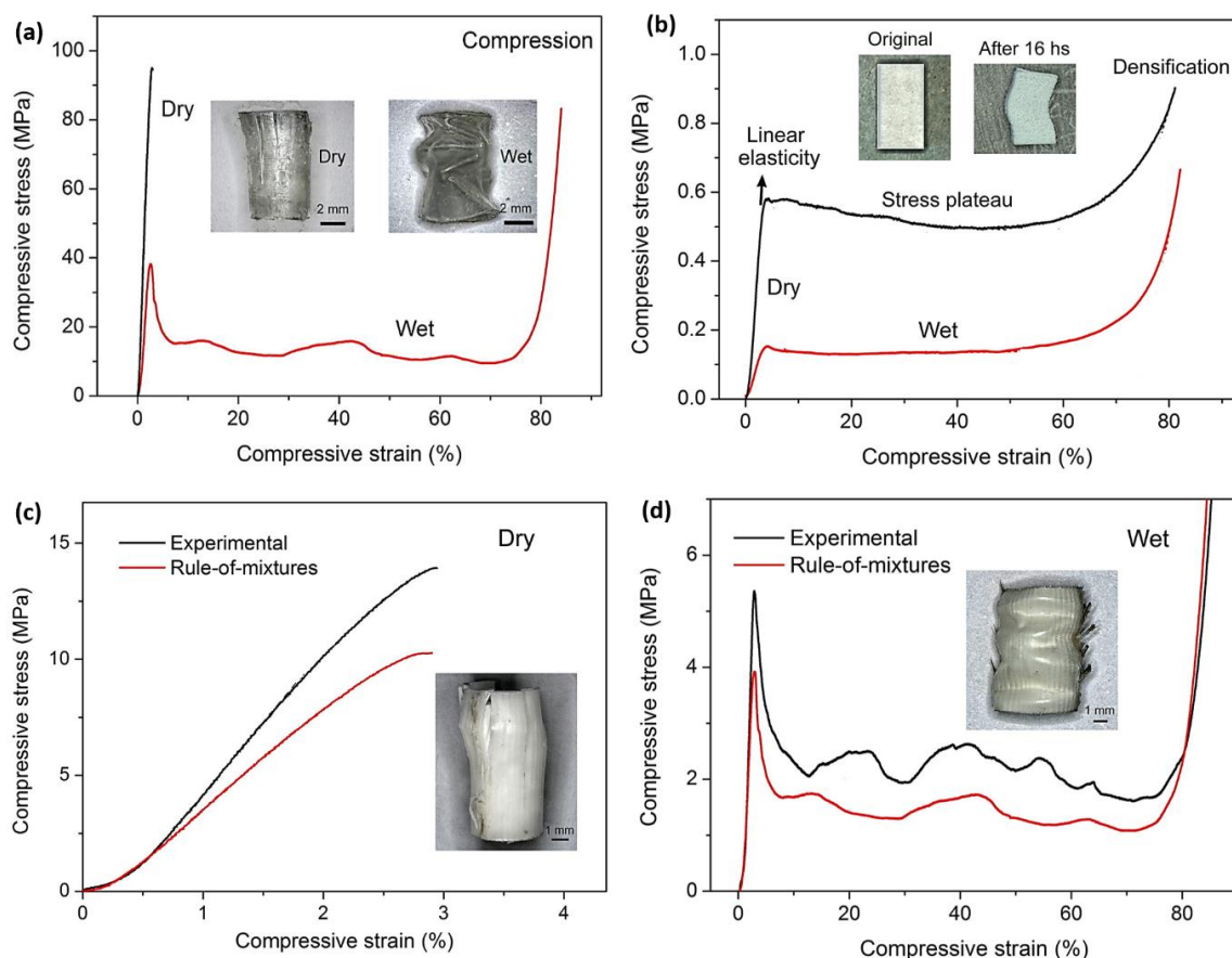
Figure 3.24 Compressive behavior of tail feather from peacock: (a) stress-strain curves of cortex at dry and wet conditions; (b) stress-strain curves of medullary foam at dry and wet conditions; stress-strain curves of experimental overall rachis and the calculated ones at (c) dry and (d) wet conditions [203].
