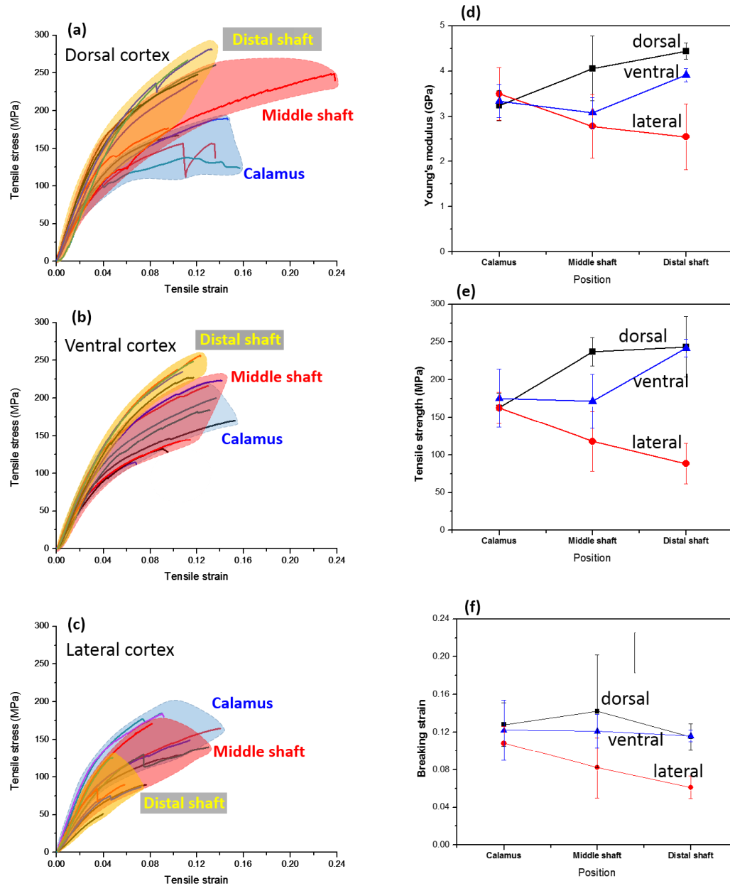
Figure 5.13 Tensile responses of seagull cortex strips along the shaft length: stress-strain curves of (a) dorsal cortex, (b) ventral cortex, (c) lateral cortex at the calamus, middle shaft and distal shaft; Variation of (d) Young's modulus, (e) tensile strength, (f) breaking strain of the dorsal, lateral and ventral cortex strips along the shaft length.
