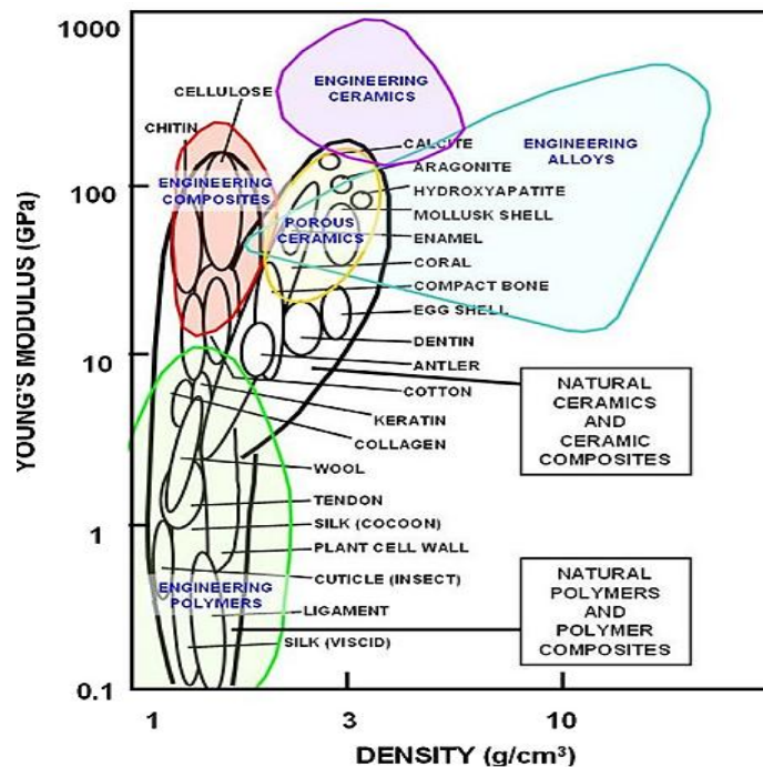
Figure 1.3 Young's modulus as a function of density for biological materials, overlaid with synthetic materials [10], [12], [25].
