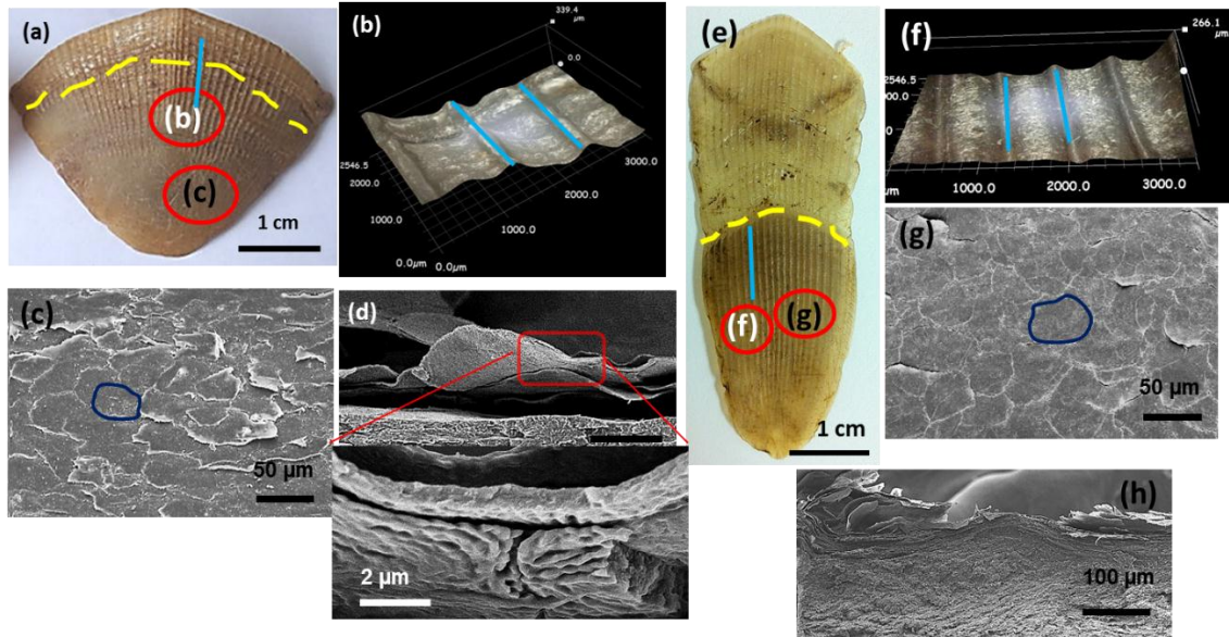
Figure 4.3 Scale surface structure: (a) Chinese pangolin scale. (b) 3D optical micrograph of the scale external surface showing the longitudinal ridges parallel with growth direction; (c) plane view of the external surface showing the keratinized cuticle cells; (d) transverse cross section of the scale at the superficial 3~5 layers of cuticle cells and an image of the keratin mesh morphology; (e) African pangolin scale. (f) 3D optical micrograph of the scale external surface showing the longitudinal ridges parallel with growth direction; (g) plane view of the external surface showing the keratinized cuticle cells; (h) transverse cross section of the scale at the superficial 3~5 layers of keratinized cells.
