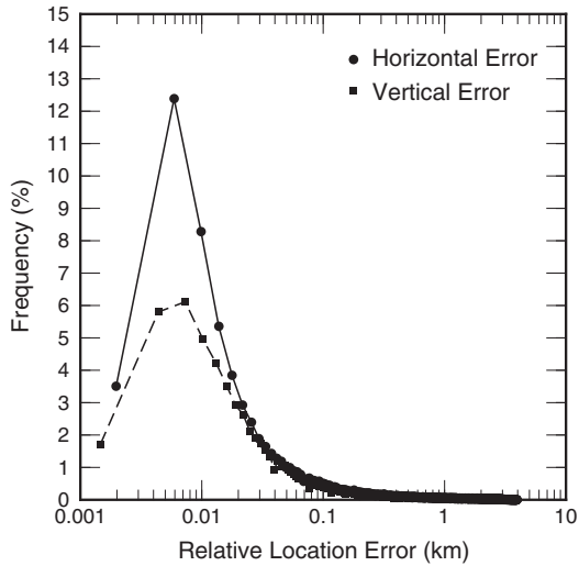
Figure 6. Histograms of formal relative location errors estimated by bootstrapping. For the horizontal errors (circles, solid line), the 5th, 25th, 50th, 75th, and 95th percentiles are 4 m, 12 m, 64 m, 544 m, and 2248 m, respectively. For the vertical errors (squares, dashed line), they are 4 m, 16 m, 71 m, 516 m, and 1758 m, respectively.
