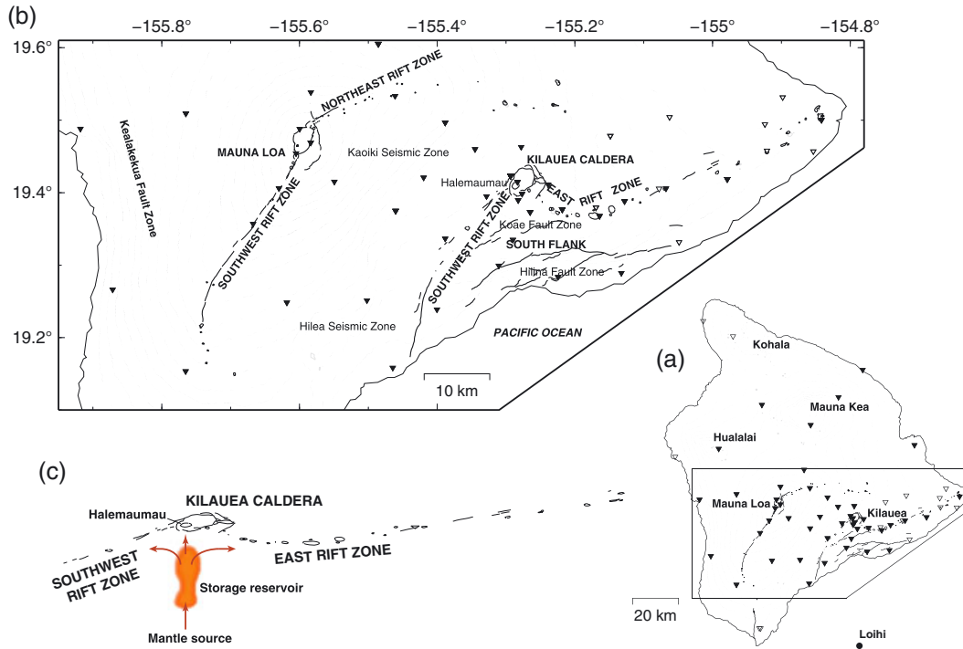
Figure 1. (a) Map of the island of Hawaii showing the locations of volcanoes (Kilauea, Mauna Loa, Mauna Kea, Hualalai, Kohala, and Loihi seamount), major faults and craters, and 60 seismic stations operated by the USGS HVO and the NOAA PTWC from which data were considered in this study (inverted triangles) [Nakata and Okubo, 2010]. Solid black inverted triangles are stations recording at least 30% of all events considered. Contour interval is 300 m. Polygon indicates area of Figure 1b. (b) Expanded view of region in Figure 1a showing the principal morphological and seismic features of Kilauea and Mauna Loa volcanoes discussed in the text. Contour interval is 200 m. (c) Schematic of Kilauea's magma system (after Tilling and Dvorak [1993]), including a mantle source, a pathway of magma transport up from the mantle, a shallow (2–6 km) subcaldera storage reservoir marked by low seismicity and deformation centroids of inflation and deflation, and shallow lateral distributaries from this reservoir into two rift zones to the east and southwest.
