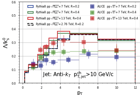
Fig. 1. The \Lambda/k_s^0 ratio in inclusive jets with different jet cone-size ( R=0.2,0.4 ) as a function of associated hadrons p_T for p-p collision at different collision energy ( \sqrt{s_{NN}}=2.76, 7 and 13 TeV)
