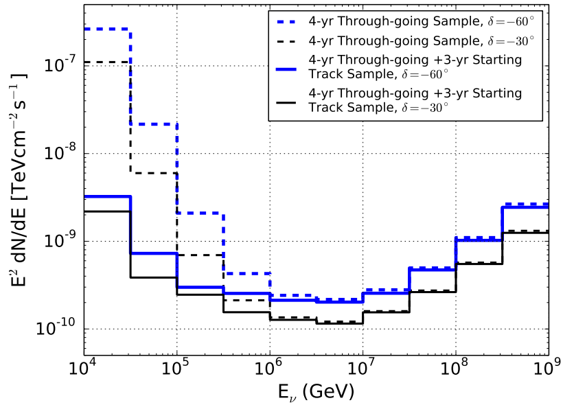
Fig. 1.— Discovery flux as a function of neutrino energy at 5\sigma confidence level. Point sources with an E^{-2} spectrum are simulated over a half-decade in energy, and the flux in each bin required for discovery forms the curve above. Previous IceCube results (Aartsen et al. 2014d) are shown with dashed lines. The new event selection lowers the discovery threshold at 10^5 GeV by a factor of \sim 10 .
