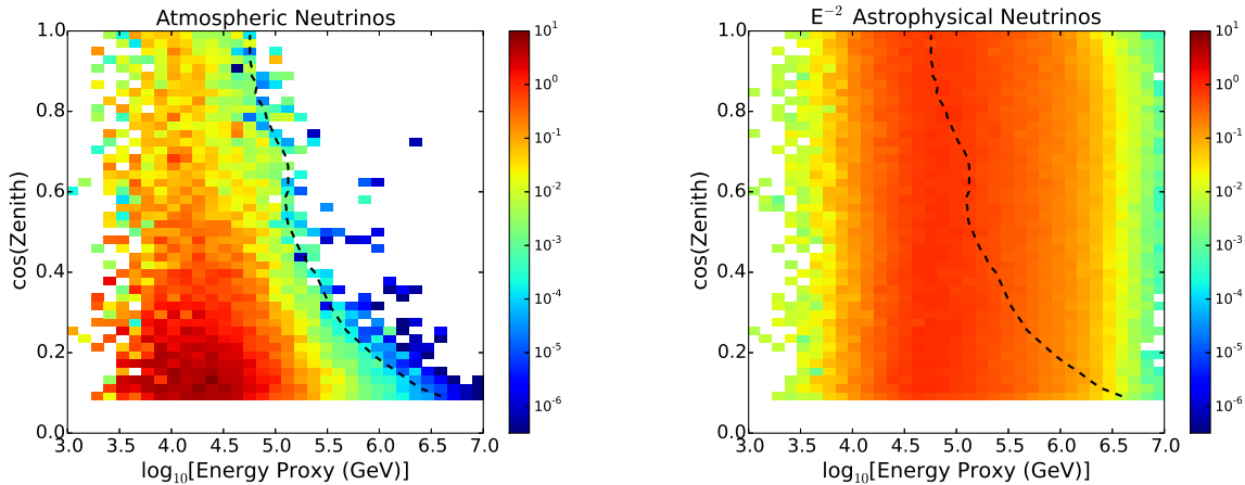
Fig. 4.— Atmospheric \nu_\mu background and astrophysical signal PDFs. The left plot shows the PDF as a function of reconstructed zenith angle and reconstructed energy for atmospheric neutrinos following models from Honda et al. (2007); Enberg et al. (2008); Gaisser (2013); Aartsen et al. (2014c). This includes the self-veto probability from Gaisser et al. (2014) for each event. The right plot shows the PDF for E^{-2} astrophysical neutrinos. The likelihood ratio between the signal and background hypothesis is calculated for the observed event’s energy and zenith, and the dashed line denotes the zenith-energy contour with this likelihood ratio. Events to the right of this contour are more “signal-like” than the observed event.
