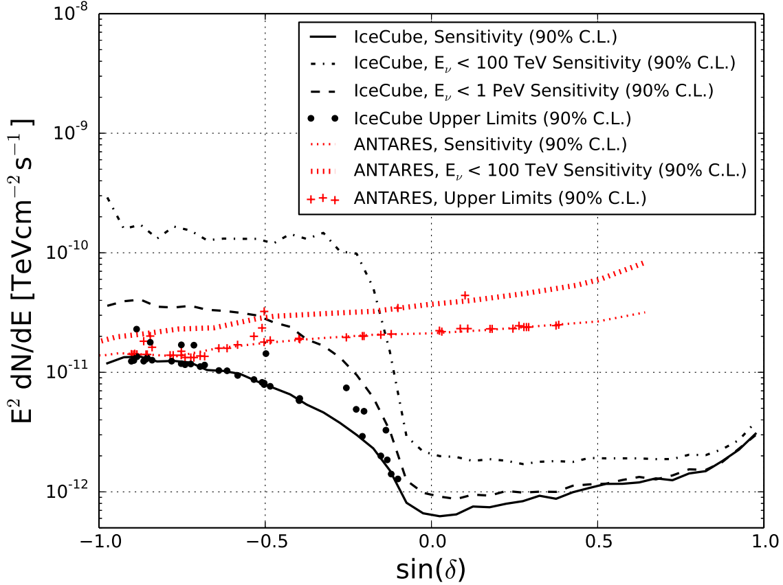
Fig. 3.— Muon neutrino upper limits (90% C.L.) evaluated for 38 sources (dots), for the three-year starting track sample combined with the four-year throughgoing muon sample. The solid black line is the median 90% C.L. upper limit or sensitivity for a point source with an unbroken E^{-2} spectrum. The sensitivities to E^{-2} spectra ending (with a sharp cutoff) at 1 PeV and 100 TeV are shown in the black dashed and dash-dotted lines, respectively. The ANTARES (1338 days livetime) upper limits and sensitivities for two spectral hypotheses are shown in red (Adrian-Martinez et al. 2014).
