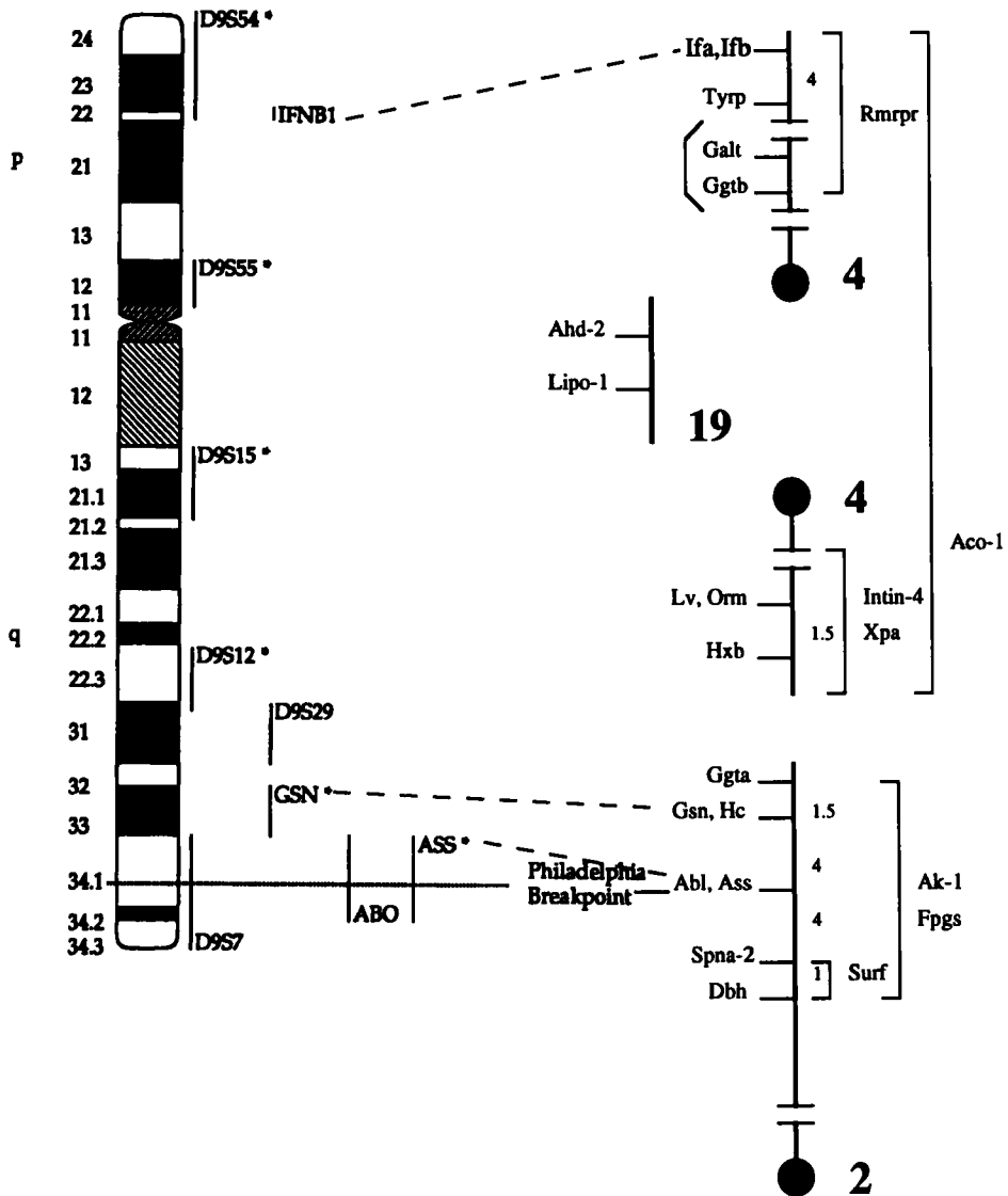
Fig. 7. Conserved mouse linkages and synteny aligned to the human chromosome 9. The centromere, where orientation is known, is represented by a filled circle. Chromosome 4 is displayed twice in order to allow the alignment to be shown. Genes where precise localization is not known in the mouse are displayed to the side and bracketed around the limits of their location. Where human and mouse nomenclature differs markedly both names are noted at the foot. Distances on the mouse chromosomes, where known accurately from at least one large backcross pedigree, are shown in cM.
