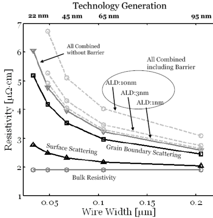
Figure 7.26: Cu resistivity in terms of wire width taking into account the surface and grain boundary scattering and barrier effect. The barrier layer is assumed to be uniformly deposited, e.g., using atomic layer deposition (ALD) [87].
