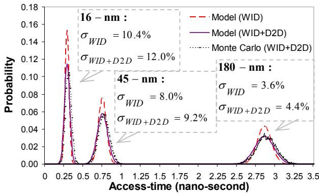
Figure 4: Verifying the proposed model with Monte Carlo.
