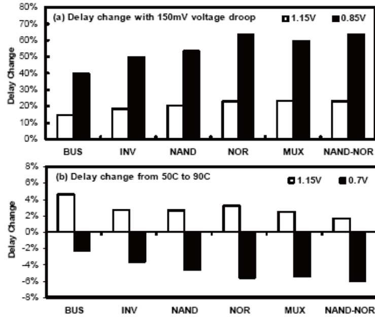
Fig. 4: Measured delay change to V_{cc} & Temp.
