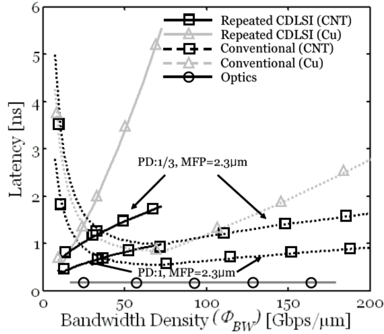
Figure 7.44: Delay vs. bisectional bandwidth density ( \Phi_{BW} ). For optics, WDM technique is assumed. (Total 10 wavelengths with 10Gbps/ch bandwidth) [87].
