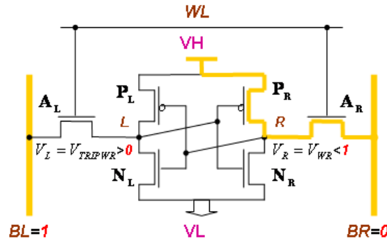
Figure 8.2: Write Failure: Memory cell does not register an input change correctly.
