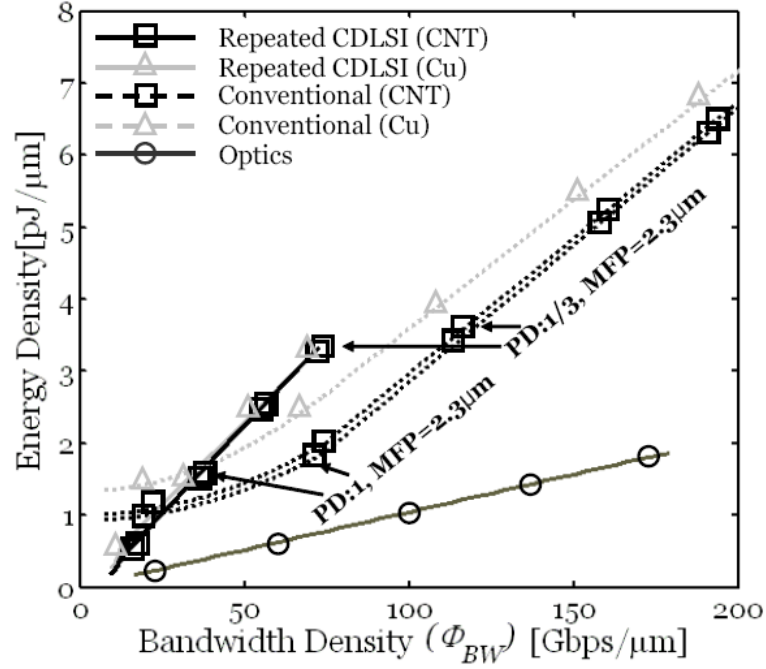
Figure 7.45: Energy Density vs. bisectional bandwidth density ( \Phi_{BW} ). For optics, WDM technique is assumed. (Total 10 wavelengths with 10Gbps/ch bandwidth) [87].
