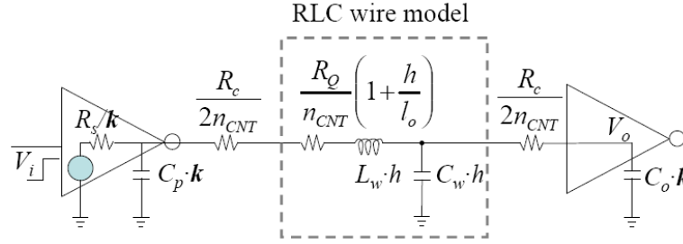
Figure 7.34: Equivalent circuit model of a repeater segment for CNTs. k is the optimized repeater area. h is the optimized wire length per repeater. R_s is inverter output resistance. R_c and R_Q are the contact resistance and quantum resistance of SWCNT, respectively. L_w and C_w are the inductance and the capacitance of CNT bundle, respectively. C_p and C_o are the input capacitance and the output parasitic capacitance of the inverter, respectively. n is the number of segments the length L is divided into [87].
