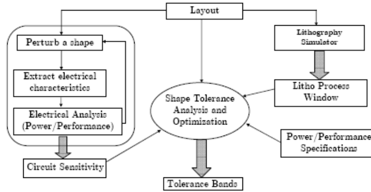
Figure 2.6: Flow for generation of tolerance bands [15].
