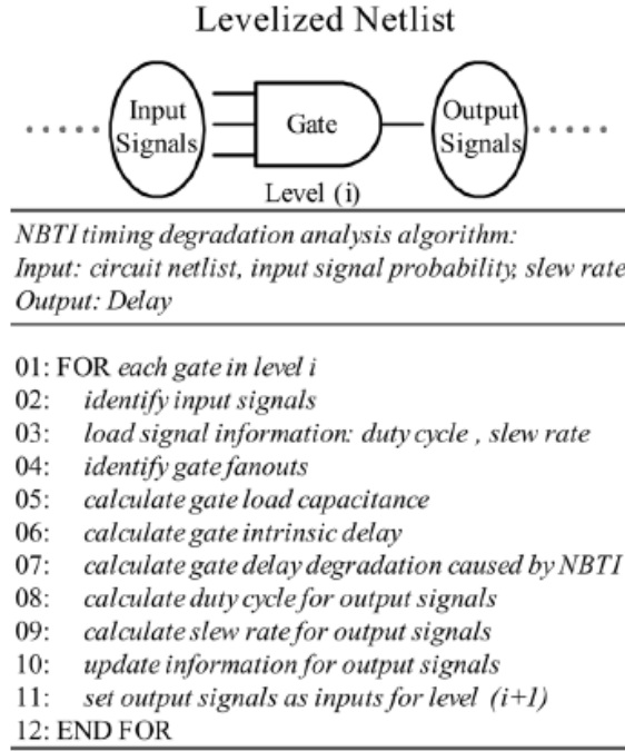
Figure 6.10: Timing degradation analysis algorithm [184].
