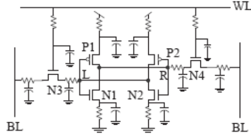
Figure 2.3: 6 Transistor SRAM Schametic with RC network [197].
