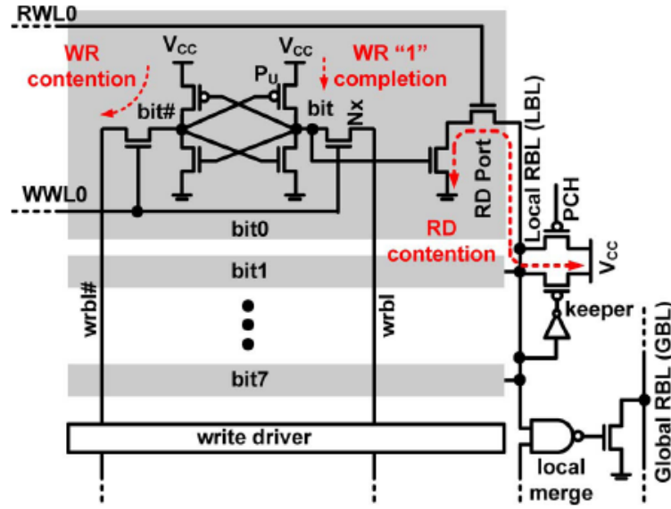
Figure 7.13: The 8T-SRAM cell architecture showing the WR and RD ports [143].
