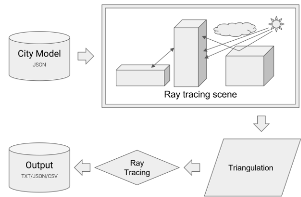
Figure 2 Flow chart of the ray tracer program.
