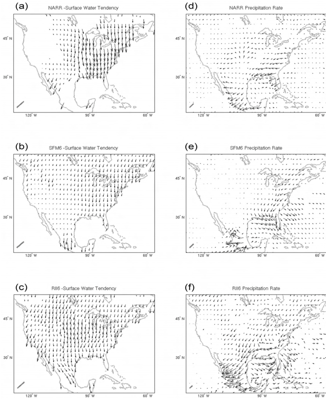
Figure 2.8: As in Fig. 2.5, but for negative surface water tendency ( a , b , and c ) with a reference length of 10 mm/day and precipitation rate ( d , e , and f ) with a reference length of 4 mm/day. Note that, for clarity, the unit vector in f has been shortened to prevent overlap of larger values.
