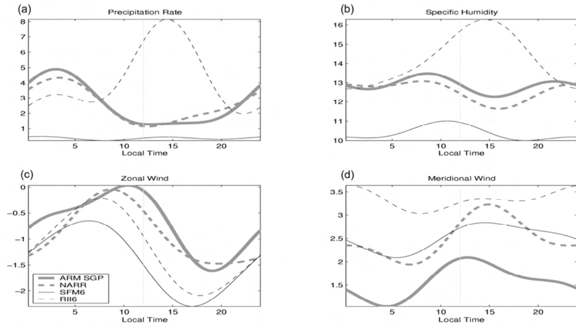
Figure 2.2: As in Fig. 2.1, but for a) precipitation rate (mm/day), b) 2-meter specific humidity (g/kg), c) 10-meter zonal winds (m/s), and d) 10-meter meridional wind (m/s).
