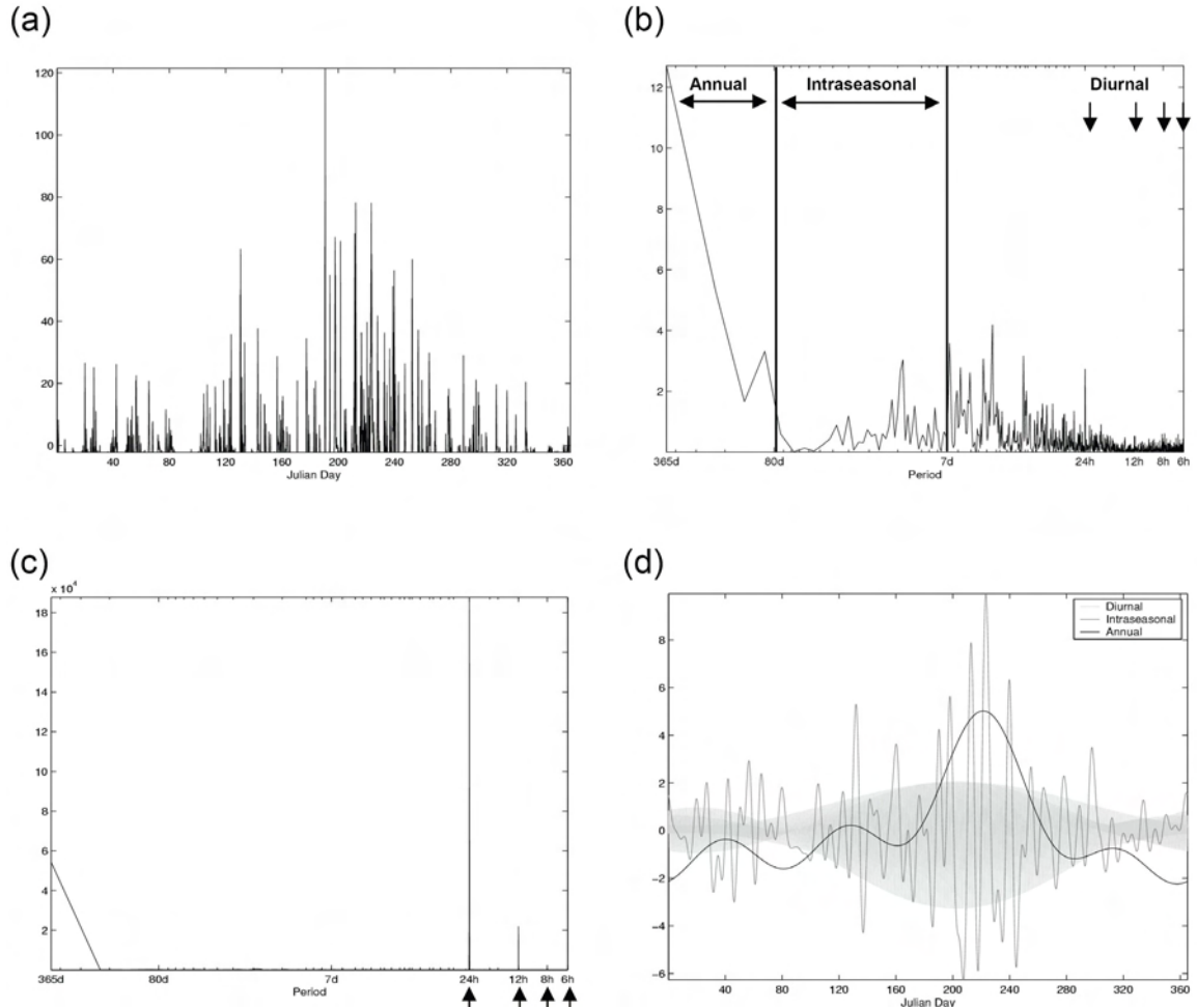
Figure 4.2: Methodology example for Lindenberg, Germany, in 2002; (a) 3-hourly precipitation rate (mm/day; deviation from the mean); (b) variance spectrum of precipitation rate ([mm/day] 2 ) with variance category definitions; (c) variance spectrum of surface downward shortwave radiation flux ([W/m 2 ] 2 ) with 4 diurnally forced peaks; (d) bandpass-filtered time series of precipitation for each variance category (mm/day). The diurnal category oscillates so rapidly that it appears to blend together into an envelope here.
