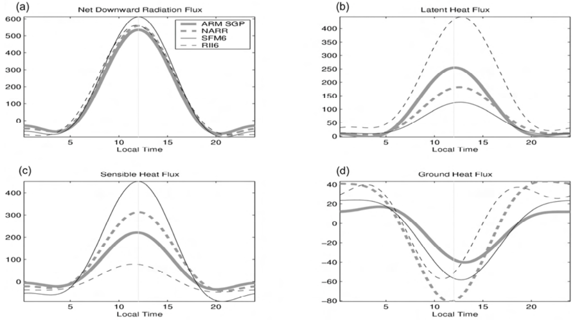
Figure 2.1: The diurnal variation of a) net downward radiation flux, b) latent heat flux, c) sensible heat flux, and d) ground heat flux ( \text{W/m}^2 ) as fitted harmonics from July, August, and September (JAS) 2001-2003 from NARR, SFM6, and RII6, as well as JAS 2003 from the ARM SGP Observations. The light vertical line represents local noon.
