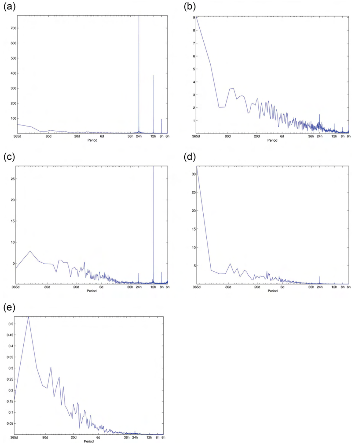
Figure 3.4: Square-root of the average 2002-2004 SFM power spectra at Darwin, Australia, of (a) surface downward shortwave radiation ( \text{W/m}^2 ), (b) precipitation rate (mm/day), (c) 500-hPa geopotential height (m), (d) precipitable water (mm), and (e) soil moisture content from the top 10 cm (cm).
