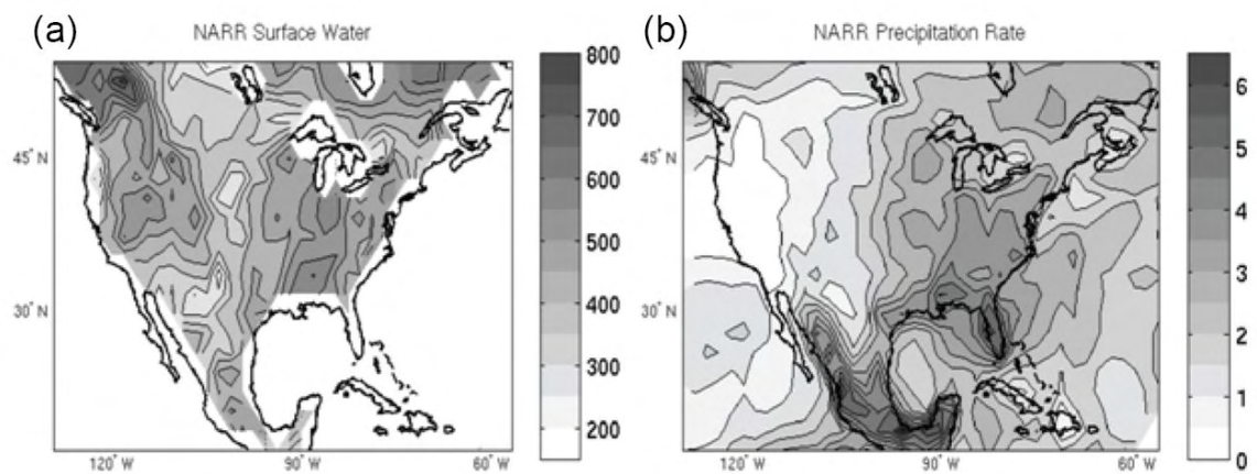
Figure 2.7: NARR July, August, and September 2001-2003 mean (a) surface water (soil water + snow pack, mm) and (b) precipitation rate (mm/day).
