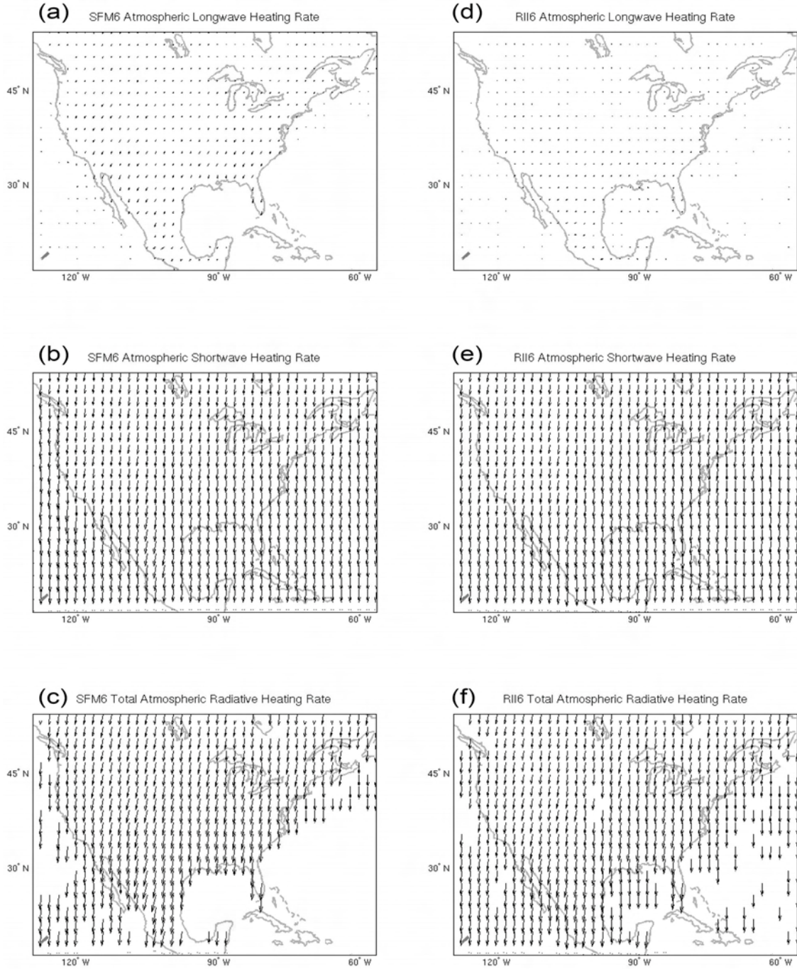
Figure 2.13: As in Fig. 2.5 but for longwave (a and d), shortwave (b and e), and total atmospheric radiative heating rate (c and f), with a reference length of 100 W/m 2 . Only the SFM (a, b, and c) and RII6 (d, e, and f) reanalyses are available.
