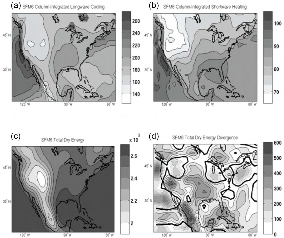
Figure 2.12: SFM6 July, August, and September 2001-2003 mean (a) column-integrated longwave cooling and (b) shortwave heating ( \text{W/m}^2 ), (c) total dry energy ( \text{J/m}^2 ) and (d) total dry energy divergence ( \text{W/m}^2 ). Dashed lines indicate negative contours, and the bold line is the zero contour.
