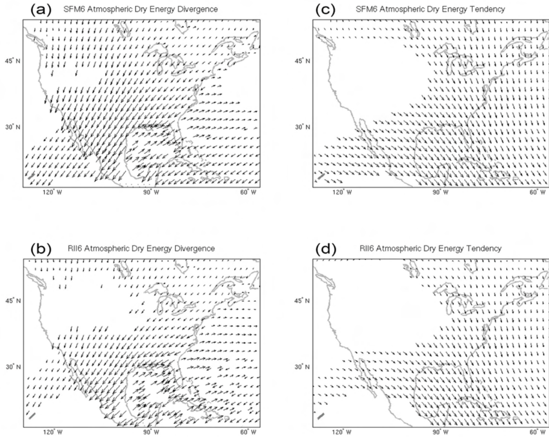
Figure 2.14: As in Fig. 2.5, but for total atmospheric dry energy divergence ( a and b ) and total dry energy tendency ( c and d ), both with a reference length of 500 W/m 2 . Only the SFM ( a and c ) and RII ( b and d ) reanalyses were available.
