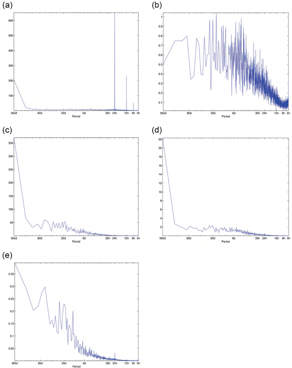
Figure 3.3: Square-root of the average 2002-2004 SFM power spectra at the ARM SGP site, of (a) surface downward shortwave radiation ( \text{W/m}^2 ), (b) precipitation rate ( \text{mm/day} ), (c) 500-hPa geopotential height (m), (d) precipitable water (mm), and (e) soil moisture content from the top 10 cm (cm).
