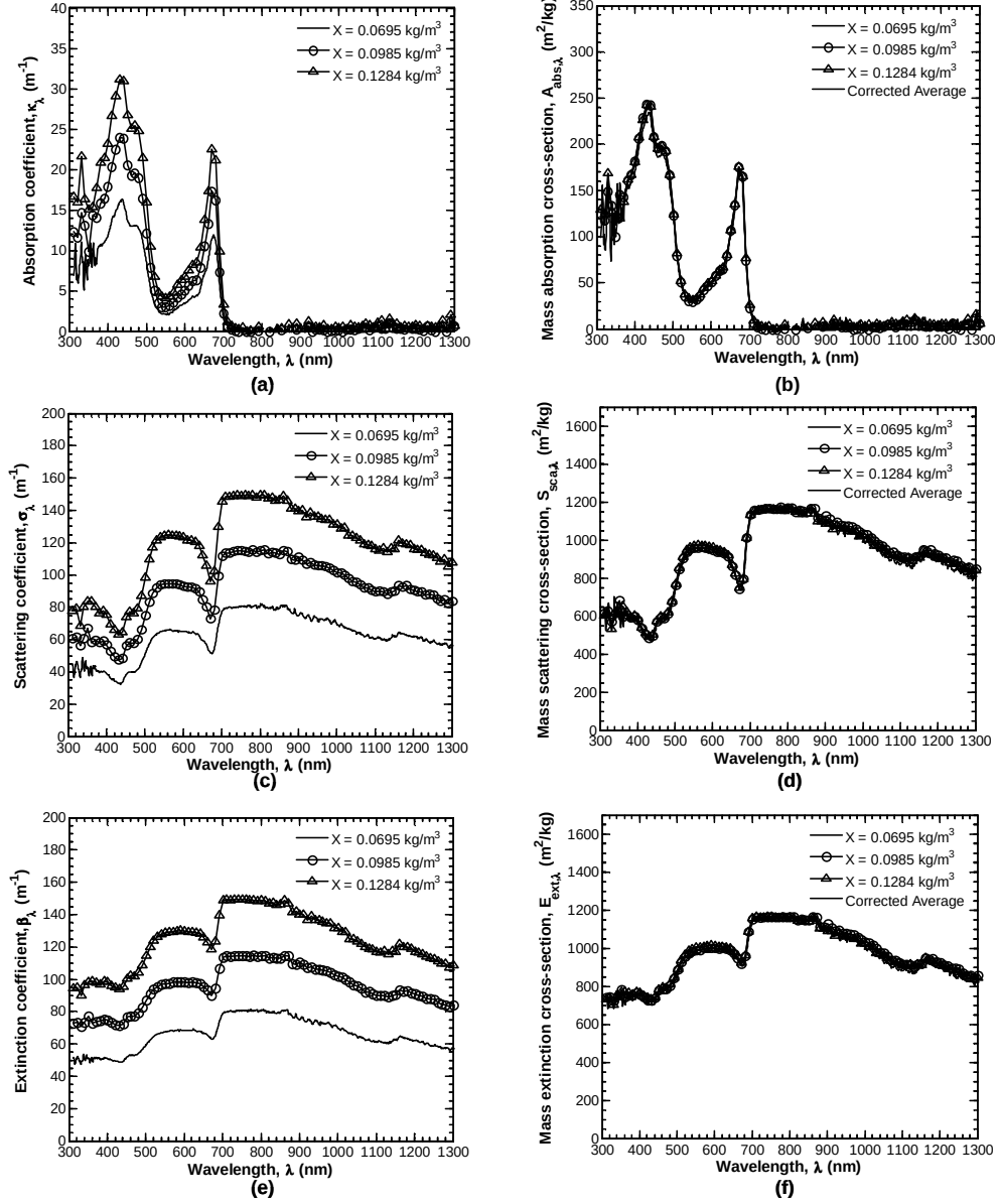
Figure 7: The (a) absorption \kappa_\lambda , (c) scattering \sigma_\lambda , and (e) extinction \beta_\lambda coefficients and the corresponding (b) mass absorption A_{abs,\lambda} , (d) mass scattering S_{sca,\lambda} , and (f) mass extinction E_{ext,\lambda} cross-sections of C.reinhardtii tla1 over the spectral range from 300 to 1,300 nm at three different microorganism concentrations.
