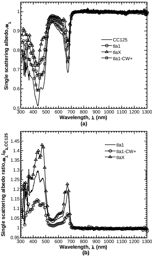
Figure 11: (a) The single scattering albedo \omega_\lambda for all strains and (b) the ratio of the single scattering albedo of tla1 , tlaX , and tla1 -CW + with respect to that of C.reinhardtii CC125 over the spectral range from 300 to 1,300 nm.
