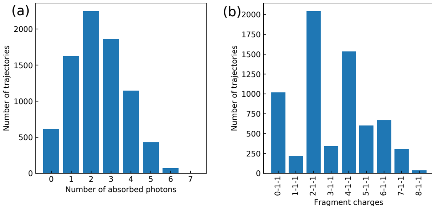
545 FIG. 8. Number of trajectories for H 2 O grouped according to the number of absorbed photons (a) and grouped according to the fragment charges (only three-body fragmentations) (b). The total number of trajectories is 8,000.
