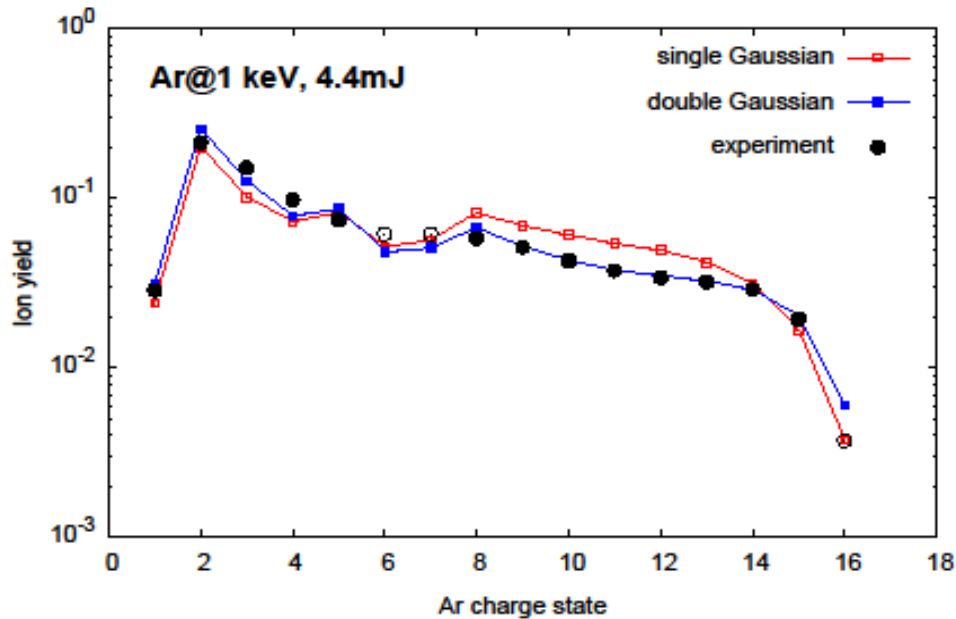
750 Fig 14. Argon calibration measurement. The black circles show measured ion yields (open circles are excluded for calibration), and the lines show ion yields as calculated from atomic simulations. The red line shows results obtained with a single-Gaussian for the spatial fluence distribution, while the blue line shows results obtained with a double-Gaussian fluence distribution. See text for the optimized parameters of the fluence distribution.
