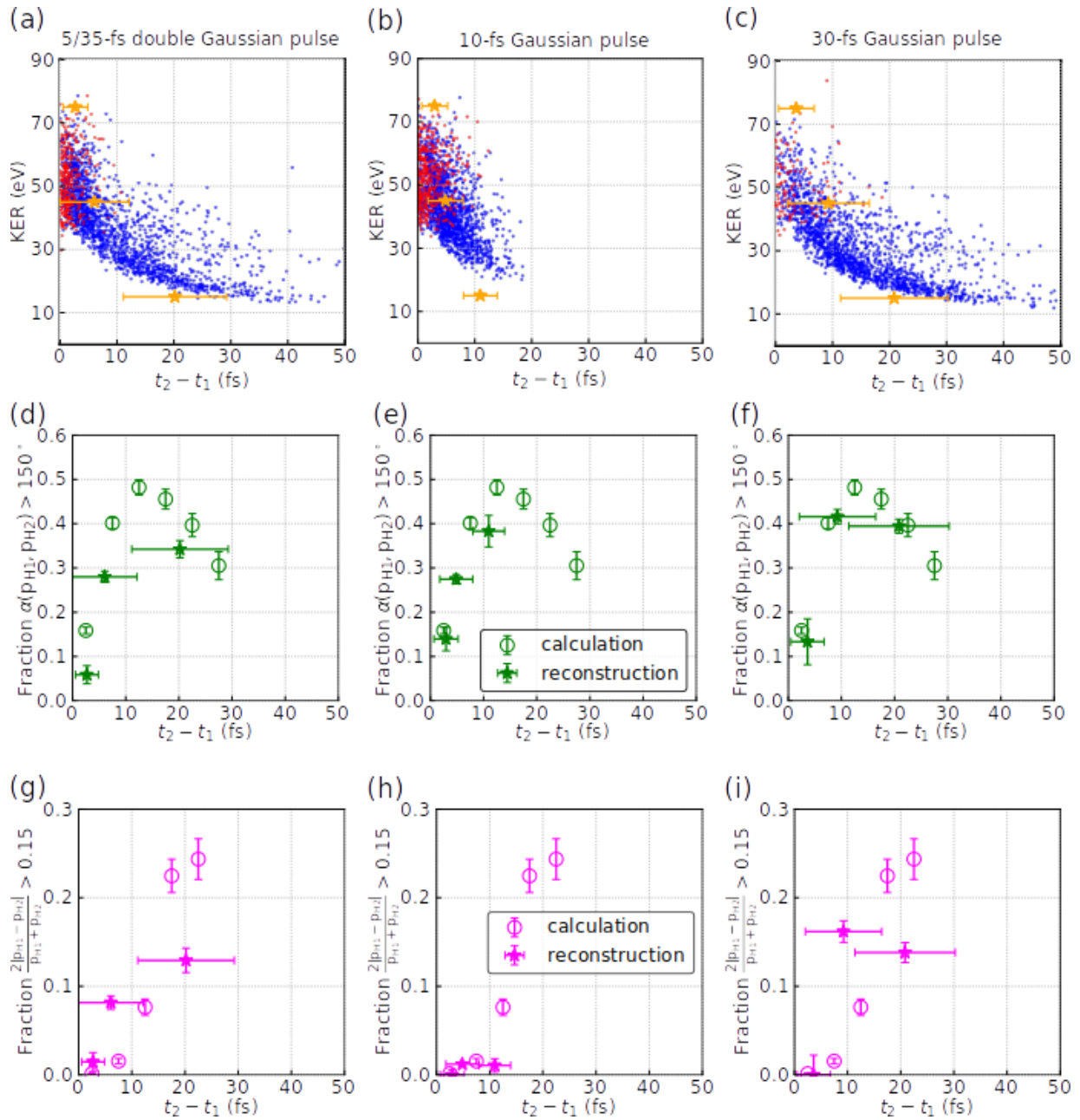
Fig 16. (a), (b), and (c): KER as a function of time between the first and the second photoionization t_2-t_1 for different pulse shapes. The yellow stars mark the average timing values for the selected KER bins. The error bar shows the standard deviation of t_2-t_1 within the bin. (d), (e), and (f): Fraction of proton angles larger than 150^\circ as a function of t_2-t_1 . (g), (h), and (i): Fraction of proton asymmetry larger than 0.15 as a function of t_2-t_1 . The circles show the data as extracted from the simulations, the stars show data, where the timing information has been deduced by the KER–time relation. Vertical error bars indicate standard error, horizontal error bars indicate the standard deviation of t_2-t_1 within the selected KER bin.
