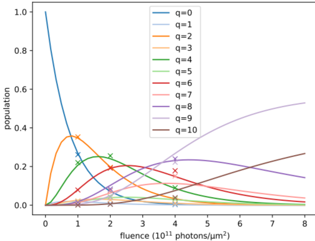
FIG. 7. Population of different charge states q as a function of fluence. The solid lines show results for a fixed-geometry simulation, the crosses show results for a dynamic geometry calculation.
