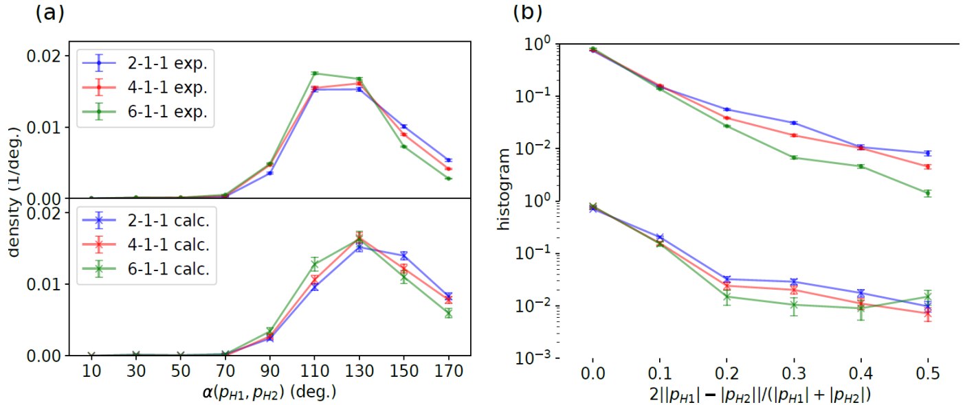
FIG. 6. Distribution of proton momentum angle (a) and proton momentum asymmetry (b) for different charge coincidences (experiment and simulations). The error bars show standard errors due to finite sampling.
