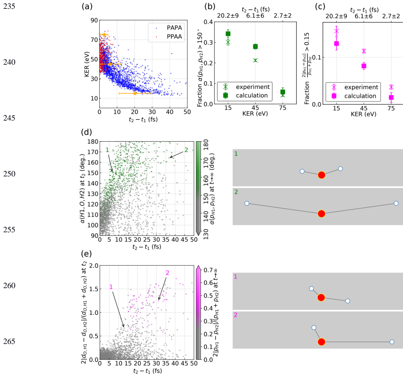
270 FIG. 4. Evolution in time. (a) KER as a function of time between the first and the second photoionization, t_2 - t_1 (simulation). Two different ionization sequences, alternating photoionization and Auger decay (PAPA) and two photoionizations followed by two Auger decays (PPAA), are marked in different colors. The yellow stars mark average delay times for the three KER bins considered in Fig. 1 and Figs. 4(b) and 4(c). The bars indicate standard deviations of the delay times within the respective KER bins. (b), (c): Fraction of coincidence events with large proton-proton momentum angle and large relative proton momentum asymmetry as a function of KER (experiment and simulation). (d), (e): HOH bond angles and asymmetry ratio of the OH distances at the point in time of the second photoabsorption vs. time delay with respect to the first photoabsorption (simulations) accompanied by selected snapshots of the molecular geometry. All plots are for coincidences with oxygen charge 2+ and 2H+ ions. 275 280
