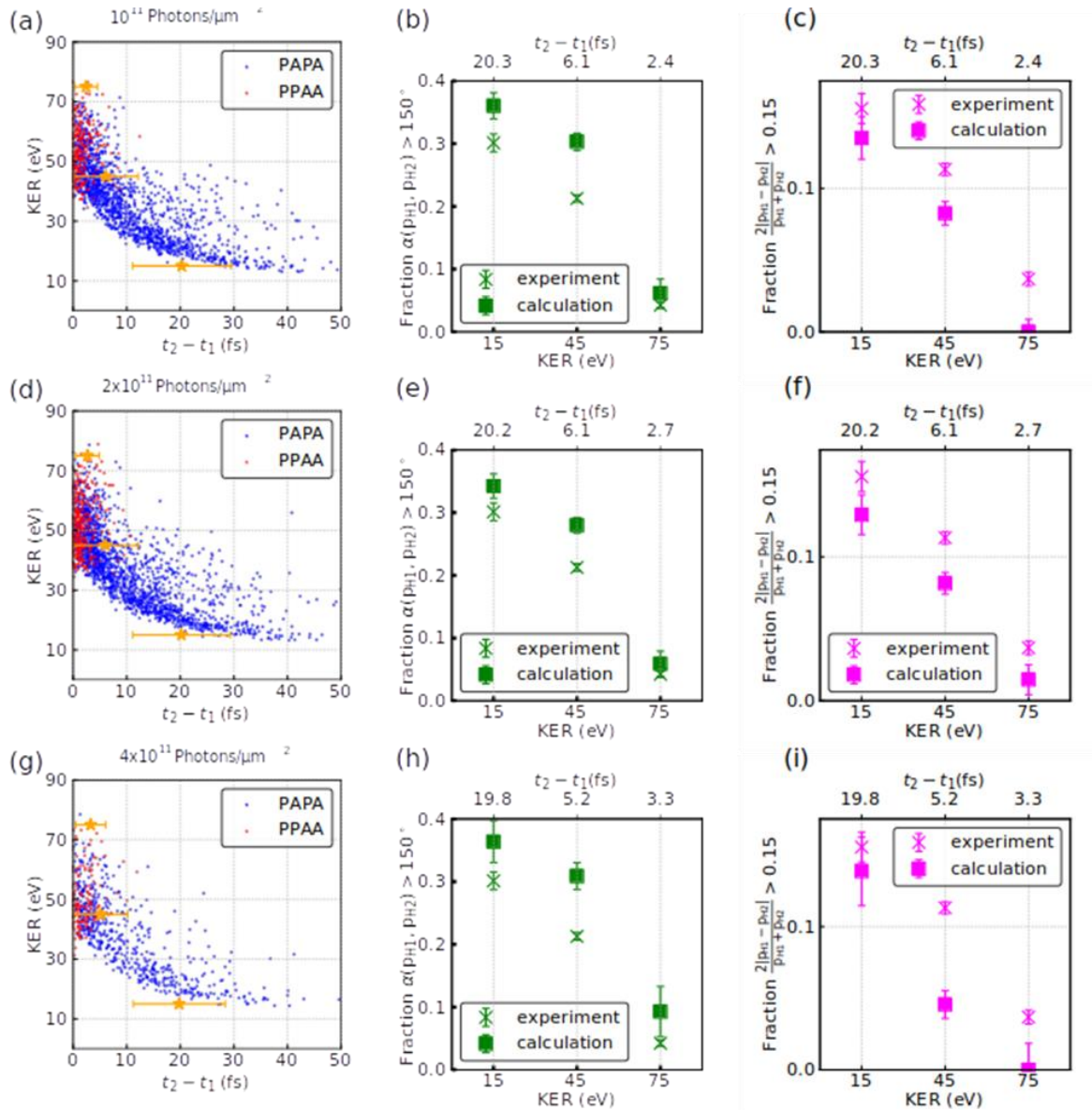
810 Fig 15. Evolution in real time [same as Fig. 4 (a), (b), (c) but for different fluences]. (a), (d), (g) KER as a function of time between the first and the second photoionization, t_2 - t_1 (simulation) for different fluence values. The yellow stars mark average delay times for the three KER bins considered in Figs. (b), (e), (h) and (c), (f), (i). The bars indicate standard deviations of the delay times within the respective KER bins. (b), (e), (h): Ratio of coincidence events with large proton-proton momentum angle and large relative proton momentum asymmetry as a function of KER (experiment and simulation). (c), (f), (i): HOH bond angles and asymmetry ratio of the OH distances at the point in time of the second photoabsorption vs. time delay with respect to the first photoabsorption (simulations) accompanied by selected snapshots of the molecular geometry. All plots are for coincidences with oxygen charge 2+ and 2H^+ ions. The calculated results are obtained for different fluence values (a), (b), (c): 10^{11} ph./ \mu\text{m}^2 , (d), (e), (f): 2 \times 10^{11} ph./ \mu\text{m}^2 , (g), (h), (i): 4 \times 10^{11} ph./ \mu\text{m}^2 815 820
