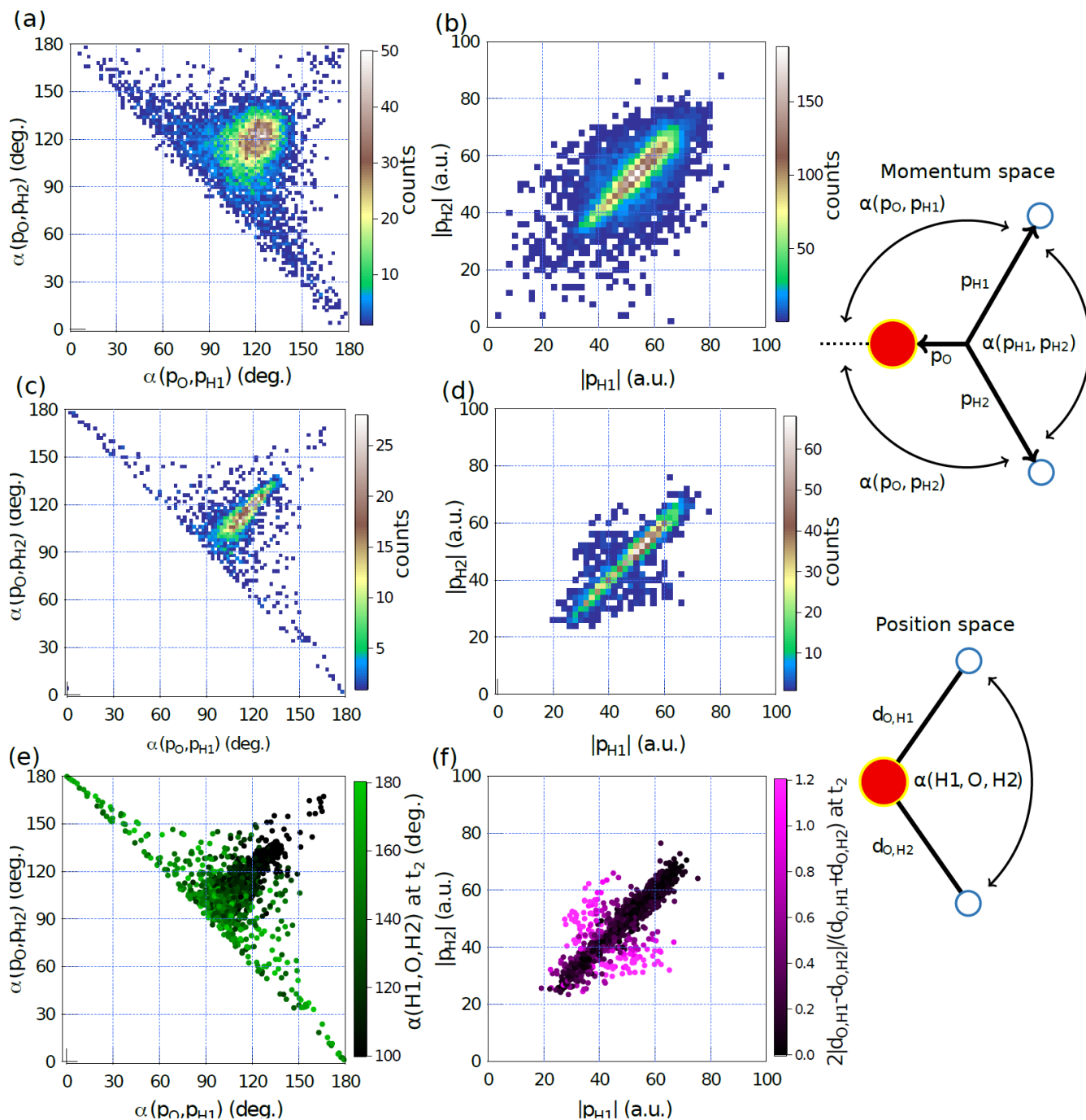
FIG. 3. Scatter plots. (a), (c): Scatter plots showing the angles of the final proton momenta with respect to the final oxygen momentum (experiment and simulation); (e): scatter plot of proton angles (simulation), where large HOH bond angle at the time of the second photoionization is indicated by green color; (b), (d): Scatter plots showing the magnitudes of the final proton momenta (experiment and simulation); (f): scatter plot showing final proton momenta (simulation), where structural asymmetry at the time of the second photoionization is indicated by pink color. The relevant momentum- and real- space coordinates are also shown.
