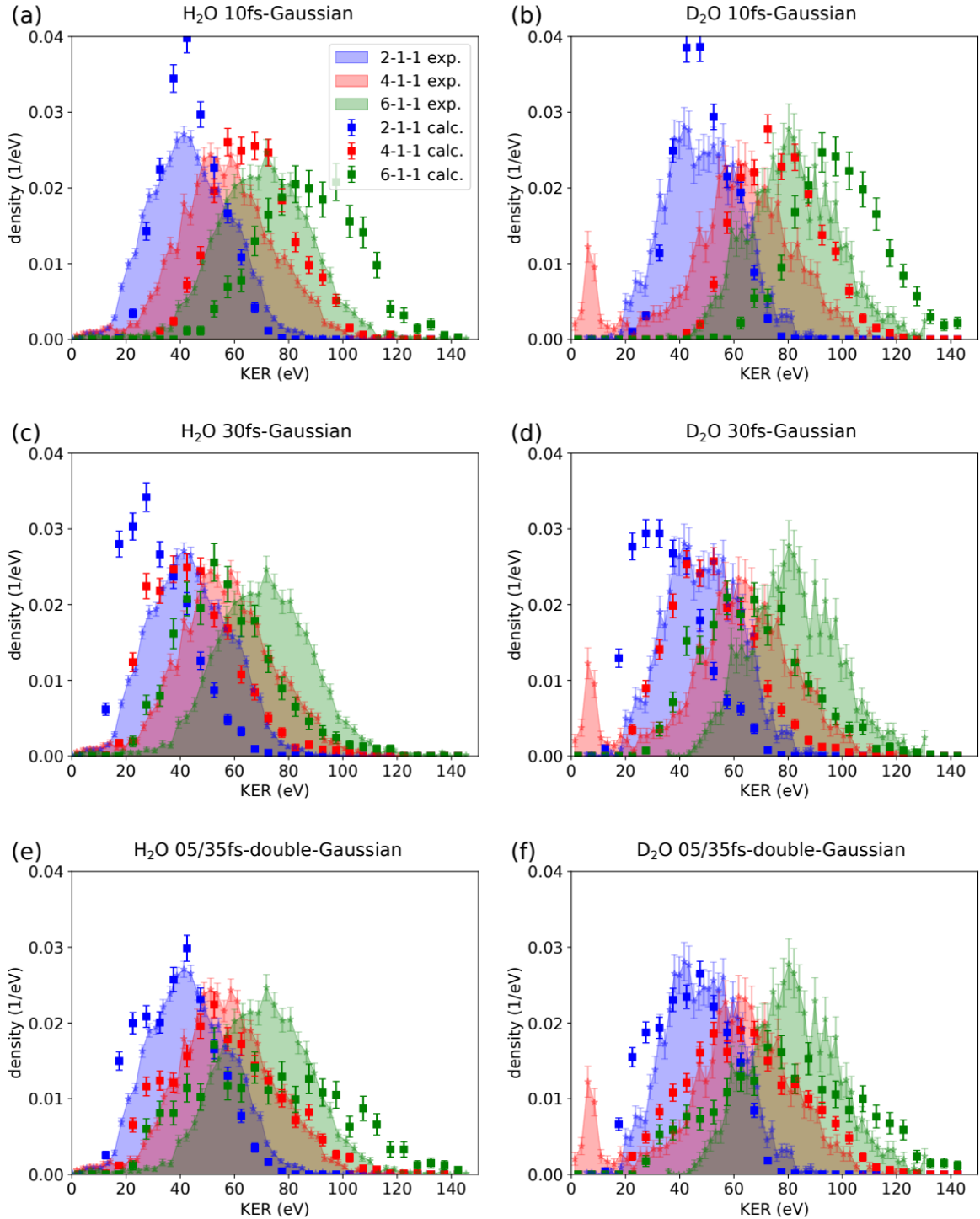
FIG. 9. Total kinetic energy release for H 2 O and D 2 O for different coincidence channels and for different temporal pulse shapes. x-1-1 labels coincidence channels with final oxygen fragment charge +x and hydrogen charges +1. The squares show data from the simulation, the asterisks and the shaded areas show data from the experiment. The error bars show standard errors due to finite sampling. Note that the peak at 10 eV for D 2 O in the experimental data is an artifact caused by He + .
