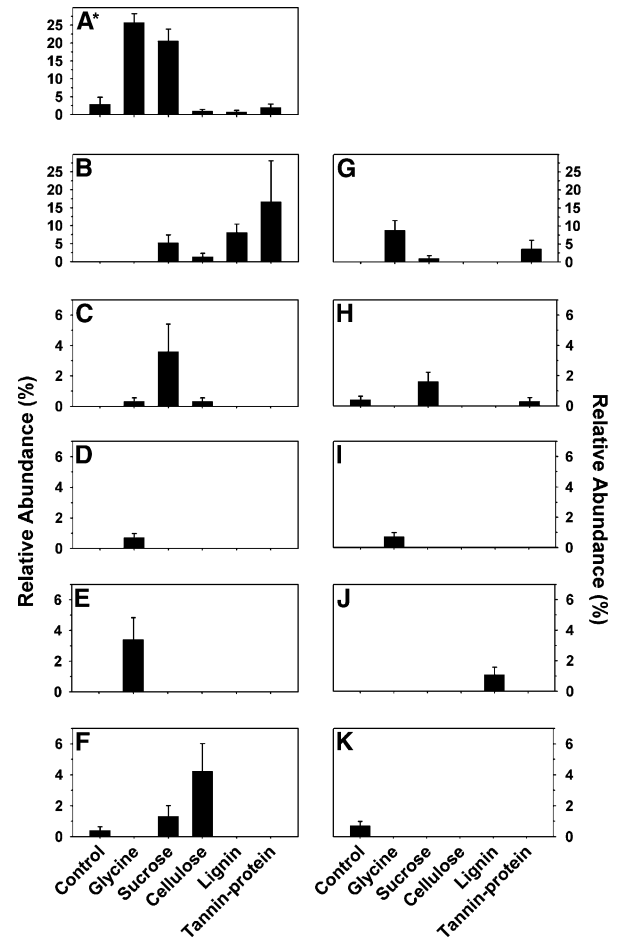
Figure 2. Relative abundances (% of sequences within a treatment) of active fungal OTUs showing at least a marginally significant change in relative abundance ( P < 0.10 , except * = P < 0.05 , Kruskal–Wallis tests) among substrate additions. In total, only 11 OTUs exhibited significant or marginally significant changes. (A) Zygomycete (Mortierellaceae), OTU 5. (B) Zygomycete ( Mortierella ), OTU 18. (C) Zygomycete (Mortierellaceae), OTU 13. (D) Zygomycete (Mortierellales), OTU 17. (E) Zygomycete ( Umbelopsis ), OTU 42. (F) Unknown fungus, OTU 25. (G) Unknown fungus, OTU 8. (H) Unknown fungus, OTU 52. (I) Unknown fungus, OTU 120. (J) Basidiomycete (Agaricales), OTU 47. (K) Basidiomycete ( Lactarius ), OTU 77. OTUs were determined by analysis of sequences at the 97% or greater similarity level. Bars represent s.e.m., n = 4 .
