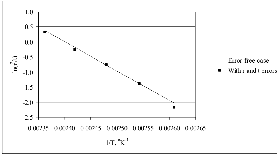
Figure 7. Illustration of a log-Arrhenius plot for laboratory induced hydration. The slope = -E/R , and the y-intercept = \ln(k_0) .
