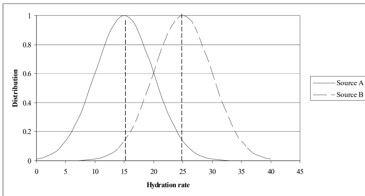
Figure 3. Hydration rate distributions for two geochemical sources. Spread is caused by intra-source variations in intrinsic water content. Geochemical sourcing controls for central tendency (dashed lines), while spread contributes of uncertainty in computed age.
