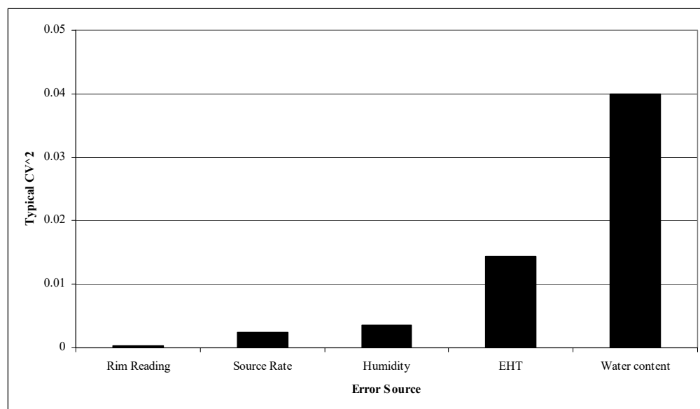
Figure 8. Typical relative magnitudes of error sources in OHD. Note that intrinsic water variation and temperature history (EHT uncertainty) are the major contributors.
