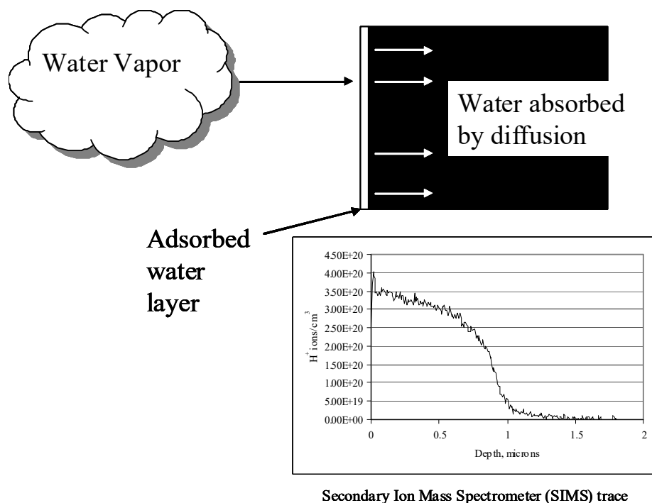
Figure 1. Schematic view of obsidian hydration. Water molecules in the atmosphere are adsorbed on the surface, and diffuse into the glass. The plot shows hydrogen ion concentration (a proxy for water) as a function of depth in the glass (SIMS trace courtesy of C. M. Stevenson). As time progresses, the curve shifts to the right.
