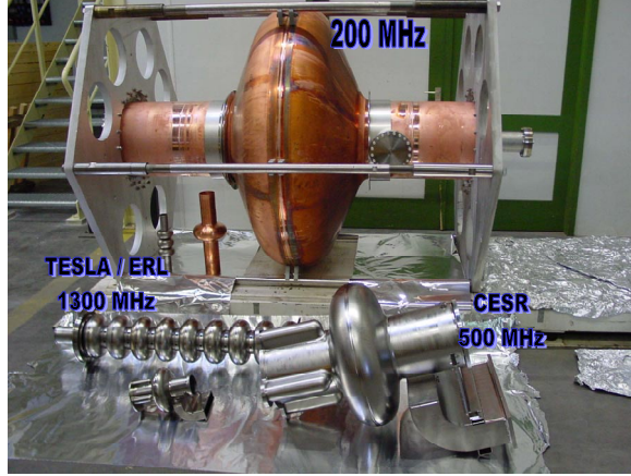
Figure 7. Photograph of 200 MHz SCRF cavity at Cornell, with its smaller siblings.
