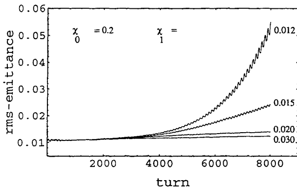
FIG. 2. Multi-particle simulation result showing stabilization of the HT motions of the rms-emittance of a Gaussian beam when \chi_1 \geq 0.026 – the theoretical stability threshold of the l = 1 mode [cf. Eq. (11)]. Here \chi_0 = 0.2 , \Upsilon = 0.22 .
