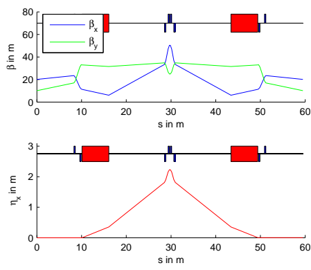
Figure 3: Twiss parameters of the double bend achromat.
