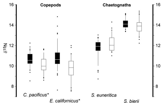
Fig. 1. Average \delta^{15}\text{N} of four zooplankton species (copepods Calanus pacificus and Eucalanus californicus , and chaetognaths Sagitta euneritica and Sagitta bierii ) in two regions of the California Current System (Southern California=solid, Central California=open). Box boundaries indicate the 25th and 75th percentiles of the distribution of values, horizontal line indicates the median, whiskers the 10th and 90th percentiles, and dots the outliers. Asterisks indicate significant differences between regions ( p < 0.05 , Mann–Whitney U ).
