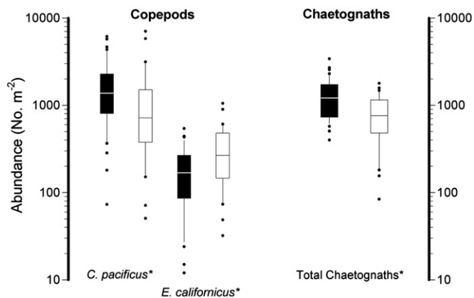
Fig. 3. Average abundance of two copepod species and total chaetognaths in two regions of the California Current System (Southern California=solid, Central California=open). Asterisks indicate significant differences between regions ( p < 0.05 , Mann–Whitney U ). Others details as in Fig. 1.
