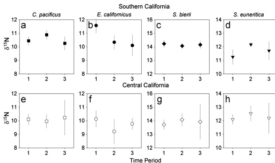
Fig. 6. Decadal variation in zooplankton \delta^{15}\text{N} across three time periods (1 = 1951–1976, 2 = 1977–1998, 3 = 1999–2004) in Southern California (a–d) and Central California (e–h) waters. (a,e) Calanus pacificus , (b,f) Eucalanus californicus , (c,g) Sagitta bierii , and (d,h) Sagitta euneritica . Mean \pm 95% C.I.
