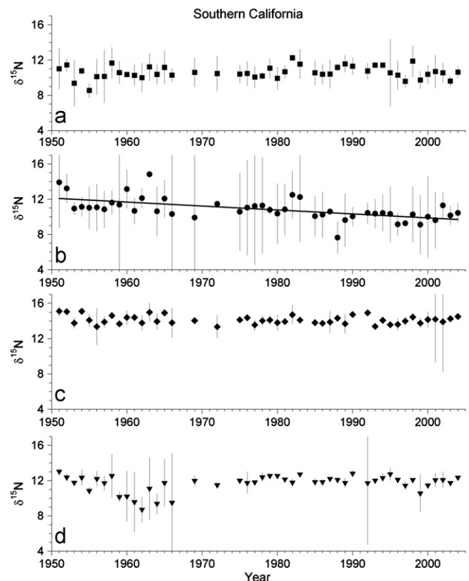
Fig. 4. Long-term variation in \delta^{15}\text{N} of four zooplankton species in Southern California waters, and p -value of a test of departure of the slope of a linear trend from zero, together with r^2 . (a) Calanus pacificus ( p > 0.10 , r^2=0.02 ), (b) Eucalanus californicus ( p < 0.001 , r^2=0.35 , solid regression line), (c) Sagitta bierii ( p > 0.10 , r^2=0.04 ), and (d) Sagitta euneritica ( p > 0.05 , r^2=0.08 ). Sample size was 46 for all regressions. Mean \pm 95% C.I.
