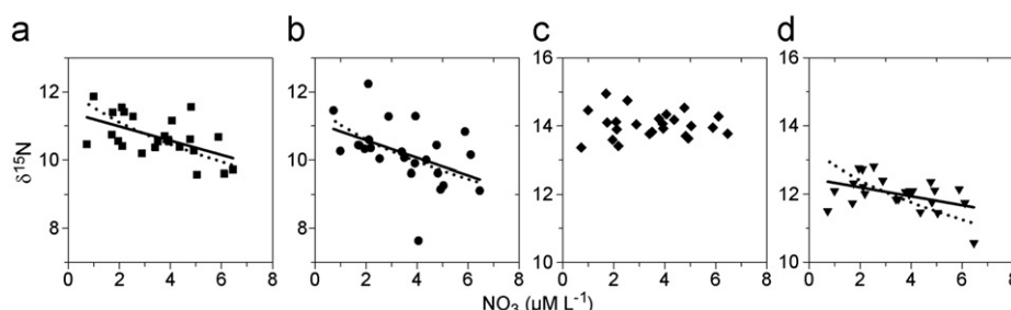
Fig. 8. Relationship between zooplankton \delta^{15}\text{N} and average nitrate concentration (10–50 m) in Southern California waters. (a) Calanus pacificus , (b) Eucalanus californicus , (c) Sagitta bierii , and (d) Sagitta euneritica . Solid lines indicate regressions significant at p < 0.05 (slope differs from 0). Dotted lines denote Rayleigh model fits where initial source [\text{NO}_3^-] = 25 \mu\text{M L}^{-1} (Liu and Kaplan, 1989; Sigman et al., 2005), source nitrate \delta^{15}\text{N} = 8\text{‰} (Liu and Kaplan, 1989; Sigman et al., 2005), instantaneous isotope fractionation by phytoplankton nitrate uptake = 5‰ (Waser et al., 1998; Altabet et al., 1999), phytoplankton \delta^{15}\text{N} = \delta^{15}\text{N} of the accumulated biomass product predicted by the model, and in each species zooplankton \delta^{15}\text{N} is trophically elevated above predicted phytoplankton \delta^{15}\text{N} by a specified constant amount: C.p. +4.2%, E.c. +3.7%, and S.e. +5.5‰.
