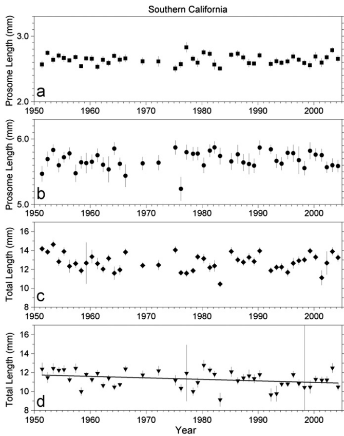
Fig. 5. Long-term variation in body length of four zooplankton species in Southern California waters, and p -value of a test of departure of the slope of a linear trend from zero, together with r^2 . Prosome length of the copepods, (a) Calanus pacificus ( p > 0.10 , r^2 = 0.01 ), and (b) Eucalanus californicus ( p > 0.10 , r^2 = 0.02 ), and total length of the chaetognaths, (c) Sagitta bierii ( p > 0.10 , r^2 = 0.01 ), and (d) Sagitta euneritica ( p < 0.05 , r^2 = 0.09 , solid regression line). Sample size was 46 for all regressions. Mean \pm 95% C.I.
