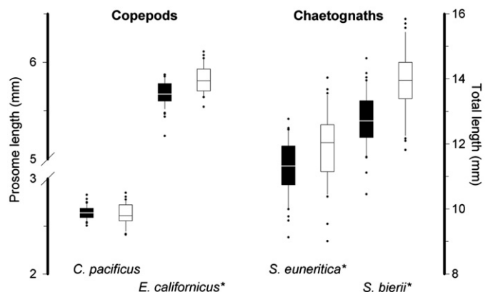
Fig. 2. Average body length of four zooplankton species in two regions of the California Current System (Southern California=solid, Central California=open). Prosome length of the copepods, (a) Calanus pacificus , and (b) Eucalanus californicus , and total length of the chaetognaths, (c) Sagitta bierii , and (d) Sagitta euneritica . Asterisks indicate significant differences between regions ( p < 0.05 , Mann–Whitney U ). Others details as in Fig. 1.
