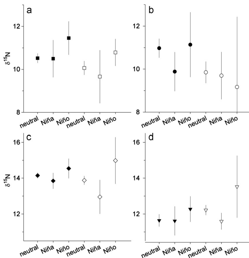
Fig. 7. Interannual variation in zooplankton \delta^{15}\text{N} in three phases of ENSO: neutral =El Niño-neutral years, Niña =La Niña years, Niño =strong El Niño years (Southern California=solid, Central California=open). (a) Calanus pacificus , (b) Eucalanus californicus , (c) Sagitta bierii , and (d) Sagitta euneritica . Mean \pm 95% C.I.
