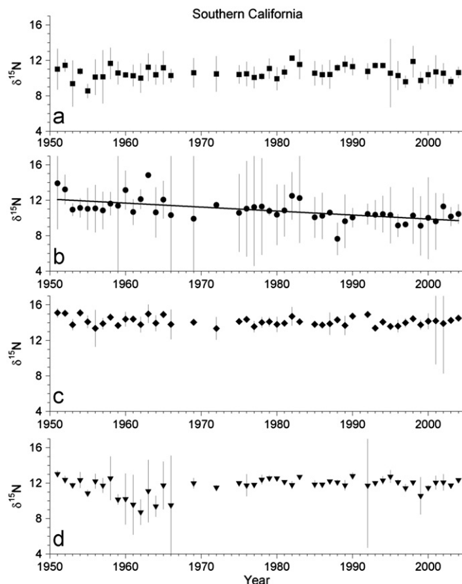
Fig. 4. Long-term variation in \delta^{15}\text{N} of four zooplankton species in Southern California waters, and p -value of a test of departure of the slope of a linear trend from zero, together with r^2 . (a) Calanus pacificus ( p > 0.10 , r^2=0.02 ), (b) Eucalanus californicus ( p < 0.001 , r^2=0.35 , solid regression line), (c) Sagitta bierii ( p > 0.10 , r^2=0.04 ), and (d) Sagitta euneritica ( p > 0.05 , r^2=0.08 ). Sample size was 46 for all regressions. Mean \pm 95% C.I.
