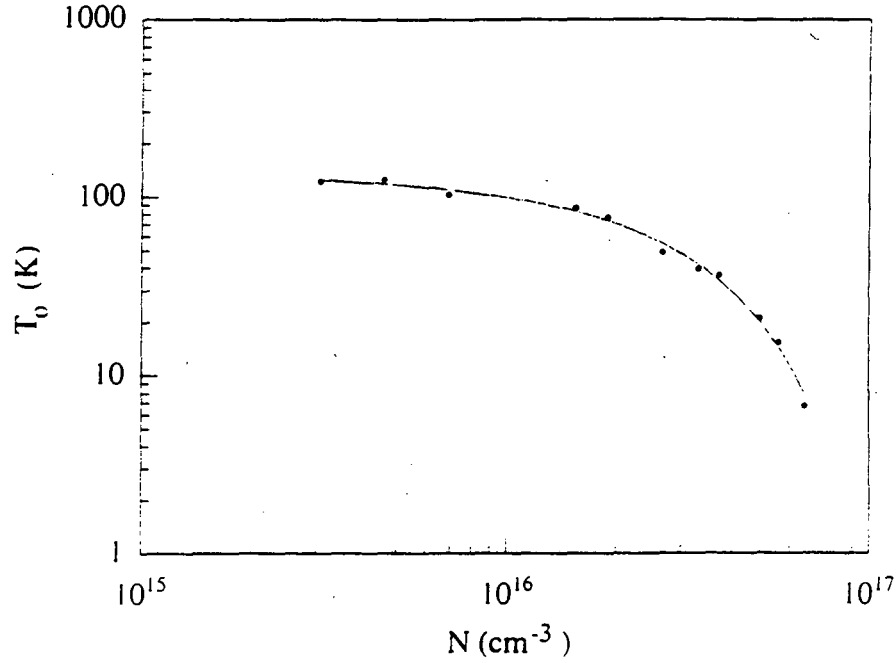
Fig. 3.8 Measured dependence of the variable range hopping parameter T_0 on impurity concentration N for the NTD ^{\text{nat}}\text{Ge}:\text{Ga} samples studied in Experiment 1.
