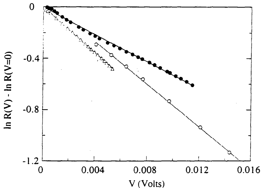
Fig. 5.2 Measurements of the electrical nonlinearities in neutron transmutation doped germanium. The curves are very well fit by a straight line, in agreement with Equation 5.1. Similar curves have been measured for a wide range of temperatures, from which we deduce a length parameter L = 450/T^{0.5} \text{ \AA} for all three samples. The curves represent NTD-19 at T = 96 \text{ mK} (open triangles), NTD-6 at T = 101 \text{ mK} (open circles), and NTD-17 at T = 113 \text{ mK} (closed circles).
