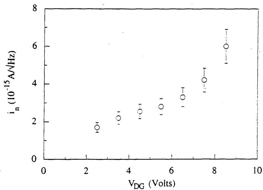
Fig.A.6 Room temperature current noise of the NJ132L JFET as a function of drain-gate voltage.
