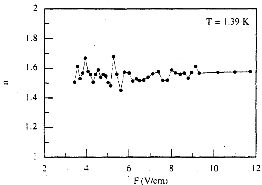
Fig. 3.29 Exponent x from Equation 3.11 as a function of electric field. The data are described by x \approx 1.54 over the entire range of fields.
