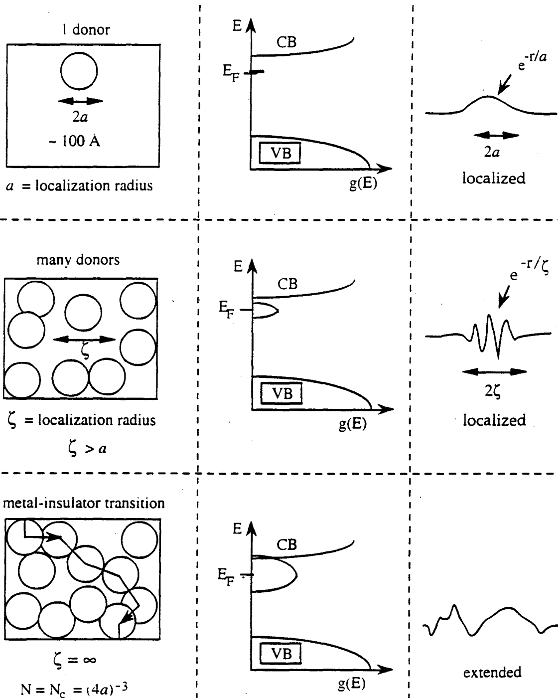
Fig.1.3 As the impurity concentration increases, the doped semiconductor undergoes a metal-insulator transition corresponding to the transition between extended and localized states at the Fermi level.
