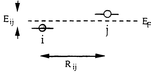
Fig. 1.7 An occupied impurity site i and an unoccupied impurity site j , separated by a distance R_{ij} and by energy E_{ij} .
