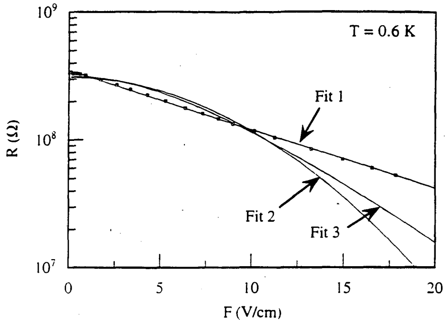
Fig. 3.10 Electric field dependence of the resistance of \text{natGe:Ga} with an impurity concentration N \approx 0.046N_c . The three fits are described in the text.
