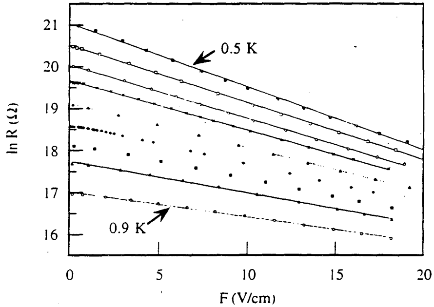
Fig. 3.9 Electric field dependence of the resistance of a lightly doped ^{\text{nat}}\text{Ge}:\text{Ga} sample with an impurity concentration N \approx 0.046N_c . Curves were measured at temperatures between 0.5 K and 0.9 K, with successive curves separated by 0.05 K.
