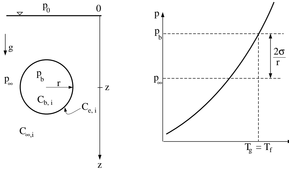
Figure 2: Schematic of a single bubble in thermal equilibrium with the glassmelt and the corresponding p-T diagram.
