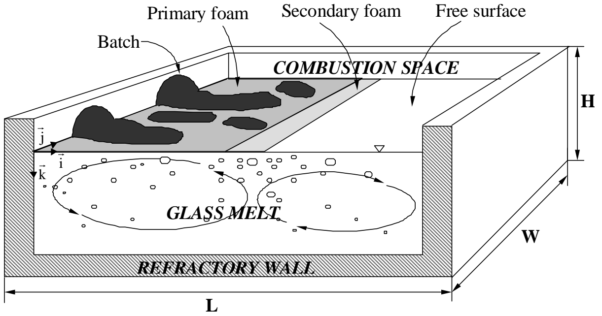
Figure 1: Schematic of a glass melting furnace and the coordinate system.
