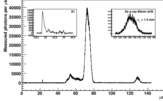
Figure 4: Typical full energy 662 keV gamma ray event waveform: the sum of the previously calibrated waveforms of the 19 photomultipliers is shown. The S1 pulse (shown in detail in the left inset) due to xenon scintillation is short and with O(200) measured photons. Two S2 pulses caused by electroluminescence of xenon from ionization electrons follow. The first with \sim 270,000 measured photons is likely due to a 630 keV electron from the photoelectric interaction of the 662 keV gamma ray; the pulse structure reflects the ionization density of the track along its \sim 2.5 cm long projection on the drift ( z ) direction. The second (shown in detail in the right inset) with \sim 12,000 measured photons is likely due to the interaction, a few cm away, of a 30 keV xenon X-ray following the photoelectric process; since the 30 keV energy deposition is nearly point-like the pulse shape is gaussian with a \sigma_L of 1.4 mm set by the longitudinal diffusion of the electrons during the \sim 8 cm drift. This event is from a data run taken at 10 atm with a 0.16 kV/cm drift electric field and an E/P of 2.1 kV/(cm atm) in the EL region.
