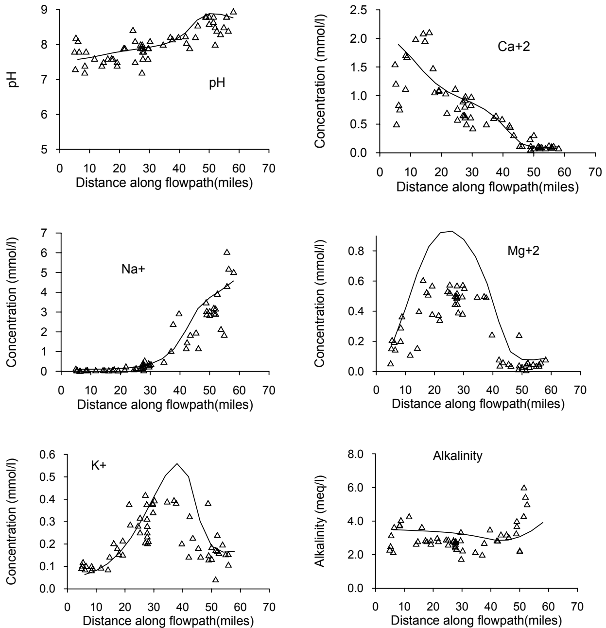
Figure 8.2.4. Concentrations of Na + , K + , Mg 2+ , Ca 2+ , alkalinity, and pH along a flow path in the Aquia aquifer (Maryland). Symbols indicate observations provided by Appelo (1994) and originally from Chapelle and Knobel (1983); solid lines represent simulated concentrations using TOUGHREACT.
