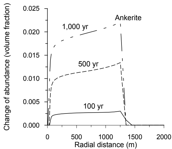
(a) Ankerite
