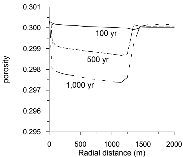
(b) Porosity
