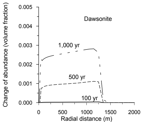
(b) Dawsonite
