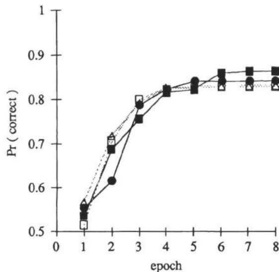
Figure 7: Best fit of standard back propagation to human learning data in Figure 5.
