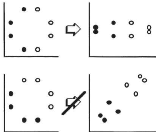
Figure 2: Top panel shows that increasing attention to the horizontal dimension and decreasing attention to the vertical dimension causes exemplars of the two categories (denoted by filled and open circles) to have greater between-category dissimilarity and greater within-category similarity (after Nosofsky 1986, Fig. 2). Lower panel shows that ALCOVE cannot differentially attend to diagonal axes.
