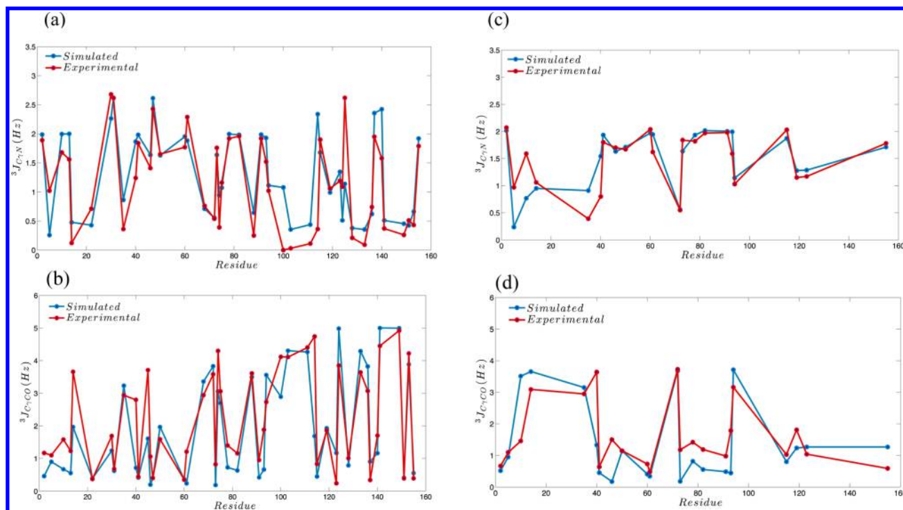
Figure 4. J -coupling constants: (a) {}^3J_{C7N} and (b) {}^3J_{C7CO} for the DHFR binary product complex E:THEF, and (c) {}^3J_{C7N} and (d) {}^3J_{C7CO} for the DHFR binary product complex E:FOL. The red symbols are the experimental data from ref 167. The blue symbols are calculated from the MC-SCE ensemble using backbones from molecular dynamics and the Karplus parametrization from ref 167. Reprinted with permission from ref 61. Copyright 2015 Elsevier.
