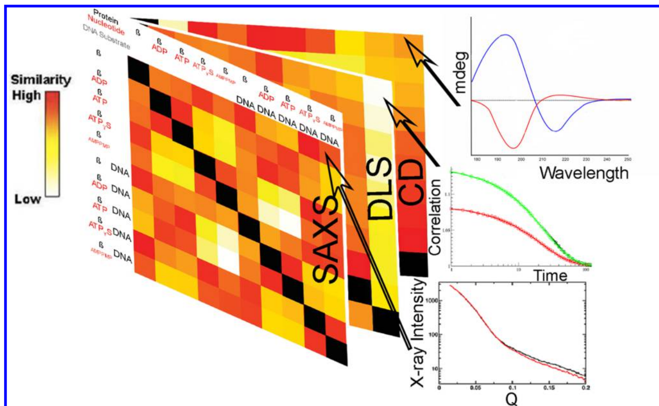
Figure 1. Heat map comparing pairs of profiles from multiple experimental techniques including SAXS, DLS, and CD. Each cell is a pairwise comparison between a condition or construct. Similarity between SAXS curves is measured by the metric V_r and displayed as a gradient color, where red indicates similarity (low V_r score) and white indicates dissimilarity. The black square diagonals are self-comparisons. Adapted with permission from ref 79. Copyright 2016 Nature Publishing Group.
