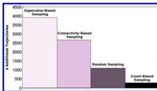
Figure 3. Convergence time for Fs (capped 21 alanine) peptide transition matrix generated with various hybrid sampling schemes. Time is measured in the number of eigenvalue-based trajectories needed to converge to an absolute error of 2.00 after 1000 initial trajectories are run from a chosen sampling method. Absolute error is defined as the sum of absolute deviations in transition matrix elements. Convergence times for each method were, averaged over 10 simulations, (1) 3913 for pure eigenvalue-based sampling, (2) 2669 for connectivity-based hybrid sampling, (3) 1107 for even sampling hybrid sampling, and (4) 286 for min count-based hybrid sampling. Reprinted with permission from ref 154. Copyright 2011 American Chemical Society.
