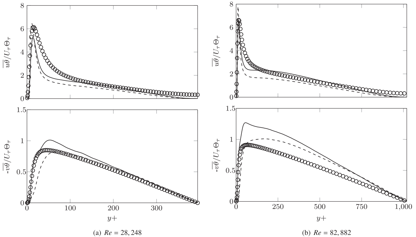
Fig. 4. Heated channel flow: A-priori results of turbulent heat fluxes: — present model, -- model by [8], ○ Abe et al. [11].
