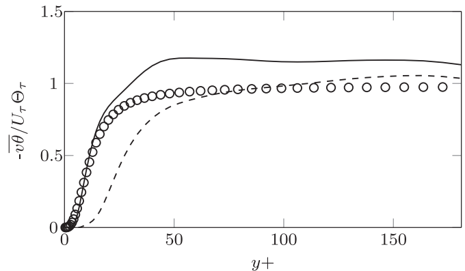
Fig. 2. Heated Couette flow: A-priori results of turbulent heat fluxes at Re_w = 25,600 : — present model, -- model by [8], \circ Tsukahara et al. [13].
