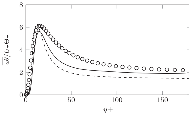
Fig. 2. Heated Couette flow: A-priori results of turbulent heat fluxes at Re_w = 25,600 : — present model, -- model by [8], \circ Tsukahara et al. [13].
