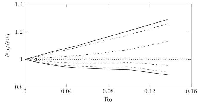
Fig. 12. Spanwise rotating channel: Nusselt number as function of rotation number at Re = 21,522 . The turbulence field is calculated using the DY model: — present model, -- model by [8], - - - Fourier's law.
