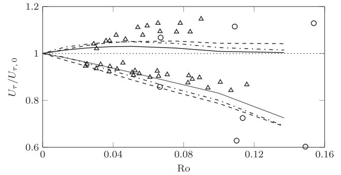
Fig. 11. Spanwise rotating channel: Wall friction velocity as function of rotation number at Re = 21,522 : — DY, -- LRR-IP, - - - SSG, \circ Johnston et al. [3] 23,400 < Re < 36,000 , \Delta Johnston et al. [3] Re = 11,400 .
