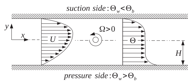
Fig. 8. Spanwise rotating channel flow.
