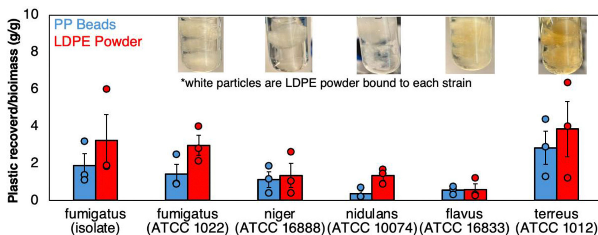
Figure 3: Plastics flocculation is conserved across Aspergilli
