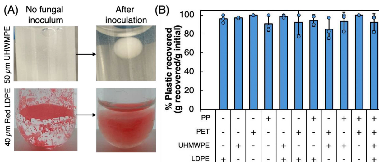
Figure 1: Novel fungal isolate ubiquitously capture microplastics from solution.
