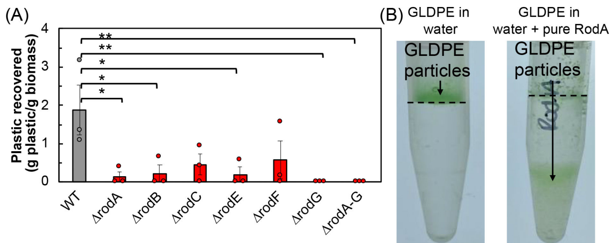
Figure 5: Hydrophobins are responsible for microplastics flocculation by AF-UD1.
