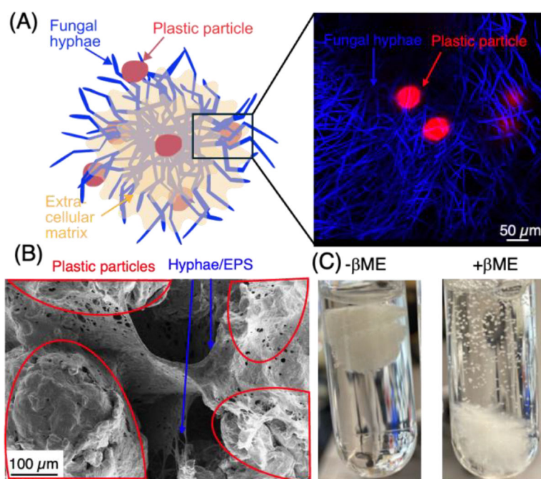
Figure 4: Hydrophobins drive microplastics flocculation in Aspergilli .
