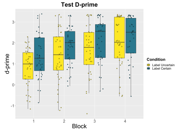
Figure 6: Test d' by block and condition.
