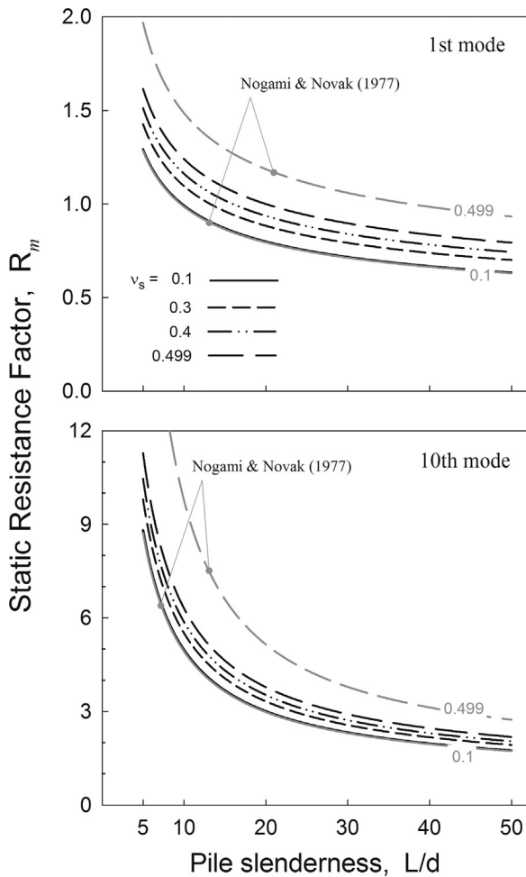
Fig. 7. Effect of Poisson's ratio on static soil resistance factor.
