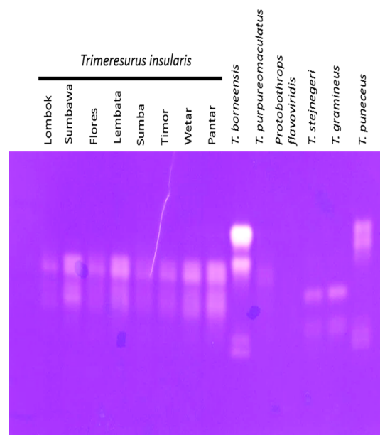
Figure 10. Venoms from each T. insularis population and from the representative Trimeresurus species were analyzed by gelatin zymography. All T. insularis venoms exhibited identical banding patterns, although digestion intensities appear to vary between several populations. Species in the Trimeresurus complex appear to have drastically different gelatinolytic compared to T. insularis . Trimeresurus purpureomaculatus showed weak gelatinolytic activity similar to T. insularis , and P. flavoviridis had no apparent activity.
