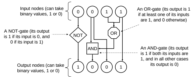
Figure 1: Illustration of a Boolean circuit. In our formalization of RD, the binary string on the input nodes represents an encoding of object a and the binary string on the output nodes represents an encoding of object b .
