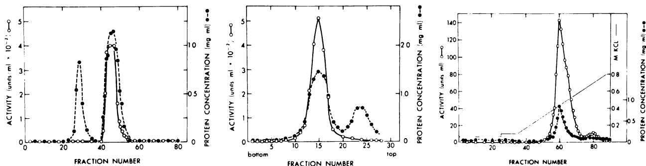
FIG. 1 (left). DEAE-Sephadex column chromatography of yeast RNA polymerase I. Fraction 3 was concentrated by ammonium sulfate precipitation and loaded onto a column (4 × 30 cm) of DEAE-Sephadex A-25 previously equilibrated as described in the text. Eighty fractions of 4.2 ml each were collected and assayed for protein and RNA polymerase activity.
