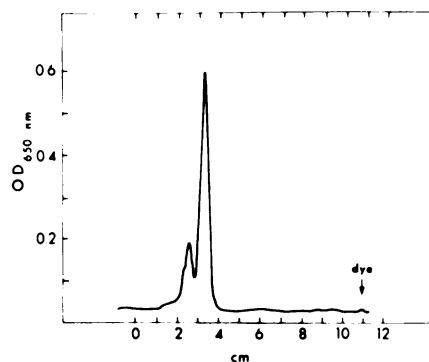
FIG. 4. Polyacrylamide gel electrophoresis of yeast RNA polymerase I under nondenaturing conditions. A sample of 10 \mu g of purified enzyme was subjected to electrophoresis on a 5% acrylamide slab gel as described under "Experimental Procedures."
