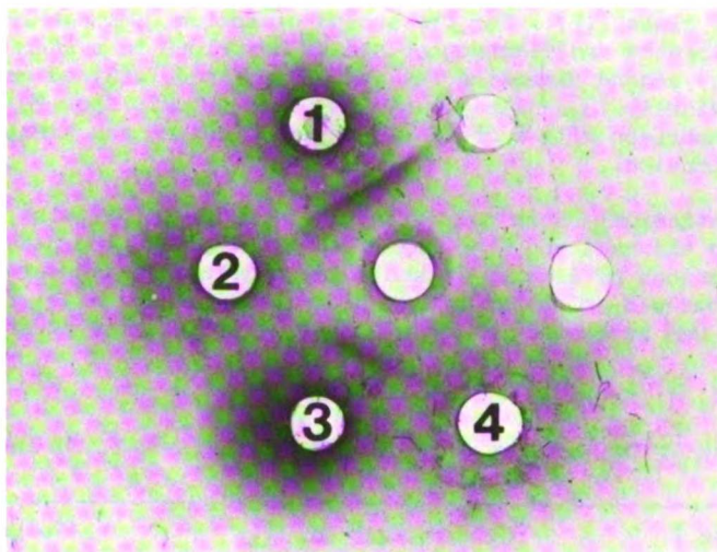
Figure 1. Double diffusion in agar. Immunodiffusion against rabbit antiserum was done at 4°C in 0.6% agar in 0.05 M sodium barbital, pH 8.2 and 0.2% sodium azide. The center well contained 5 \mu l of anti-polymerase I antiserum. Antigen wells contained: 1.5 \mu g of polymerase I (1); 2.5 \mu g of polymerase II (2); 3.5 \mu g of polymerase III (3); 4.2 \mu g of E. coli RNA polymerase (4). After formation of precipitin lines, the immunodiffusion plates were washed with 0.2% sodium bicarbonate overnight. The washed plates were then stained with 0.1% Coomassie brilliant blue in methanol:water:acetic acid (5:5:1) and destained in 10% acetic acid.
