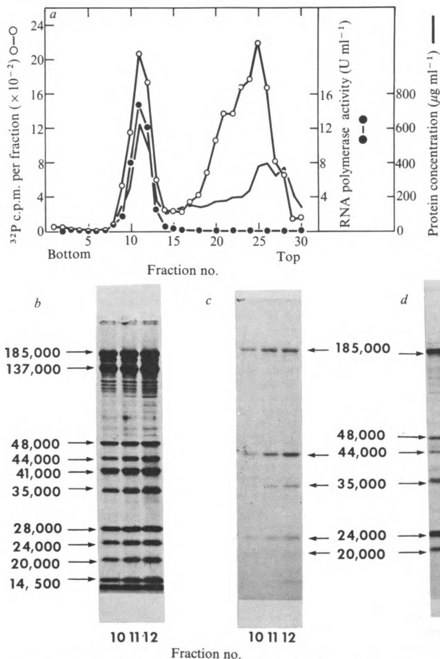
Fig. 1 Phosphorylation of yeast RNA polymerase I. ^{32}\text{P} -labelled RNA polymerase I was isolated from a prototrophic tetraploid strain of Saccharomyces cerevisiae (provided by Dr L. Hartwell) grown in complete medium (YEPD) 15 containing ^{32}\text{P} -phosphate ( 5 \mu\text{Ci ml}^{-1} ). Cells ( 2 \text{ l} ) were collected in the late-log phase of growth ( 30 \text{ g} , wet weight) and spheroplasts were prepared by the two-step procedure of Cabib 16 as described by Wintersberger et al. 20 . RNA polymerase I was extracted in the presence of 1 \text{ mM} ATP and was purified to fraction 3 by a microadaptation of Valenzuela et al. 21 . The ^{32}\text{P} -labelled enzyme fraction was mixed with unlabelled polymerase I (fraction 4) 21 and protein was precipitated by dialysis against a saturated ammonium sulphate solution. The precipitate was collected by centrifugation ( 10,000\text{g} , 20 \text{ min} ) and dissolved in 15\% glycerol, 0.2 \text{ M} KCl, 0.1 \text{ mM} EDTA, 6 \text{ mM} 2-mercaptoethanol, 50 \text{ mM} Tris-HCl, \text{pH} 7.9. The RNA polymerase I was further purified by centrifugation in a 5\text{--}20\% (w/v) sucrose gradient in 0.5 \text{ M} KCl, 15\% glycerol, 0.1 \text{ mM} EDTA, 6 \text{ mM} 2-mercaptoethanol, 50 \text{ mM} Tris-HCl, \text{pH} 7.9 (SW56 rotor, 56,000 \text{ r.p.m.} , 15 \text{ h} , 4^\circ\text{C} ). Fractions were collected by tube puncture. a , Sucrose gradient profile of RNA polymerase I phosphorylated in vivo . RNA polymerase activity and protein concentration of each fraction were determined as before 21 . An aliquot of each gradient fraction was spotted on to a glass fibre filter (GF/C, Whatman). Filters were washed in 10\% trichloroacetic acid (TCA). Contaminating ^{32}\text{P} -labelled nucleic acid was hydrolysed by boiling the filters in 5\% TCA for 15 \text{ min} . The filters were then washed twice more in 5\% TCA, then in ethanol and dried. The ^{32}\text{P} -labelled protein was counted in Omnifluor (New England Nuclear)-toluene scintillant. b , Resolution of polypeptides by sodium dodecyl sulphate (SDS)-acrylamide gel electrophoresis of in vivo ^{32}\text{P} -labelled RNA polymerase. The polypeptides in each sucrose gradient fraction were resolved by 10\% acrylamide slab-gel electrophoresis in the presence of 0.1\% SDS 22 and stained with Coomassie blue. Buffers and solutions were prepared according to Laemmli 22 . The putative subunits of RNA polymerase I and assigned molecular weights are indicated by the arrows. c , Autoradiogram of RNA polymerase polypeptides labelled in vivo with ^{32}\text{P} . The stained gel prepared in ( b ) was dried and the ^{32}\text{P} -polypeptides were located
