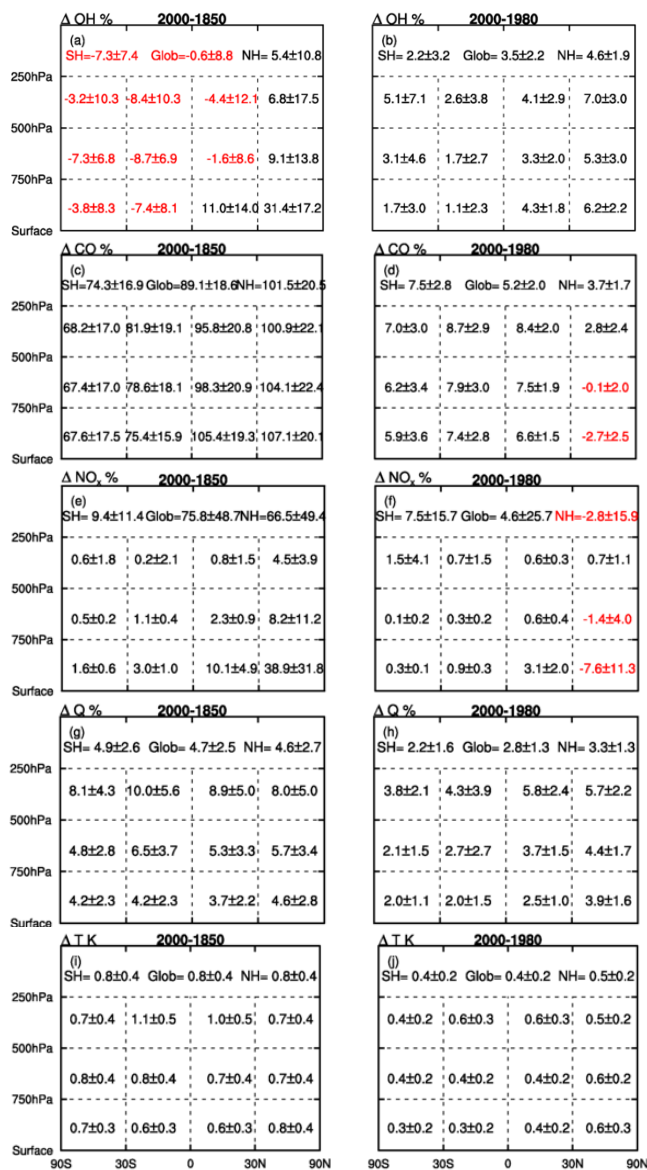
Fig. 3. Multi-model mean percentage change in tropospheric OH, CO and NO x burdens, humidity (Q), and absolute change in temperature for 12 subdomains of the atmosphere as defined by Lawrence et al. (2001) for 2000–1850 (left) and 2000–1980 (right). Decreases are shown in red and increases are in black. Changes in the mean global (Glob), Southern Hemisphere (SH), and Northern Hemisphere (NH) troposphere (surface to 200 hPa) are shown in the top-most row of each plot.
