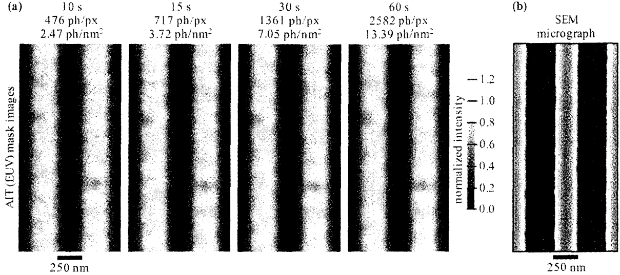
Fig. 1. A comparison of EUV aerial image measurements with an SEM micrograph from the identical region of the mask. (a) Increasing exposure time, and photon energy density, noticeably smoothes the line images, with a clear improvement occurring between 2.47 to 13.39 photons/nm². (b) SEM reveals pattern roughness, but cannot predict the features that produce the static pattern of intensity variation observed in these lines.
