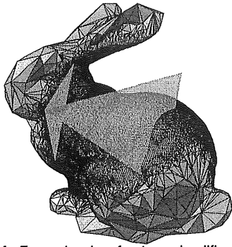
FIGURE 14. Example view-frustum simplification with two sides of a simulated view frustum shown as transparent yellow planes. Rendered 62%, or 43463 out of 69451 faces.
