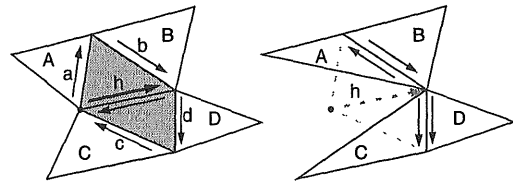
FIGURE 3. Half-edge collapse and vertex split.
