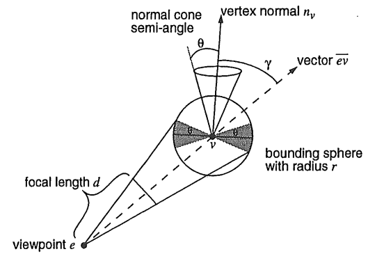
FIGURE 12. Simplification based on screen projection.
