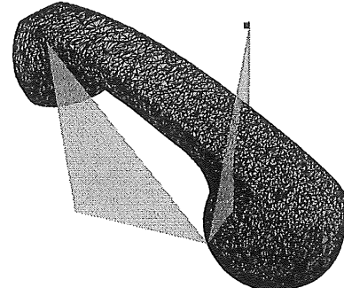
FIGURE 17. Example of screen projection based simplification with projection tolerance \tau = 1/2^{10} . Rendered 19%, or 32755 out of 165963 faces.
