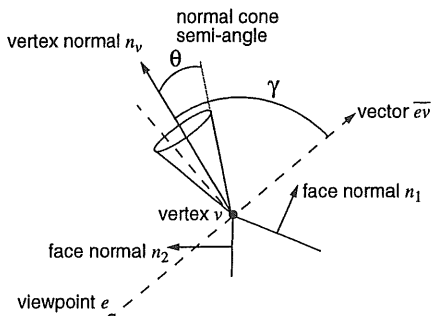
FIGURE 11. Silhouette preservation.
