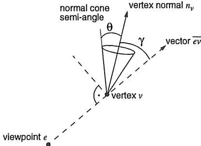
FIGURE 10. Back-face simplification.
