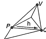
FIGURE 6. Topological ecol constraint. Half-edge h cannot be collapsed because of P and Q being connected to V .
