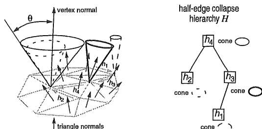
FIGURE 8. Bounding normal cone of a sequence of half-edge collapse operations.
