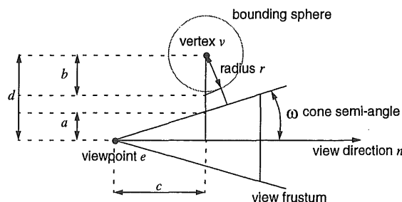
FIGURE 9. Outside view-frustum simplification.
