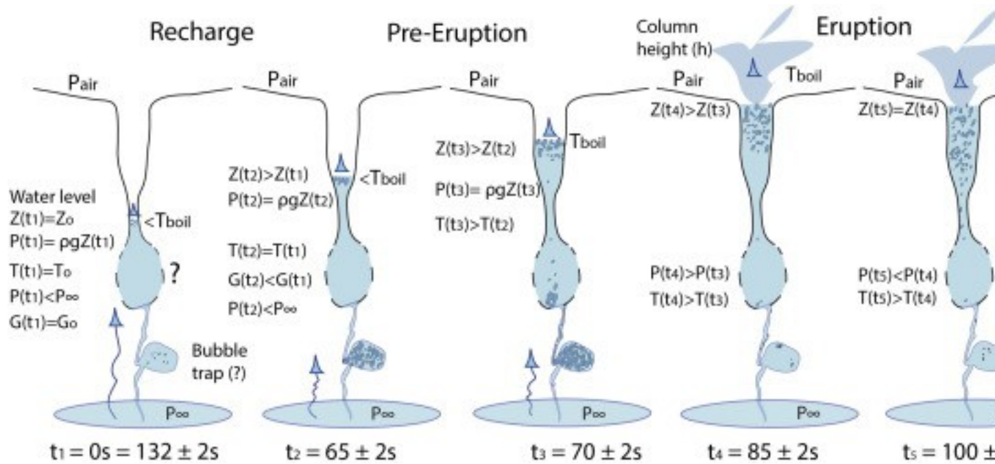
Fig. 14. Conceptual model for El Jefe geyser showing the different stages of the eruption cycle: recharge, pre-eruption, eruption, and relaxation. The model includes a bubble trap or cavity adding steam to the conduit. Blue dots inside the conduit represent bubbles of steam. Blue background represents liquid water. Conditions of pressure ( P ), temperature ( T ), water level ( Z ), and mass flow ( G ) inside the conduit evolve with time. The progression from t_1 to t_7 corresponds to the key stages in the cycle (Fig. 3).
