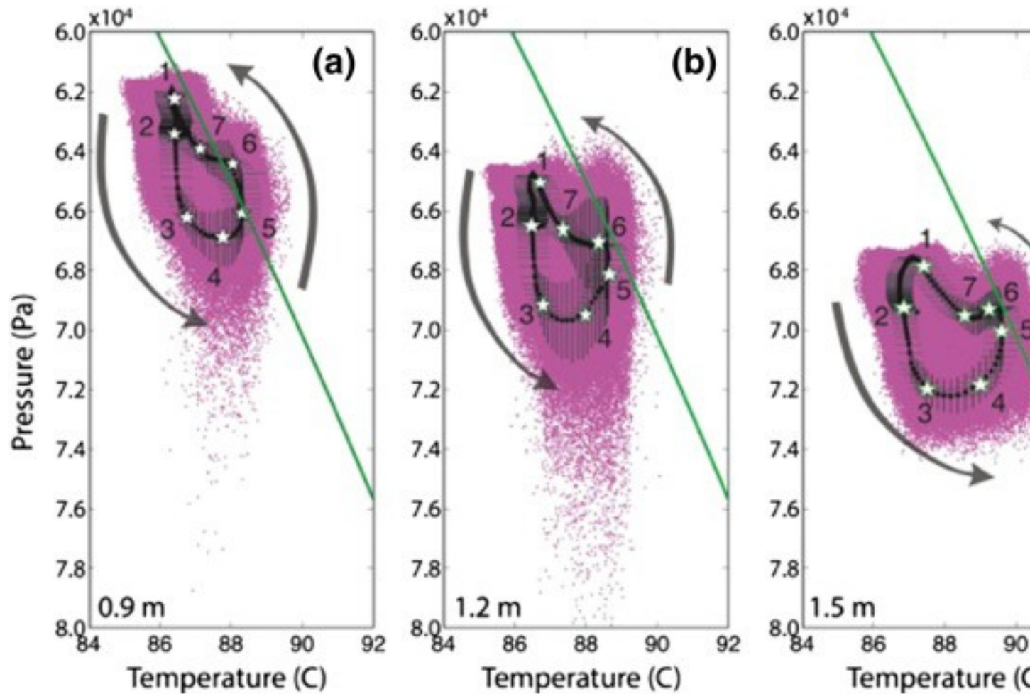
Fig. 8. Water pressure and temperature during the eruption cycles, for ~ 3531 eruptions. Gray arrows show the evolution of pressure and temperature with respect to time (stars 1 through 7: t_1 = 0 s, t_2 = 65 \pm 2 s, t_3 = 70 \pm 2 s, t_4 = 85 \pm 2 s, t_5 = 100 \pm 2 s, t_6 = 105 \pm 2 s, t_7 = 120 \pm 2 s). Black curves show the average and the black bars show the standard deviation of the data. Green lines show the calculated boiling curve for pure water. We define the upper conduit as the part of the conduit without water during quiescent period, from the surface to the air–water interface right before an eruption (~ 0.6 m from surface). Once water at the air–water interface reaches T_{\text{boil}} (Fig. 7c, points 3 to 4) the eruption starts, and boiling water moves rapidly upward through the conduit, reaching the upper sensors in the conduit (Fig. 7ab, points 3 to 4), and the surface (Fig. 5, points 3 to 4). After the ~ 35 second duration of the eruption (Fig. 7ab points 3 to 5), temperature decreases continuously as the water level decreases. The temperature at the top of the water column remains constant at T_{\text{boil}} for ~ 45 s (Fig. 7c, points 3 to 7). Subsequently, the temperature drops ~ 15 °C as cooled erupted
