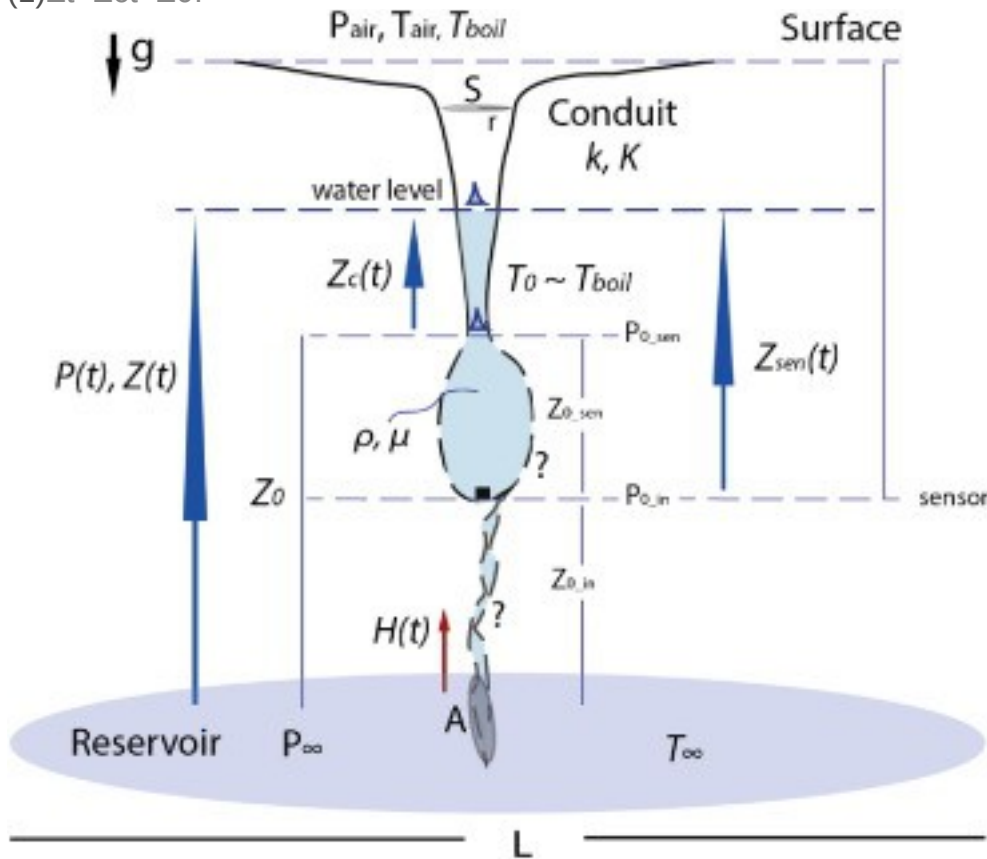
Fig. 10. Schematic illustration of the geyser subsurface showing parameters used in the recharge model.
