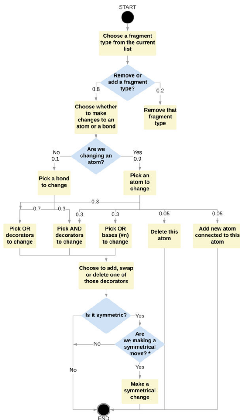
Figure 8. Flowchart to illustrate the decision tree used for SMIRKY move proposals.
