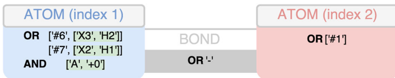
Figure 7. Mapping between ChemicalEnvironment and corresponding SMIRKS pattern.
