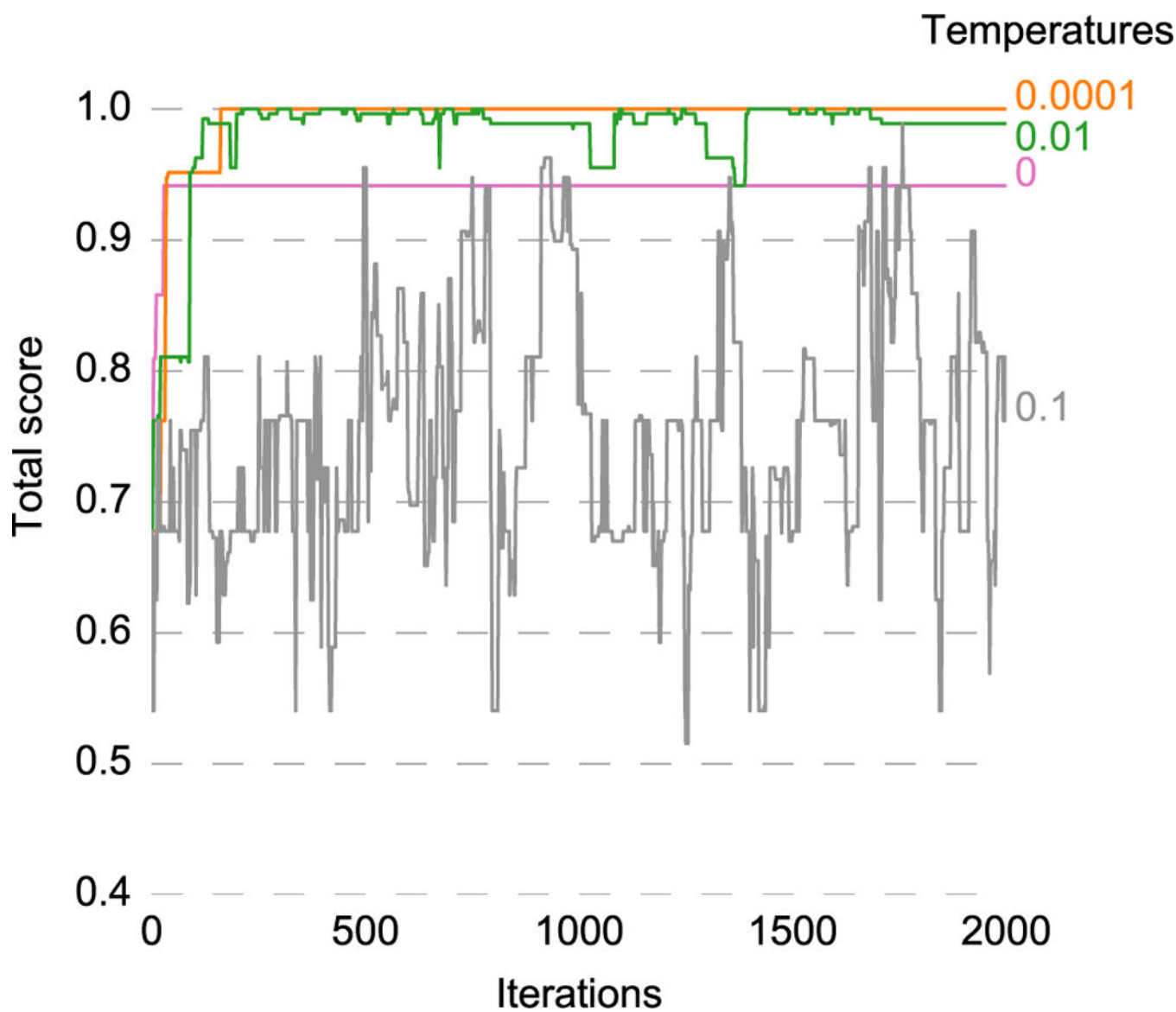
Figure 9. Total score as a function of iteration for SMARTY orig sampling AlkEthOH.
