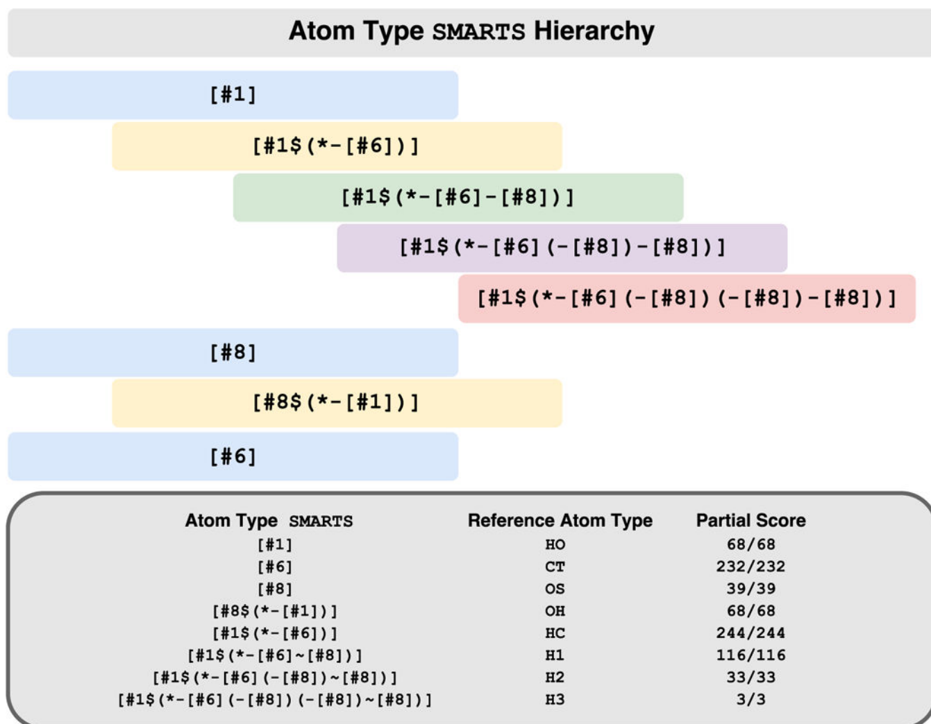
Figure 11. Example of a SMARTY hierarchy and inheritance in AlkEthOH.
