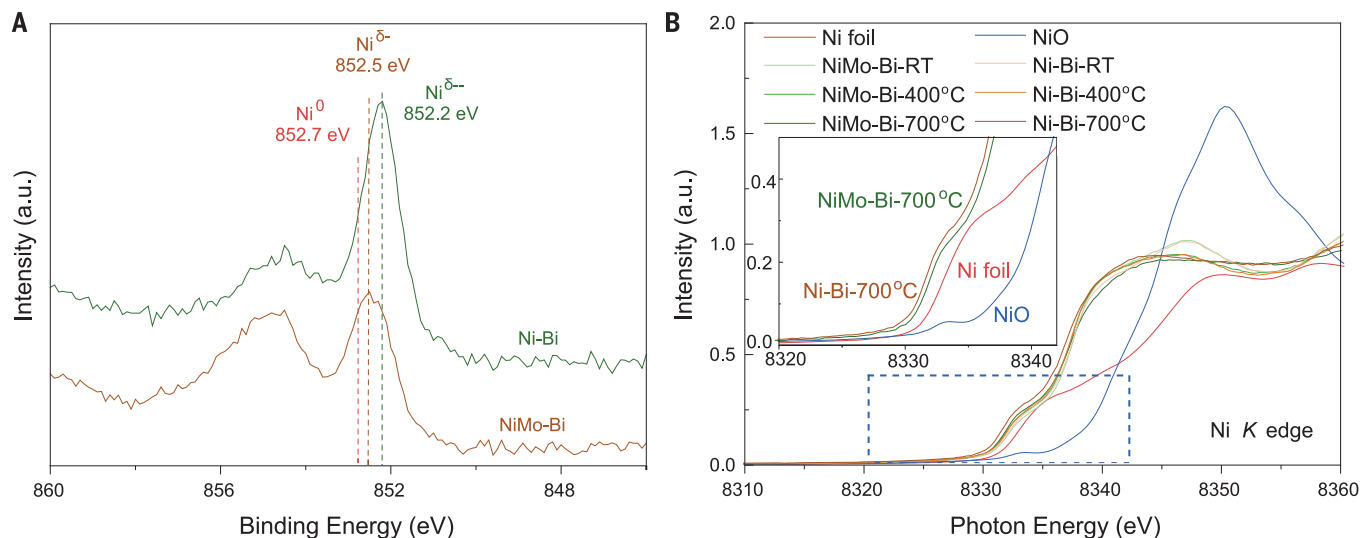
Fig. 3. Statement of Ni species of Ni-Bi and NiMo-Bi liquid alloy catalysts. (A) Nickel 2p x-ray photoelectron spectroscopy (XPS) of Ni-Bi and NiMo-Bi catalysts at room temperature. (B) Ni K-edge x-ray absorption near edge spectroscopy (XANES) spectra of Ni-Bi and NiMo-Bi catalysts at room temperature (RT) and operating temperature.
