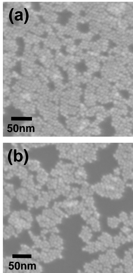
Figure 2. (a) SEM images of PVP coated nanoparticles on silicon wafer (a) before and (b) after UV/ozone treatment for 270 minutes.
