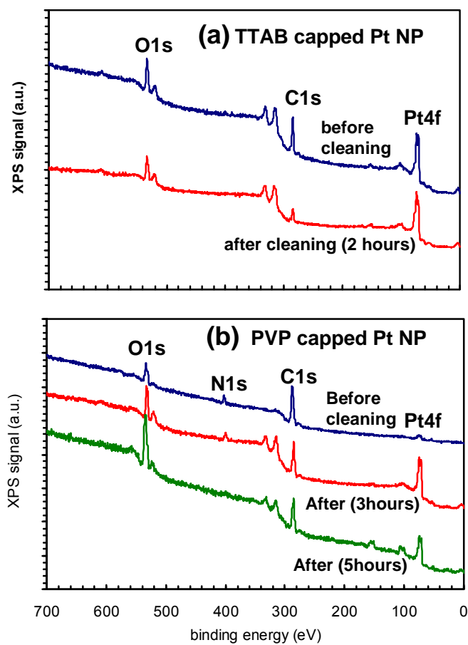
Figure 3. XPS results of (a) TTAB coated, and (b) PVP coated Pt nanocubes deposited on silicon wafer before and after UV-ozone treatment
