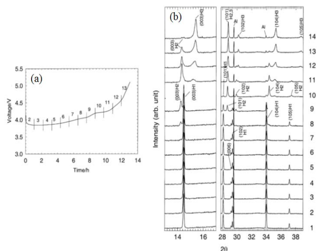
Figure 4 (a) The first charging profile of Li 1-x NiO 2 at C/13 between 3.0 and 5.1 V, (B) In situ XRD patterns of Li 1-x NiO 2 in the (003) to (105) region of the hexagonal structure collected at the designated state of charge. 40 Used with permission from reference 40.
