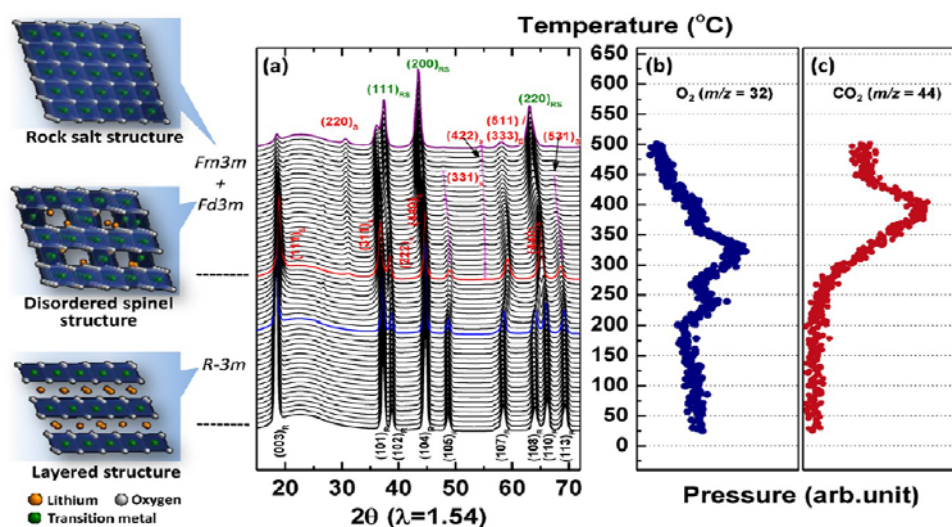
Figure 30 (a) TR-XRD patterns and in-situ mass spectra for (b) \text{O}_2 and (c) \text{CO}_2 when heating \text{Li}_{0.5}\text{Ni}_{0.8}\text{Co}_{0.15}\text{Al}_{0.05}\text{O}_2 up to 500 °C. The left panels show the crystal structure of rhombohedral, spinel, and rock salt. 236 Used with permission from reference 236.
