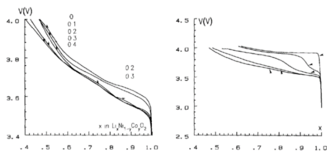
Figure 11 Charge profiles of a \text{Li}/\text{Li}_{1-y}\text{Ni}_y\text{Co}_y\text{O}_2 at various Co contents ( y ). 57 Used with permission from reference 57.
