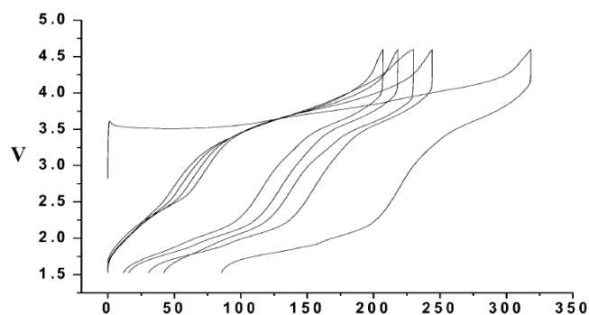
Figure 8 Voltage profiles of a Li half cell containing orthorhombic \text{Li}_2\text{NiO}_2 cycled in the voltage range 1.5 - 4.6 V at a current density of 12.5 mA/g. 12 Used with permission from reference 12.
