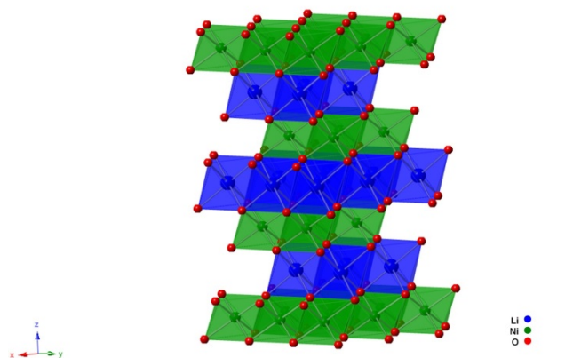
Figure 1 Crystal structure of an idealized layered LiNiO 2 ( R\bar{3}m ), where lithium, nickel and oxygen are represented by blue, green and red spheres, respectively.
