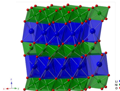
Figure 16 Crystal structure of layered O 2 structure, where lithium, nickel and oxygen are represented by blue, green and red spheres, respectively.
