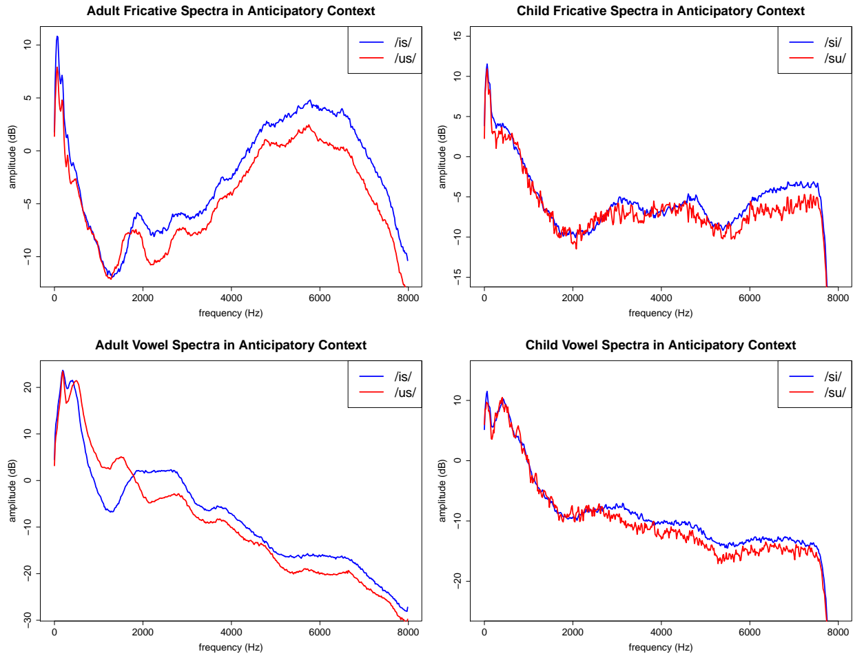
Figure 2: Averaged spectra generated 80% of the way into the fricative (top) and 20 ms into the adjacent vowel (bottom), preceding either a round or non-round vowel, for adult (left) and child (right) data.
