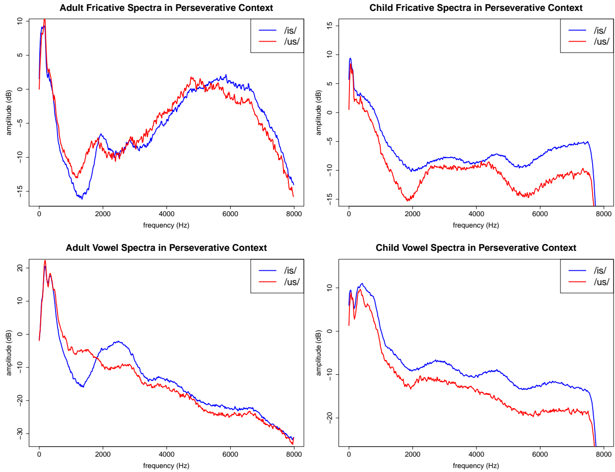
Figure 3: Averaged spectra generated 20% of the way into the fricative (top) and 20 ms into the adjacent vowel (bottom), following either a round or non-round vowel, for adult (left) and child (right) data.
