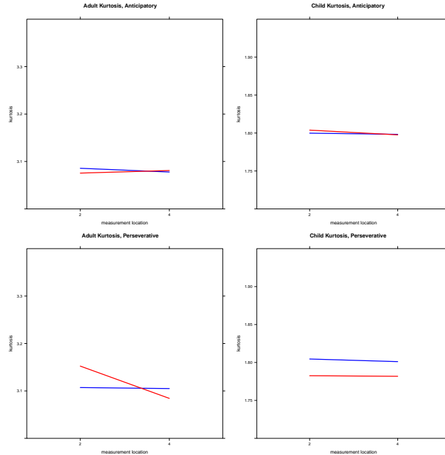
Figure 6: Kurtosis measurements taken at the 20% and 80% duration time points in the fricative, averaged across all tokens. Higher values (red lines: round vowel context) indicate a more peaked distribution, which is correlated with lip rounding. Left: adult data. Right: child data. Top: anticipatory coarticulation. Bottom: perseverative coarticulation.
