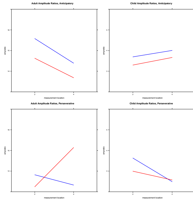
Figure 5: Amplitude ratio measurements taken at the 20% and 80% duration time points in the fricative, averaged across all tokens. Higher values (blue lines: non-round vowel context) indicate a more palatal tongue posture. Left: adult data. Right: child data. Top: anticipatory coarticulation. Bottom: perseverative coarticulation.
