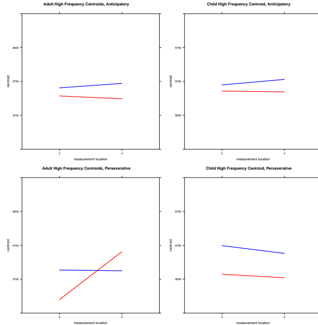
Figure 4: High frequency centroid measurements taken at the 20% and 80% duration time points in the fricative, averaged across all tokens. Lower values (red lines: round vowel context) indicate a longer front cavity, caused by lip rounding and/or retracted place of articulation. Left: adult data. Right: child data. Top: anticipatory coarticulation. Bottom: perseverative coarticulation.
