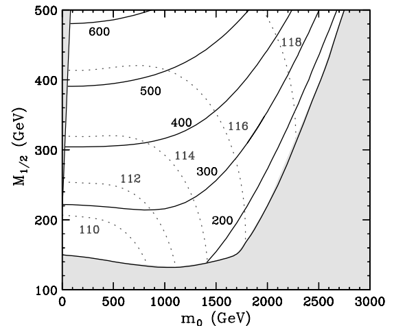
FIG. 3. Contours of \mu (solid) and m_h (dotted) in GeV for input parameters as in Fig. 1.
