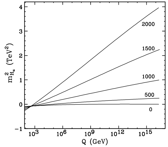
FIG. 2. The RG evolution of m_{H_u}^2 for fixed M_{1/2} = 200 GeV, A_0 = 0 , \tan\beta = 10 , m_t = 175 GeV, and several values of m_0 (shown, in GeV). The RG behavior of m_{H_u}^2 exhibits a focus point near the weak scale, where m_{H_u}^2 takes its weak scale value \sim -(300 \text{ GeV})^2 , irrespective of m_0 .
