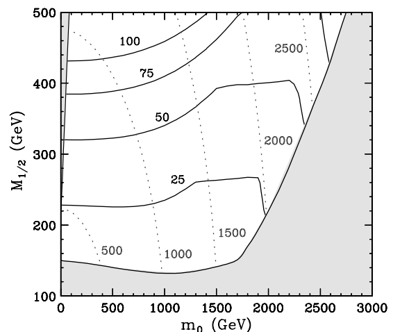
FIG. 1. Contours of constant fine tuning c (solid) and m_{\tilde{u}_L} in GeV (dotted) in the (m_0, M_{1/2}) plane for \tan\beta = 10 , A_0 = 0 , and \mu > 0 . The shaded regions are excluded by the requirement that the lightest supersymmetric particle be neutral (top left) and by the chargino mass limit of 90 GeV (bottom and right).
