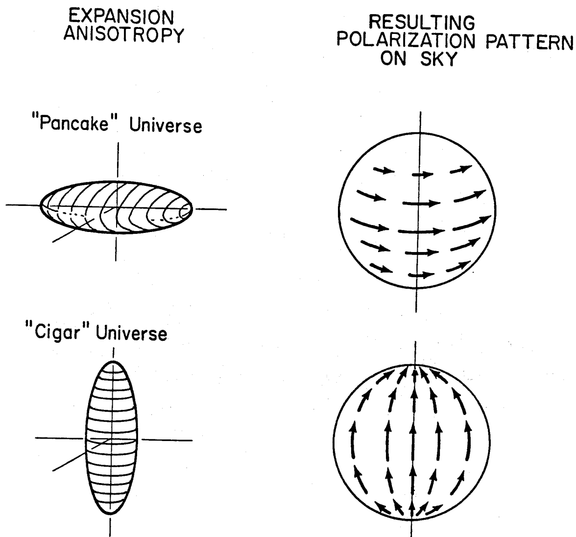
Figure 1. Expansion anisotropy and resulting polarization pattern on the sky for two simple axisymmetric anisotropic models.
