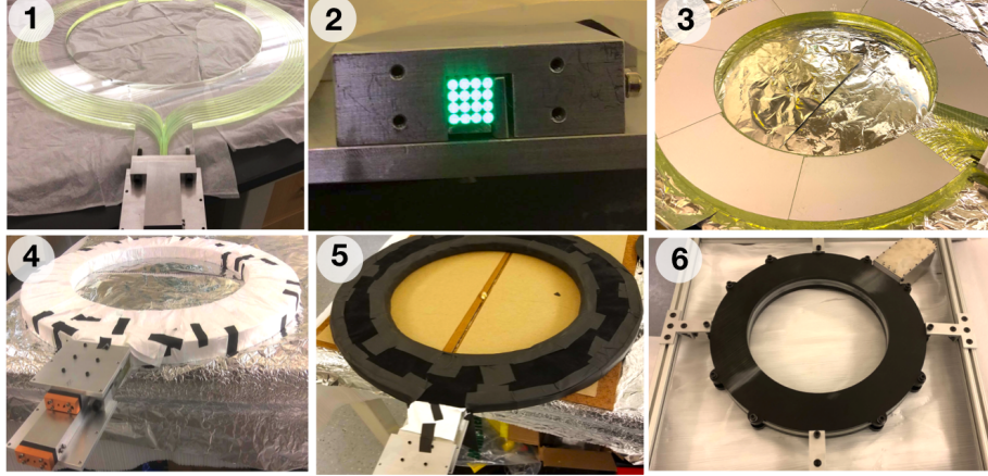
Figure 8: 1) Grooved acrylic with all fibers glued into the groove using RTV-615 silicone glue. 2) The 4\times 4 matrix of the fibers coming out of the clamp. 3) {}^6\text{LiF-Zns(Ag)} scintillator attached to the acrylic via optical glue. 4) Tyvek is wrapped around the detector for diffusive reflection of light 5) A final layer of thick black opaque paper wraps the detector to make it light tight. 6) Fully assembled Backing Detector along with its support structure.
