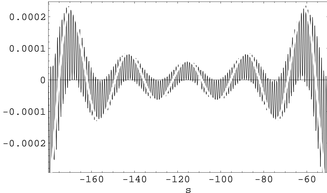
Figure 1: Plots of the partition function W(s, \{\overline{21}\}) ( black curve ) and its first Sylvester wave W_1(s, \{\overline{21}\}) ( white curve ) showing that the polynomial part provides an important information about the partition function behavior.
