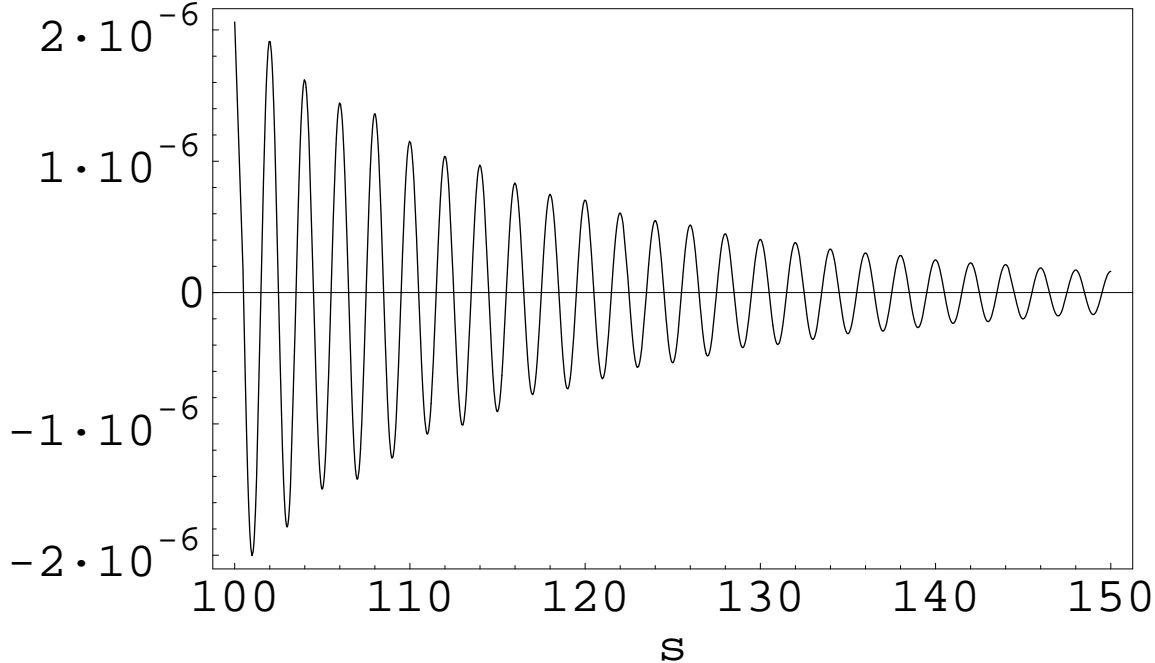
Figure 2: Plot of the normalized difference [W(s, \{\overline{21}\})/W_1(s, \{\overline{21}\}) - 1] showing that the polynomial part W_1(s, \{\overline{21}\}) at large values of the argument s gives a very accurate approximation to the partition function W(s, \{\overline{21}\}) .
