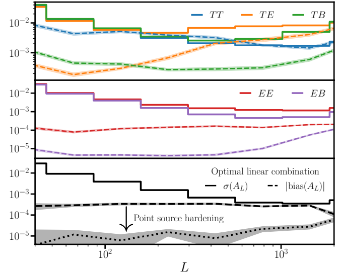
Figure 4. Top two panels: Solid lines show the 1\sigma error of the lensing amplitude ( A_L \equiv C_L^{\kappa\kappa, \text{measured}} / C_L^{\kappa\kappa, \text{true}} ) for each single-pair minimum variance (MV) estimator. Colors denote pairs of temperature and polarization. Dashed lines show the simulated (absolute) biases to the MV estimators due to radio point sources, with the shaded regions denoting the 1\sigma scatter of the mean. Bottom: Error (solid) and bias (dashed) to the lensing amplitude for the optimal linear combination of MV single-pair estimators. The dotted curve shows the bias for an optimal combination of point source hardened estimators. See sections V and VI for details regarding the experimental configuration and simulations respectively.
