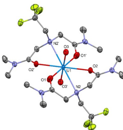
Figure 6. X-ray crystal structure of \text{UO}_2\text{L}_2(\text{ClO}_4)_2 with 50% probability ellipsoids. Perchlorate ions and hydrogen atoms are omitted for clarity.
