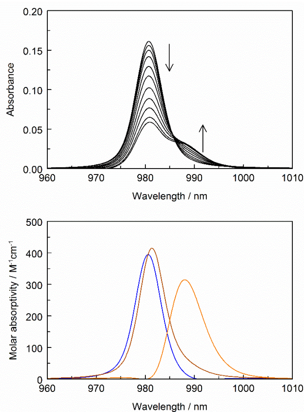
Figure 4 Spectrophotometric titrations of \text{NpO}_2^+ complexation with \text{CF}_3\text{ABDMA} (upper) and calculated molar absorptivity of \text{Np(V)} species (lower): \text{NpO}_2^+ (blue), \text{NpO}_2\text{NO}_3 (brown), \text{NpO}_2\text{L}^+ (rose). Detailed titration conditions are in Table S3 of Supporting Information.
