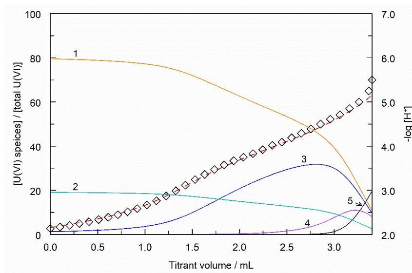
Figure 2. Potentiometric titration of U(VI)/L complexation at 25 °C and I = 1.0 M NaNO 3 . Symbols: (•) experimental -log[H + ]; (dashed line) fitted -log[H + ]; (solid lines) U(VI) speciation, 1 – free UO 2 2+ , 2 - UO 2 (NO 3 ) + , 3 - UO 2 L 2+ , 4 - (UO 2 ) 2 (OH) 2 2+ , 5 - (UO 2 ) 3 (OH) 5 + . This is titration #3, detailed titration conditions of which are shown in Table S2 of Supporting Information.
