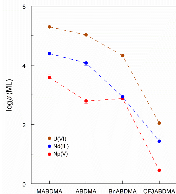
Figure 5. Thermodynamic trends in the complexation of amine-bridged diacetamide ligands with \text{UO}_2^{2+} , \text{Nd}^{3+} , and \text{NpO}_2^+ . Data are for t = 25\text{ }^\circ\text{C} and I = 1.0\text{ M NaNO}_3
