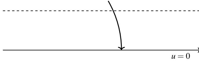
Figure 2.3 Sufficiently near the boundary geodesics behave as in the upper half plane.
